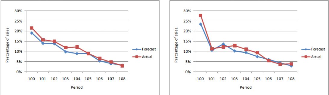
Figure 3: Weekly aggregate forecast versus actual sales for Belgium (left) and Ireland (right).
