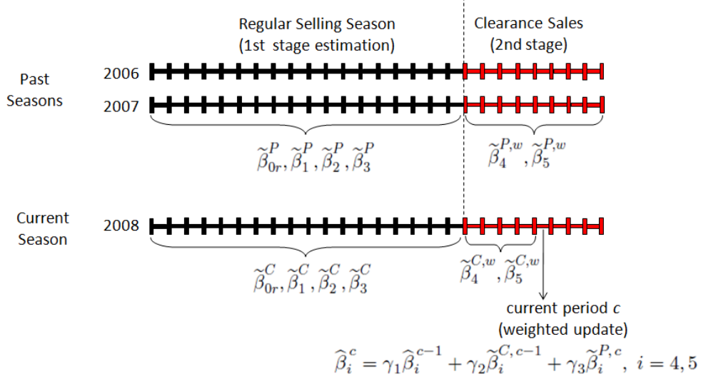
Figure 2: Two-stage estimation procedure using past ( P ) and current ( C ) season data. The current period is denoted by w = c .
