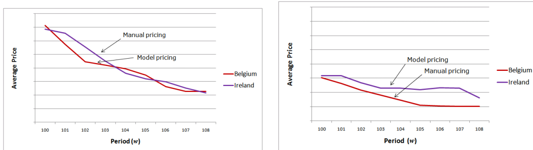
Figure 5: Average price ( P^w ) across periods for groups 1-12 (left) and groups 13-20 (right) in Belgium and Ireland.
