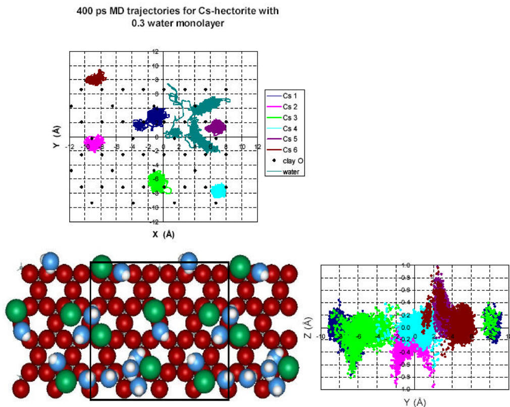
Figure 18. MD trajectories.
