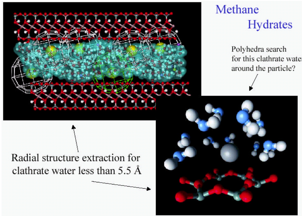
Figure 15. Methane hydrates.
