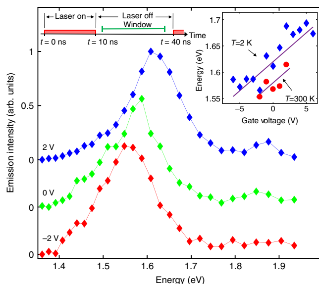
Fig. 5 Control of energy by voltage. Spectra at a delay after the laser excitation pulse in the time window shown above at gate voltages V_g = -2 , 0, and 2 V at T = 300 K. Gate voltage dependence of IX energies at T = 300 and 2 K is shown in the inset. The excitation laser has a pulse duration of 10 ns and a period of 40 ns
