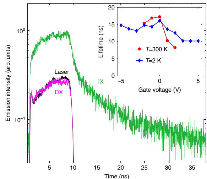
Fig. 3 Emission kinetics. Emission kinetics at energies of 1.46–1.65 eV corresponding to the IX spectral range (green), 1.89 eV corresponding to the DX spectral range (magenta), and 3.07 eV corresponding to the excitation laser (black) at T = 300 K and V_g = 0 . IX lifetimes are shown in the inset as a function of gate voltage V_g for T = 2 and 300 K, see text. The laser excitation has a pulse duration of 10 ns and a period of 40 ns
