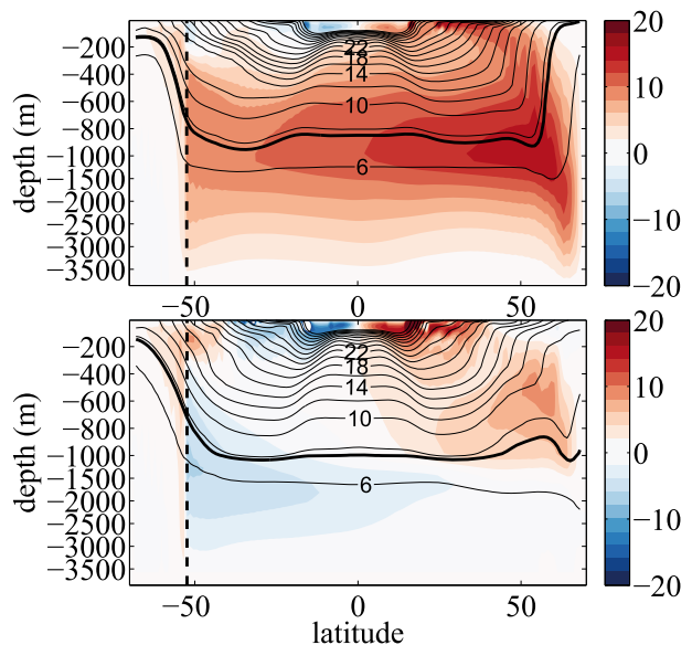
FIG. 6. Residual overturning streamfunction in Sverdrups (color contours, interval 2 Sv) and b^\# \times 10^3 \text{ m s}^{-2} , the buoyancy of the surface whose average depth is z (black contours) in the (top) narrow basin and (bottom) wide basin. Sinking is in the narrow basin. In both plots, the reentrant channel region (left of the thick black dotted line) shows the total streamfunction over all longitudes. The thick black contour denotes the isopycnal b_m = 0.0076 \text{ m s}^{-2} , which bounds the upper branch of the ROC.
