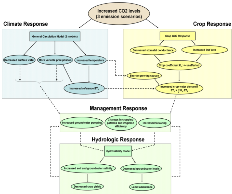
Figure 2. Overview of the methodology for assessing potential climate change impacts on irrigated agriculture.
