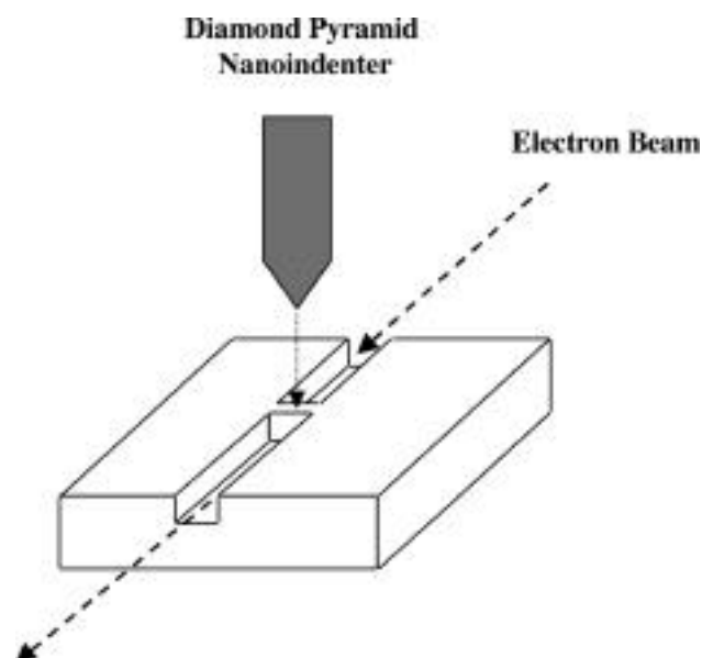
Figure 2.3.1 Schematic of the focused ion beam (FIB) sample geometry. A trench is milled out of the sample leaving behind a window thin enough to be electron transparent. The diamond indenter can approach the thin window in a direction normal to the electron beam, as shown.
