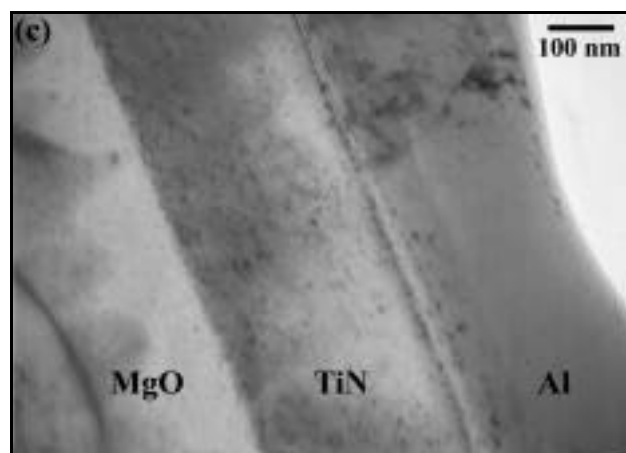
Figure 2.3.7 (a) (b) and (c) TEM images of a FIB-prepared Al/TiN/MgO sample before the Al protective layer was removed.
