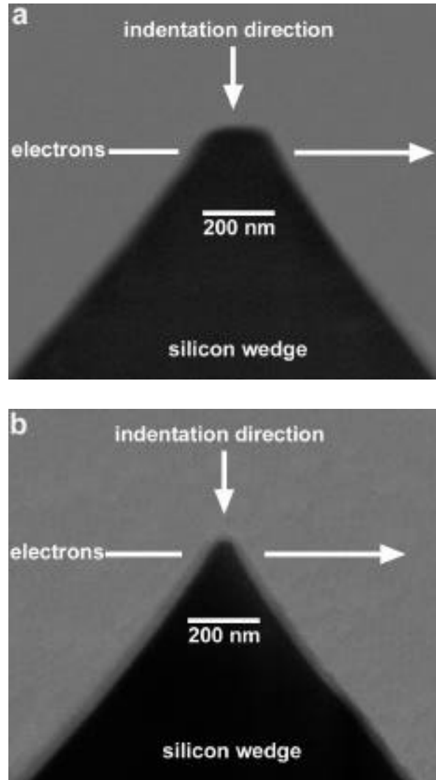
Figure 3.2.1 Scanning electron micrographs of the lithographically-prepared silicon wedge samples in cross-section. (a) , the blunt geometry, with a plateau of \sim 150 nm, and (b) the sharp geometry, with a plateau of \sim 20 nm. The cross sections were prepared with a focused ion beam after a layer of Pt was deposited for protection.
