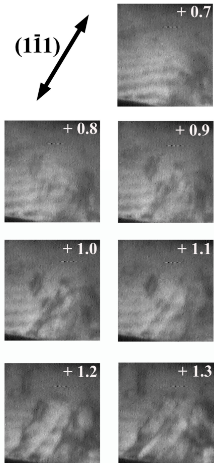
Figure 3.3.4 Series of dark field transmission electron micrographs showing the appearance and evolution of prismatic dislocation loops in a previously undeformed part of the Al grain during an in situ nanoindentation. The numbers in the micrographs are the time in seconds from the start of the indentation.
