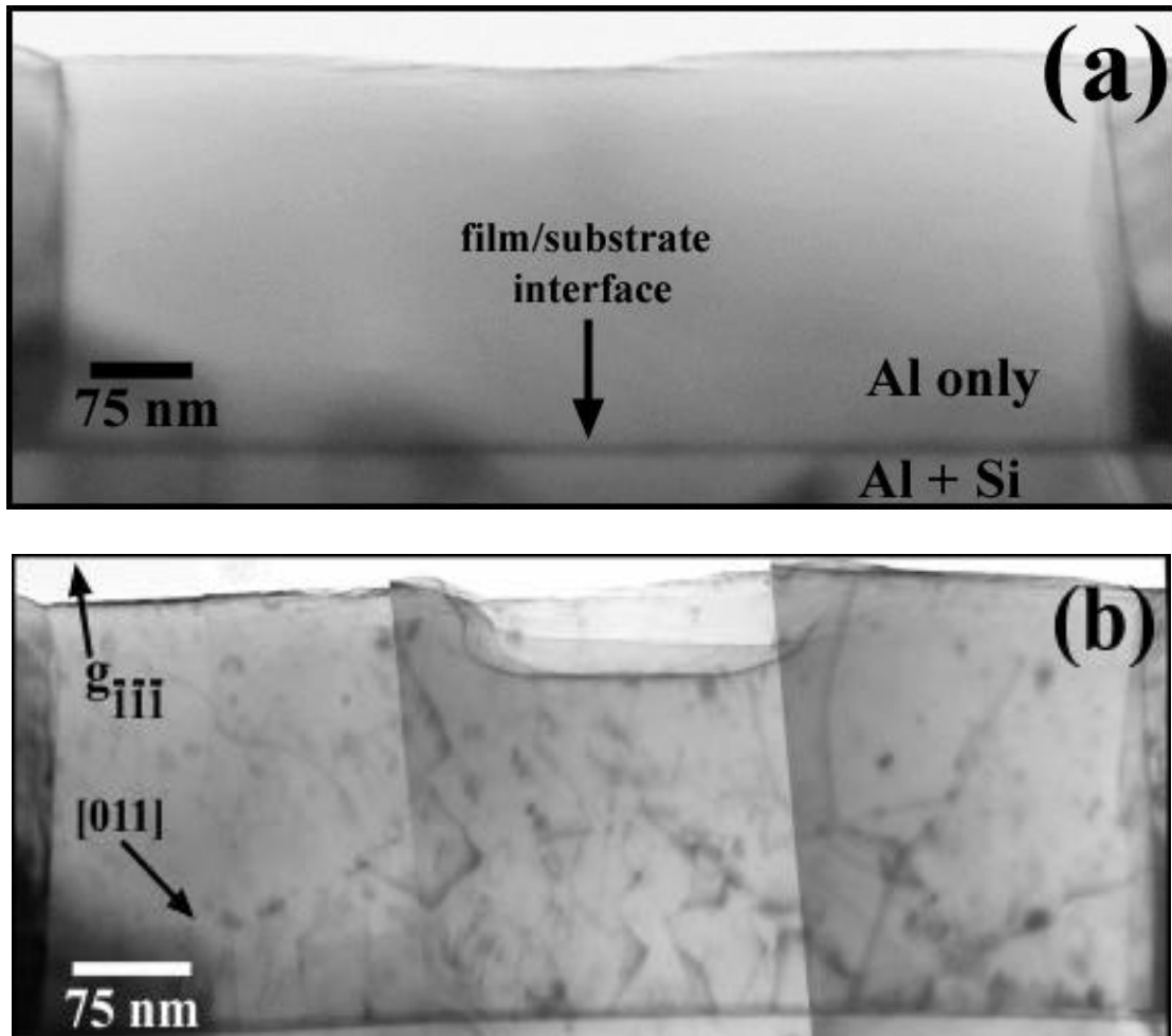
Figure 3.3.9 (a) shows the as-deposited condition of an Al grain deposited onto a Si wedge substrate. The interface of the Al grain and Si substrate can be seen at the bottom of the image. (b) Shows the same Al grain in the same diffraction condition after indentation (3 images are pasted together here in order to span the entire grain at high magnification). The indentation crater can be seen at the top of the image, as can the numerous dislocations introduced in order to accommodate the induced deformation. Quite noticeably, the dislocations pile up at the film/substrate interface.
