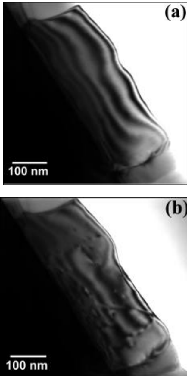
Figure 3.3.10 (a) Bright field TEM image showing the as-deposited condition of an Al grain deposited onto a Si wedge substrate (b) Shows the same Al grain in the same diffraction condition after indentation. In this case, the dislocations do not extend all the way to the lateral grain boundaries.
