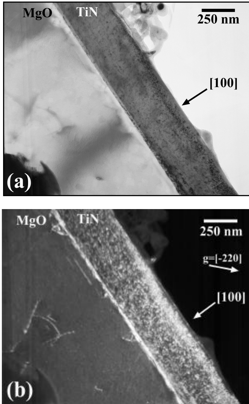
Figure 3.4.10 (a) Bright field and (b) dark field TEM micrographs of the epitaxial TiN/MgO (100) sample prior to indentation. Both images are taken in the g = (-220) condition. The arrows showing the [100] direction in both images also point to the location of the indentation shown in figure 3.4.11.
