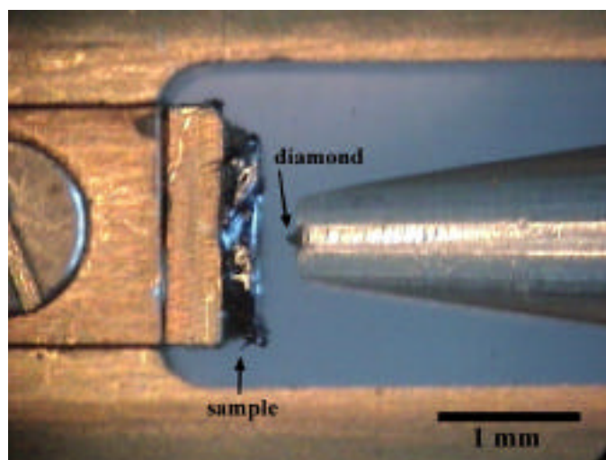
Figure 2.1.6 Image of sample loaded into the in situ nanoindentation stage. The diamond indenter can be seen mounted on the end of an Al rod. The details of the sample cannot be seen at this low magnification.
