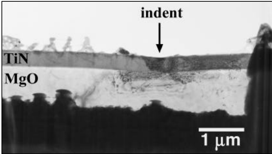
Figure 3.4.12 Lower magnification image of the same indentation shown in figure 3.4.11. The bending of the TiN film can be seen more clearly with reference to the film position farther away from the indentation. Notice the dislocations emanating from the indentation axis in the MgO.
