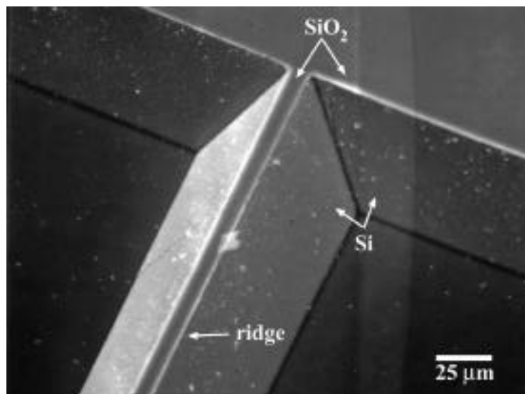
Figure 2.2.3 SEM image of silicon wedge structure after being etched in a KOH bath. The SiO 2 masking layer is still attached to the top of the structure. This corresponds to step 5 of the silicon wedge microfabrication process as described in Figure 2.2.1.
