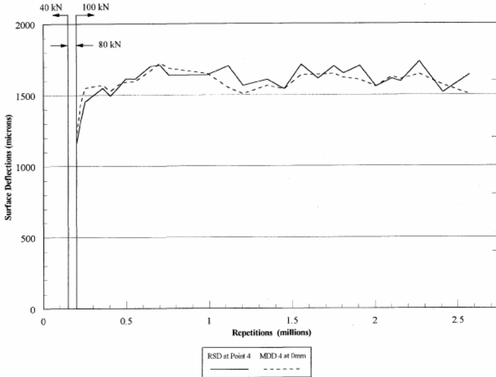
Figure 3.21 Comparison of Elastic Deflections Determined by the RSD and by the MDD at Point 4 with a 100 kN Load
