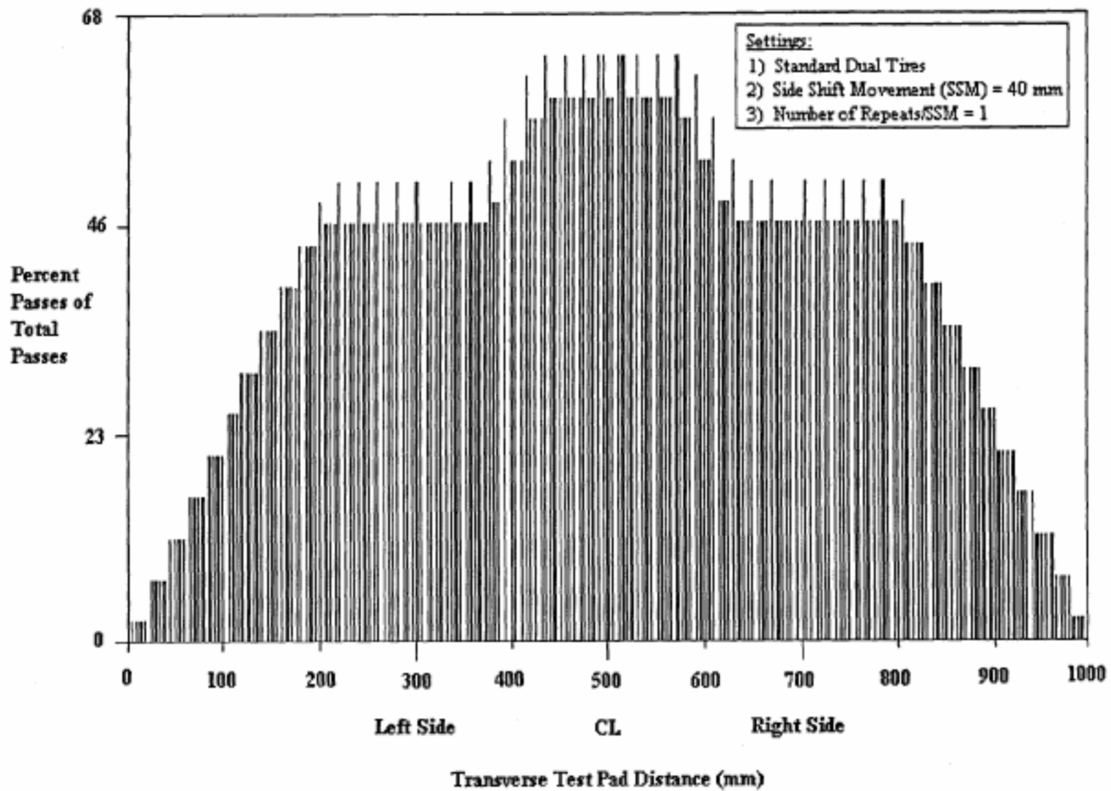
Figure 2.4 Transverse Load Distribution for HVS
