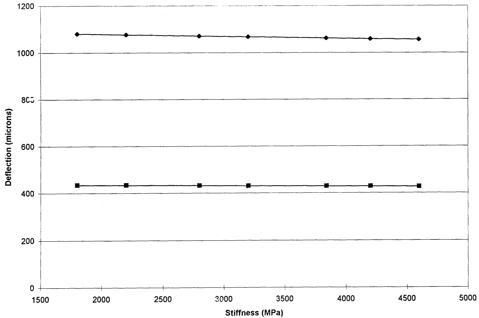
Figure C1 Effect of Stiffness of the Top Lift of AC on Surface Deflection
