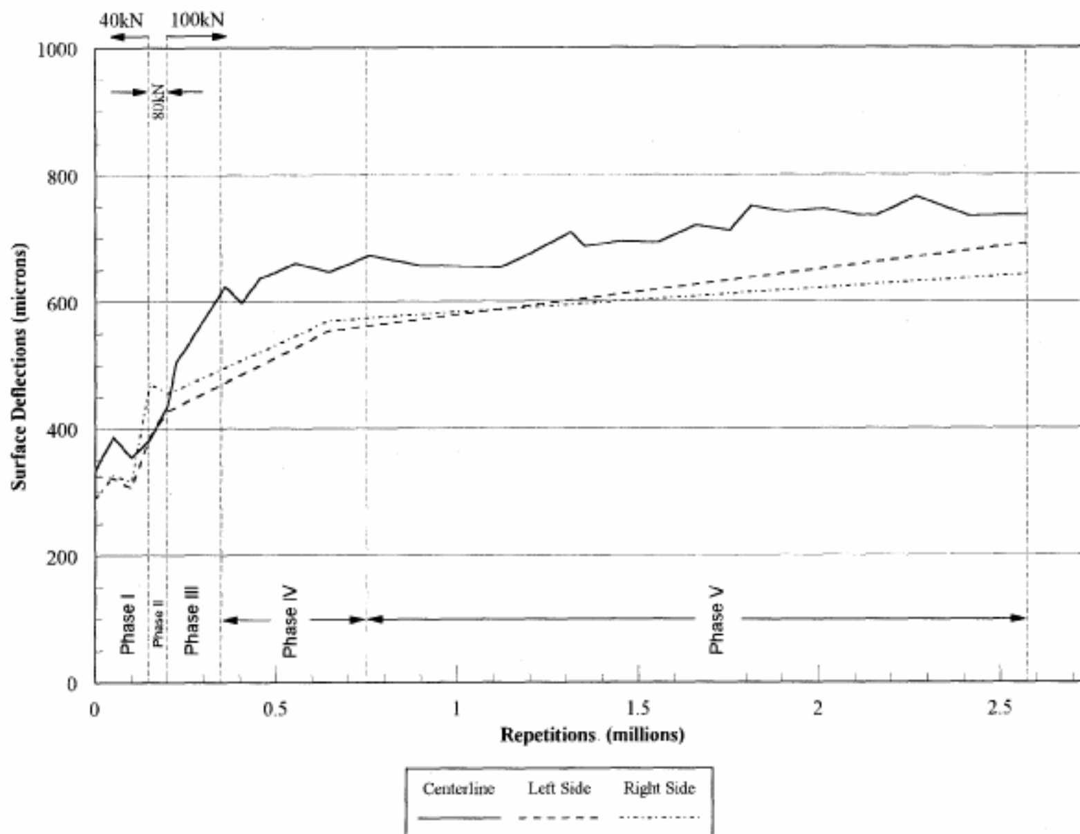
Figure 3.18 Average Road Surface Deflections, 40 kN Test Load
