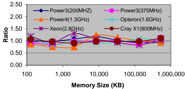
Fig. 6. The performance ratio for FFT using one random access stream
