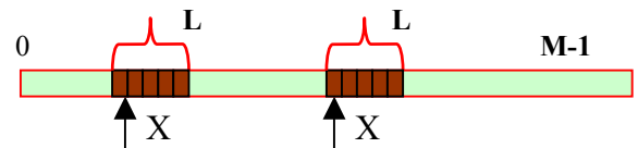
Fig. 3. The random memory access pattern of Apex-MAP.
