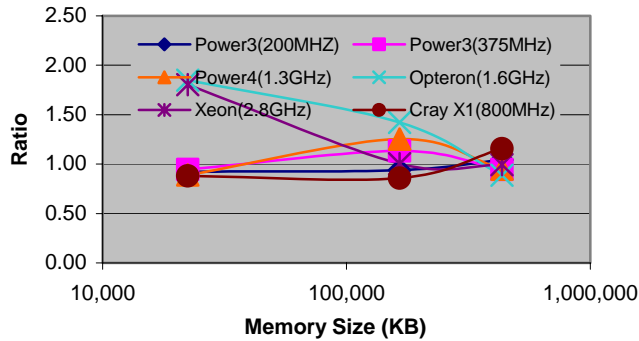
Fig. 10. The performance ratio for CG using one random access stream
