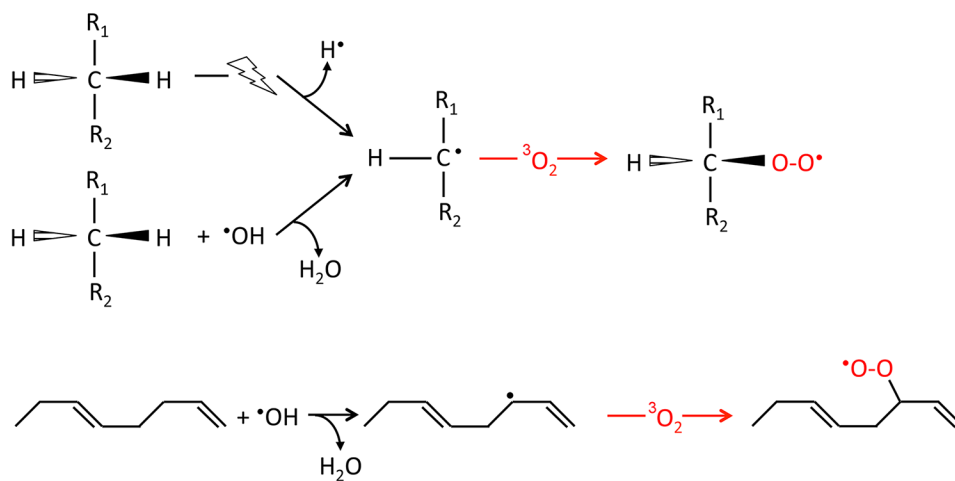
Figure 1. Basic scheme of the direct or indirect ( \cdot OH ) formation of carbon-centered radicals by hydrogen atom abstraction from an aliphatic (top) or unsaturated carbon chain (bottom) and ensuing generation of peroxy radicals by reaction with molecular oxygen in the fundamental (triplet) state.
