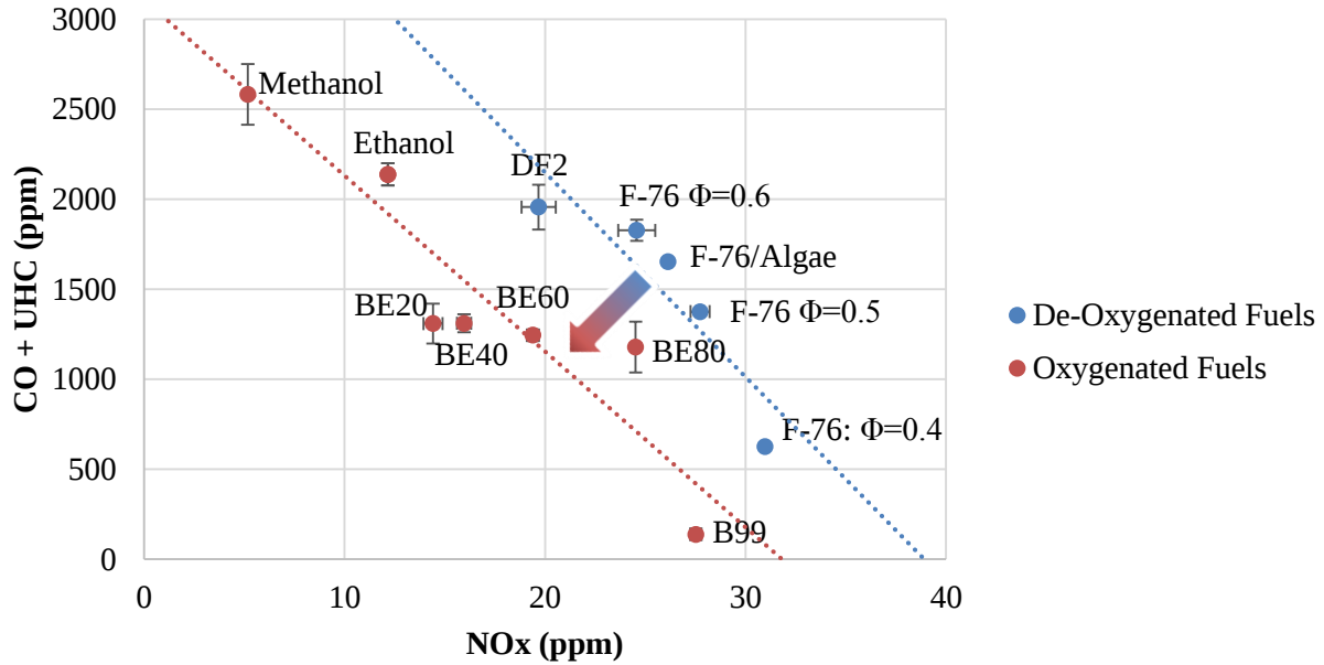
Figure 52: \text{NO}_x vs. CO & UHC for All Fuels
