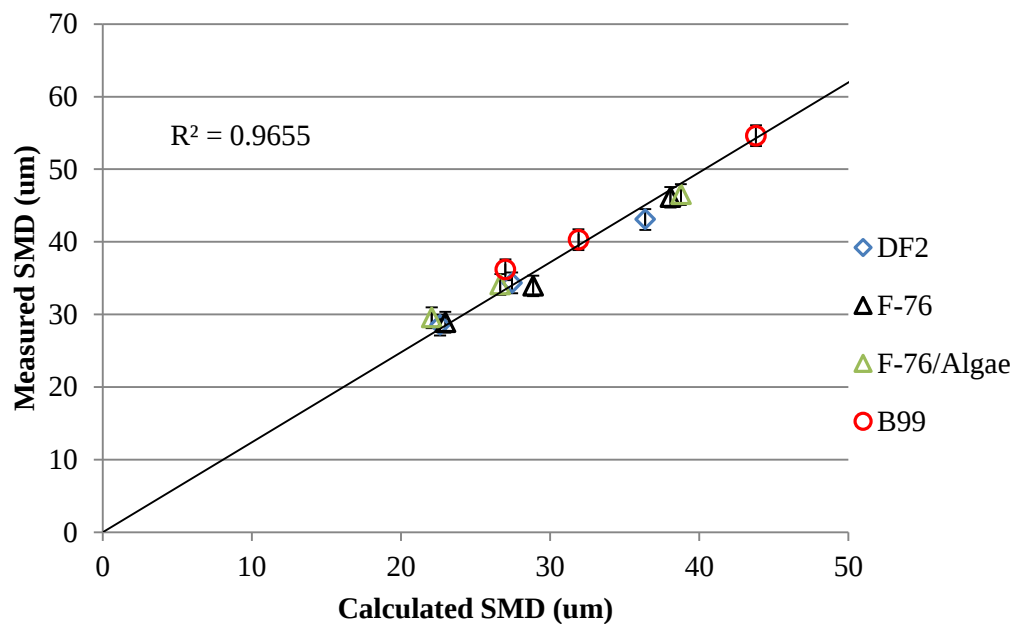
Figure 39: Measured vs Calculated SMD for Four Fuels
