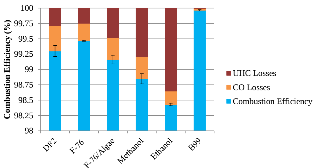
Figure 30: Combustion Efficiencies and Associated Losses
