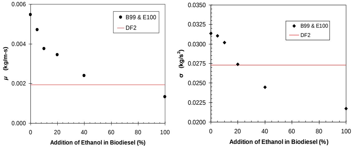
Figure 11: Viscosity [L] and Surface Tension [R] for 95/05, 90/10, 80/20, and 60/40 Percent Blends of B99 and Ethanol (Bolszo & McDonell 2008)
