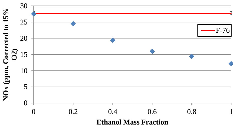
Figure 50: NO x Emissions for B99-Ethanol Blends
