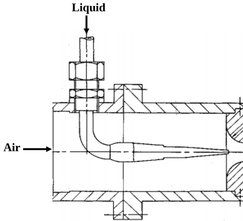
Figure 2: Plain-jet air-blast atomizer (Lefebvre et al., 1977)
