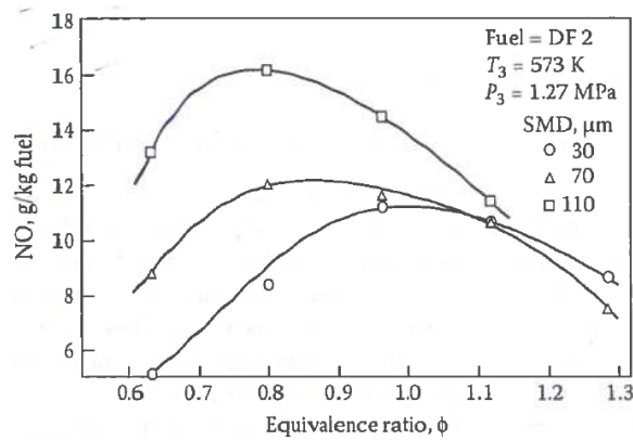
Figure 4: Influence of fuel atomization on NO emissions (Rink, Lefebvre 1989)
