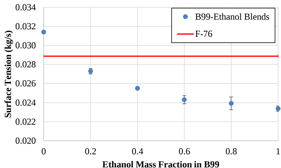
Figure 44: Surface Tension for various B99-Ethanol Blending Ratios
