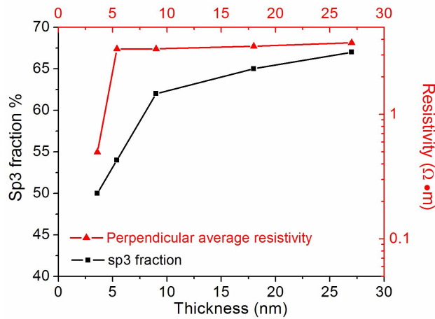
Figure 5. 5 Average resistivity and \text{sp}^3 fraction for different thickness samples.
