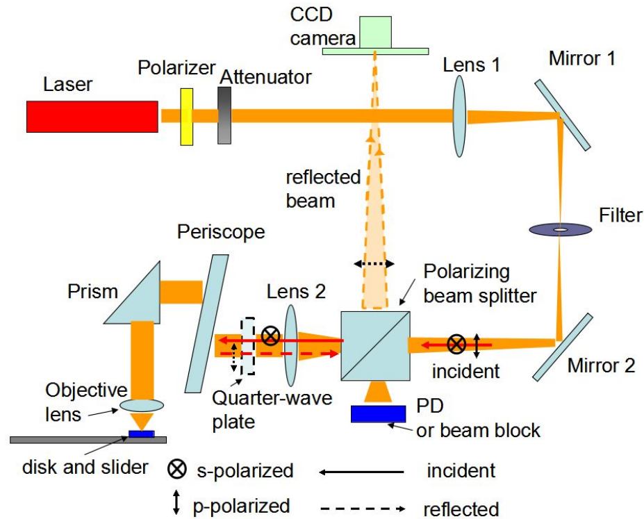
Figure 3. 4 Optical beam path of the Cal stage
