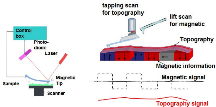
Figure 2. 3 Schematic plot of MFM
