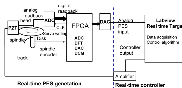
Figure 8. 16 Configuration of the FPGA based servo system for HDDs.
