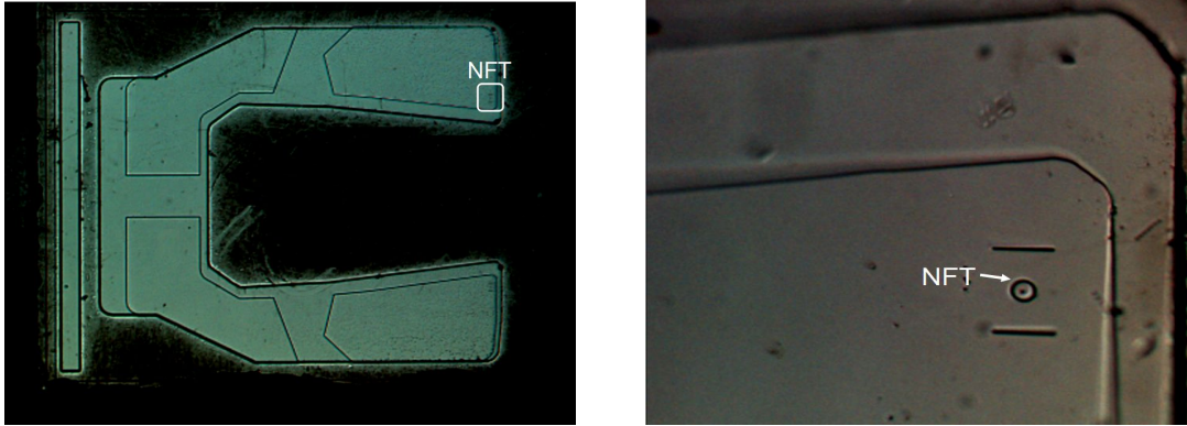
Figure 3. 7 Homemade slider with an NFT; (left) Optical microscope image of a homemade air bearing surface; (right) zoomed NFT structure and alignment structure on the trailing edge
