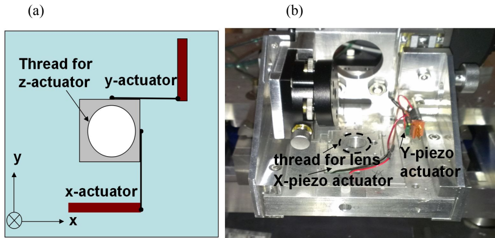
Figure 8. 6 Flexure to assist laser beam alignment to the NFT (a) schematic design of the flexure; (b) photo of the flexure
