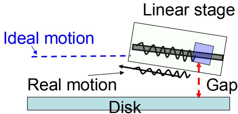
Figure 3. 19 Schematic plot of the relative motion of the linear stage relatively to the disk surface
