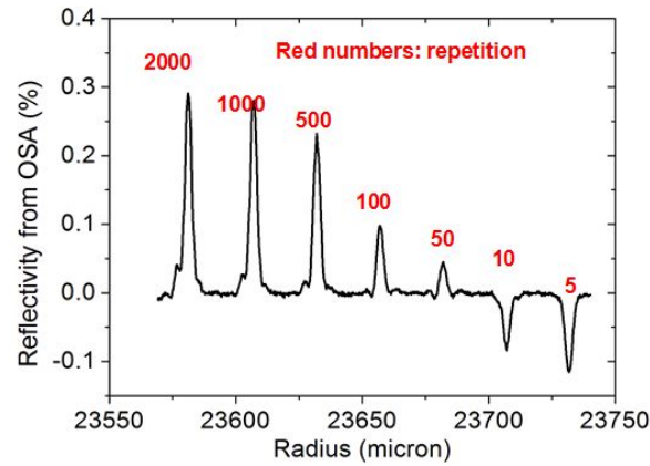
Figure 5. 12 Surface reflectivity profiles of the tracks after exposure at various repetitions at a power density of 29.0 mW/μm².
