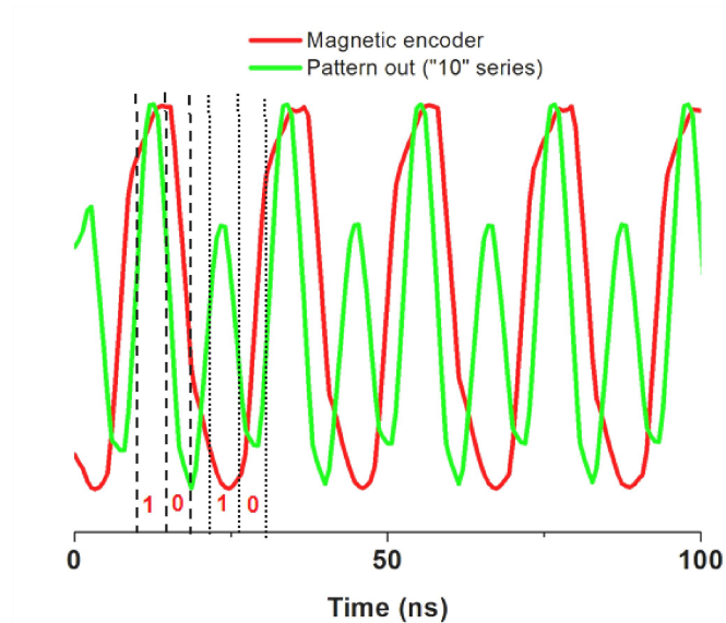
Figure 8. 30 Measured pattern output and magnetic encoder by a high speed DAQ.
