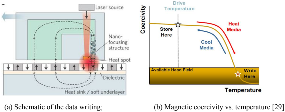
Figure 1. 12 Concept of HAMR.
