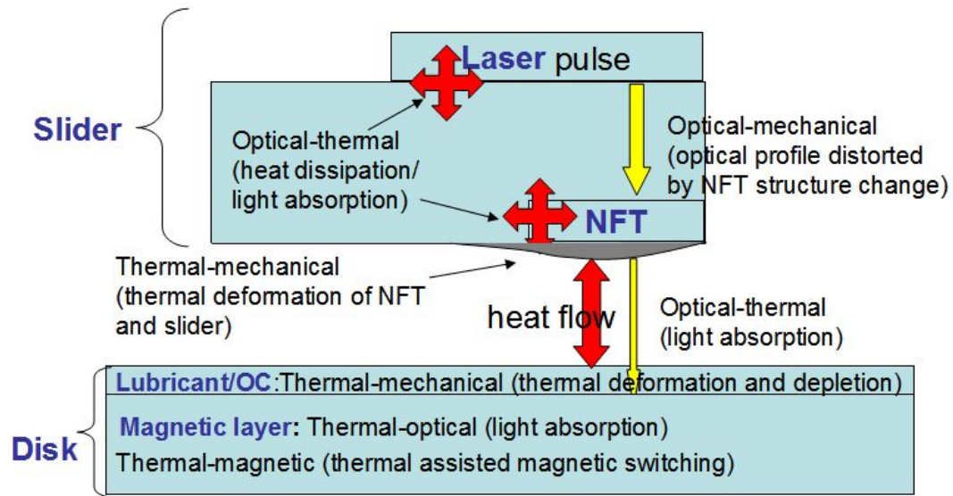
Figure 1. 17 Multiple physical couplings among light, heat, mechanical deformation and magnetism inside the HDI of HAMR systems
