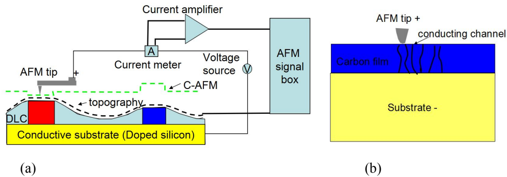
Figure 5. 2 (a) Schematic drawing of C-AFM system for conductivity measurement; (b) Conducting channels in DLC film
