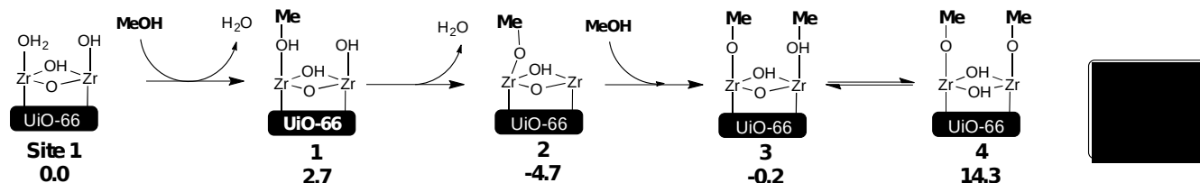
Figure 3. Relative free energies (298.15 K, liquid methanol containing 1% H 2 O) of possible products from methanol substitution.
