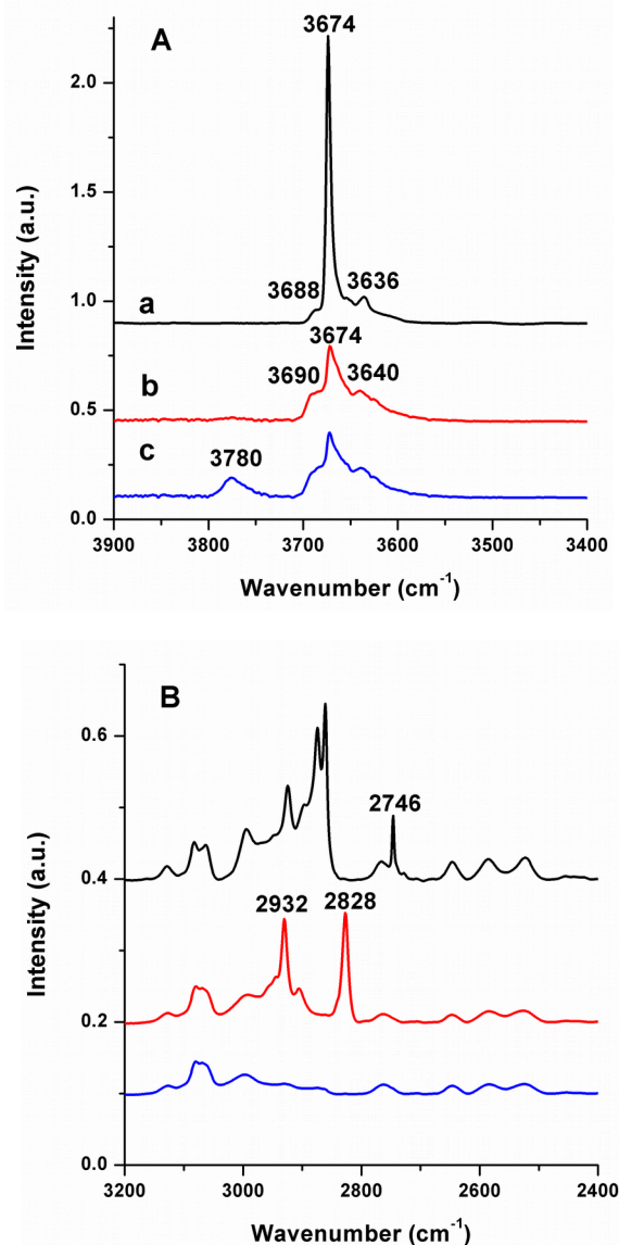
Figure 2. IR spectra in the (A) 3400-3900 \text{cm}^{-1} region and (B) 2400-3200 \text{cm}^{-1} region characterizing (a) UiO-66 and (b) UiO-66 after treatment in liquid methanol at 298 K for 48 h and (c) UiO-66 after treatment in water vapor/helium at 393 K for 30 min. The UiO-66 samples before and after treatment with liquid methanol or water vapor were activated at 393 K or 423 K, respectively, by treatment under high vacuum for 12 h.
