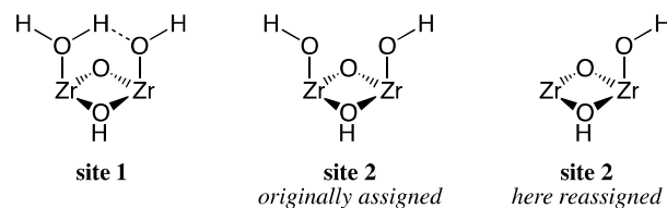
Scheme 1. Simplified depictions of the Zr 6 node-face topologies, site 1 and site 2 , the latter both as originally assigned and as reassigned here in light of new results, for the MOFs UiO-66 and NU-1000. Note that the originally assigned site 2 was for a Zr 6 node with the otherwise “missing” proton from site 1 moved to another face of the core ( i.e. , all of the sites in this scheme have zero net charge and spin).
