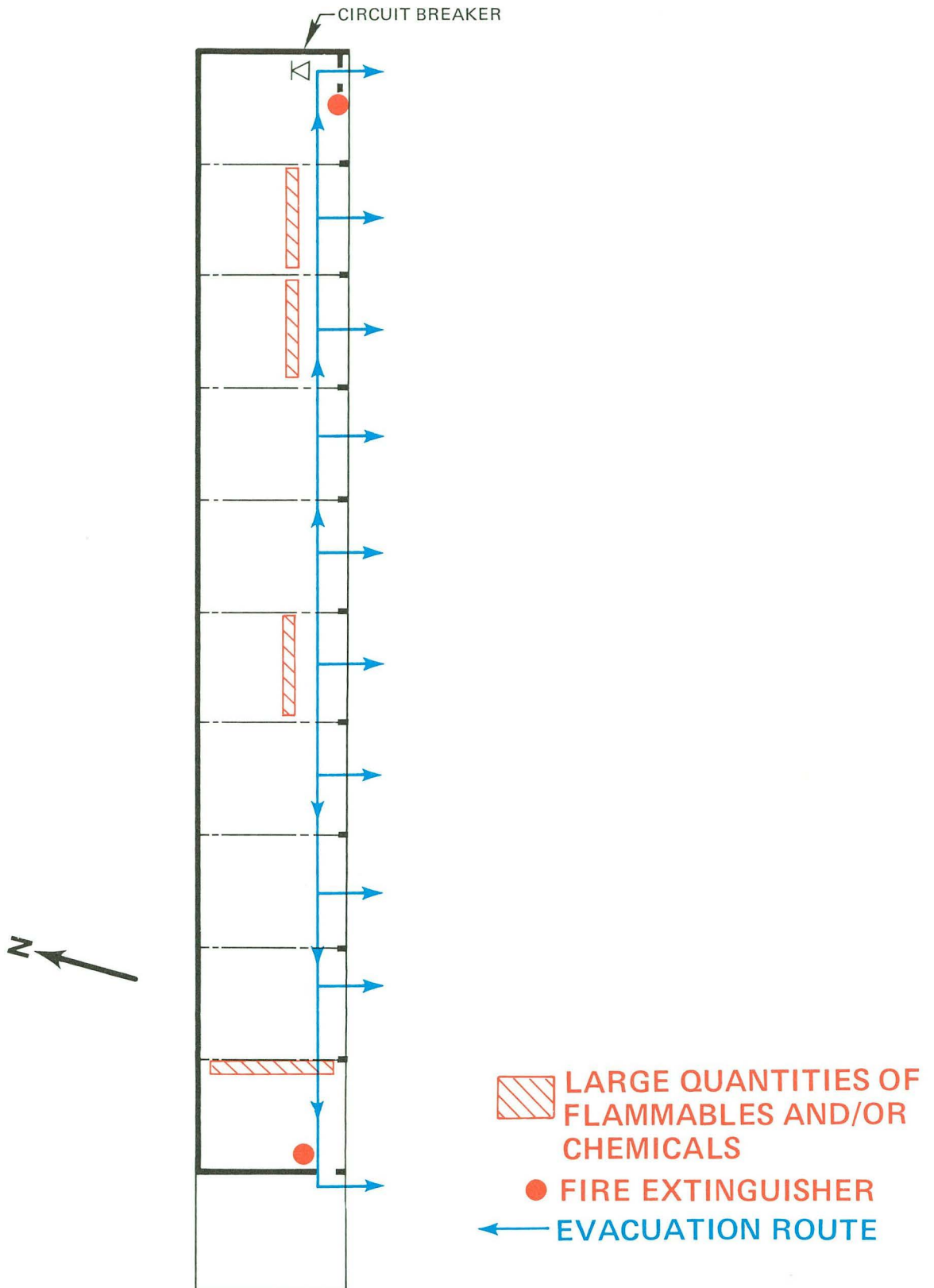
Fig. 8. Building 78, evacuation routes and fire equipment.
