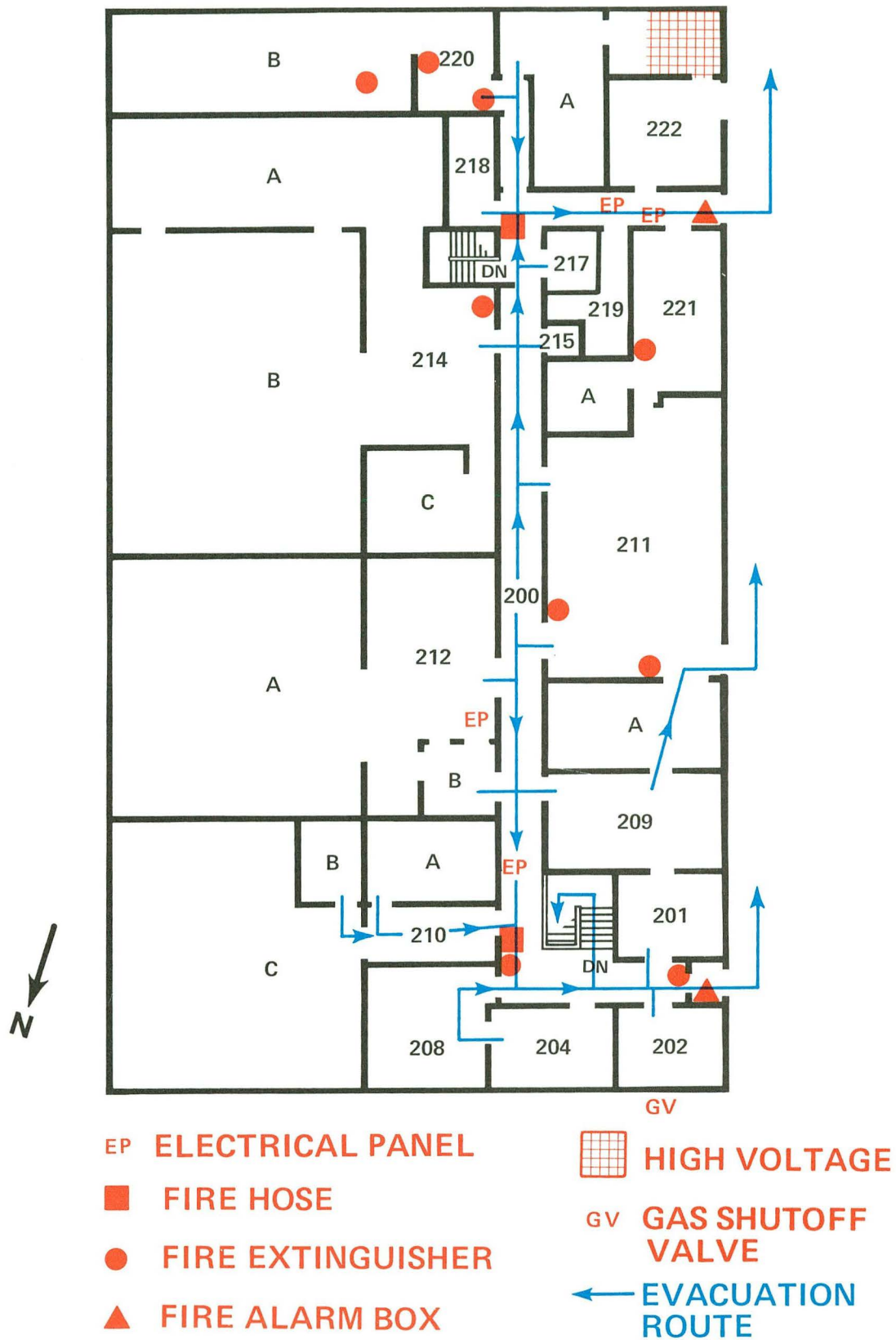
Fig. 3. Building 7, 2nd Floor evacuation routes and fire equipment.
