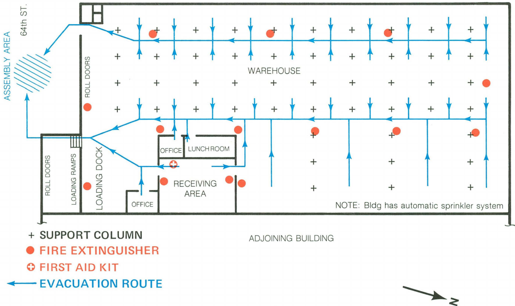
Fig. 10. Building 901, evacuation routes, assembly area, and fire equipment.
