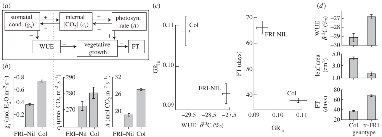
Figure 3. FRI pleiotropically affects WUE, GR_{la} and FT. (a) The conceptual model demonstrates the mechanism of pleiotropy, upstream variation in gas exchange causes subsequent changes in GR_{la} and FT. (b) FRI -NILs show reduced gas exchange compared with WT Col-0. (c) FRI -NILs have increased WUE and reduced GR_{la} compared with WT Col-0. (d) Transgenic overexpression lines show the same pattern as the FRI -NIL. Least square means \pm s.e. are presented in (b–d).
