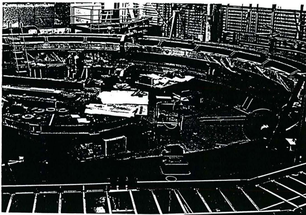
Fig. 2 The g-2 Storage Ring (June 1995) before the Electron Detectors were Installed inside of the Storage Ring
