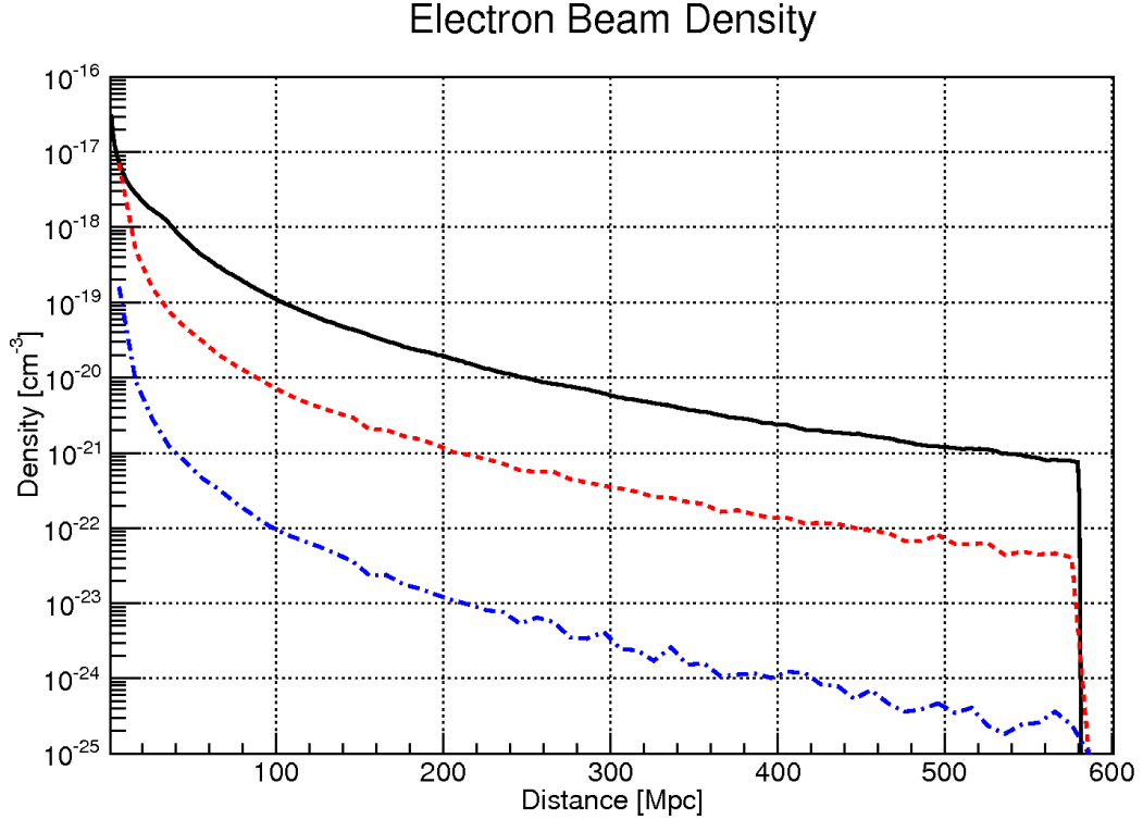
Figure 7.1 Electron Density as a function of distance from source 1ES 0229+200, assuming a normal EBL model (EBL model 1) and a spectral index in the VHE band ( \alpha ) of 1.3 and cutoff energy ( \varepsilon_c ) 3.16 TeV. The black (solid) line traces the density of electrons with energies > 10 GeV, the red (dashed) line represents the density of electrons with energies > 100 GeV, and the blue (dot-dashed) line corresponds to energies > 1 TeV.
