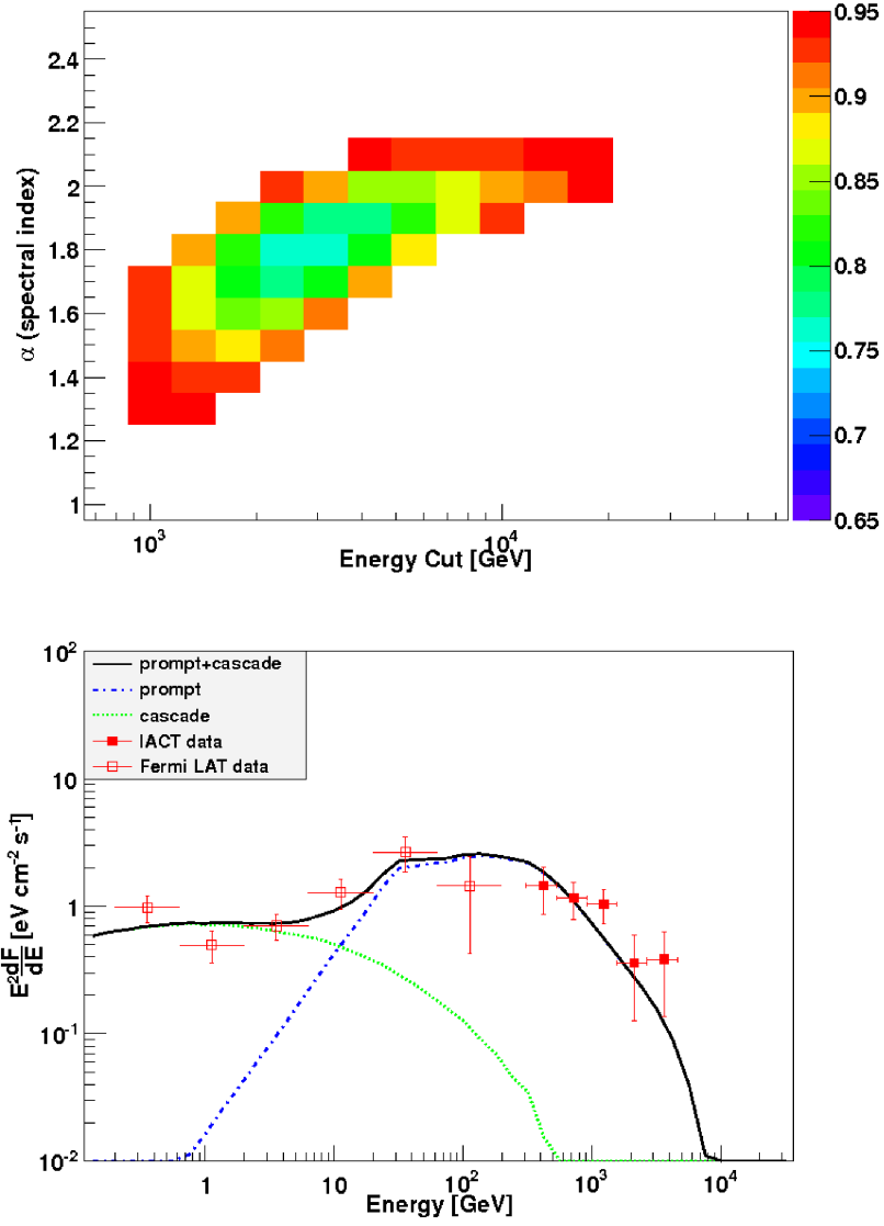
Figure 5.6 Source RGB J0710+591 analyzed under the assumption of H0 . (top) Confidence level, or the probability of exclusion of the gamma-ray source model (with fixed \alpha and \epsilon_c ), where the remaining three parameters of the model ( \gamma , \epsilon_B , and F_0 , see Eq. 3.9) are chosen so as to minimize \chi^2 . (bottom) Simulated dFED of the best fit model, of \alpha = 1.8 , \epsilon_c = 3.16 TeV, showing both the prompt and secondary cascade contributions to the total dFED, along with the HE and VHE data.
