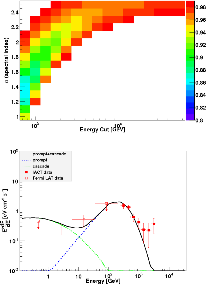
Figure 5.2 Source 1ES 0347-121 analyzed under the assumption of H0 . (top) Confidence level, or the probability of exclusion of the gamma-ray source model (with fixed \alpha and \epsilon_c ), where the remaining three parameters of the model ( \gamma , \epsilon_B , and F_0 , see Eq. 3.9) are chosen so as to minimize \chi^2 . (bottom) Simulated dFED of the best fit model of \alpha = 1.3 , \epsilon_c = 0.75 TeV, showing both the prompt and secondary cascade contributions to the total dFED, along with the HE and VHE data.
