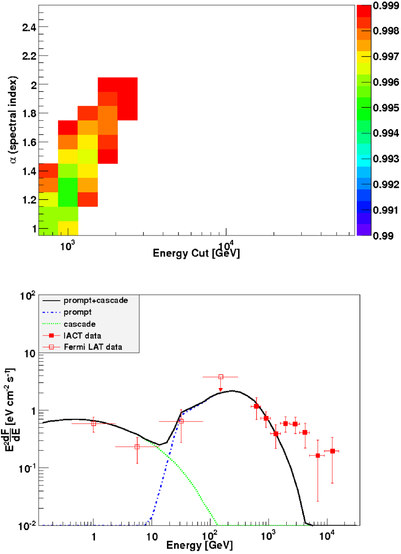
Figure 5.8 Source 1ES 0229+200 analyzed under the assumption of H0 . (top) Confidence level, or the probability of exclusion of the gamma-ray source model (with fixed \alpha and \epsilon_c ), where the remaining three parameters of the model ( \gamma , \epsilon_B , and F_0 , see Eq. 3.9) are chosen so as to minimize \chi^2 . (bottom) Simulated dFED of the best fit model (C.L. = 0.995) of \alpha = 1.3 , \epsilon_c = 1 TeV, showing both the prompt and secondary cascade contributions to the total dFED, along with the HE and VHE data.
