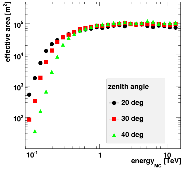
Figure 4.9 VERITAS effective area for three different zenith angles with (top) standard cuts analysis and (bottom) for soft cuts analysis.
