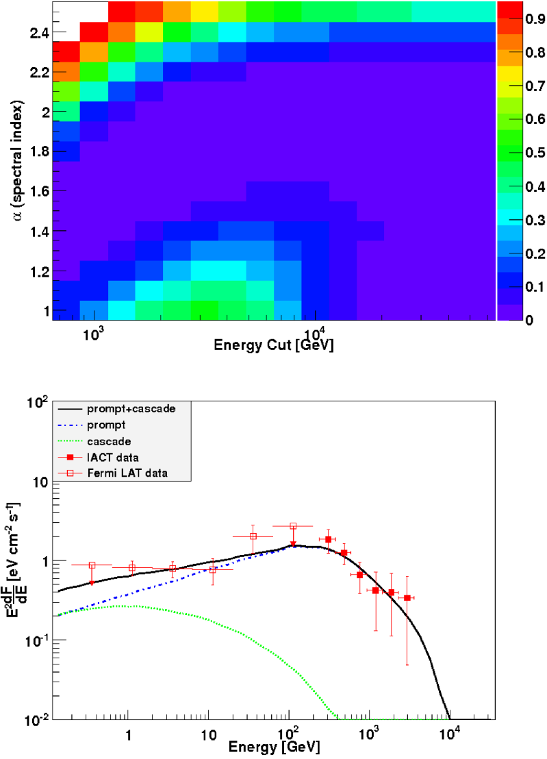
Figure 5.5 RGB J0152+017 (top) Confidence level, or the probability of exclusion of the gamma-ray source model (with fixed \alpha and \epsilon_c ), where the remaining three parameters of the model ( \gamma , \epsilon_B , and F_0 , see Eq. 3.9) are chosen so as to minimize \chi^2 . (bottom) Simulated dFED of the best fit model of \alpha = 1.9 , \epsilon_c = 3.16 TeV, showing both the prompt and secondary cascade contributions to the total dFED, along with the HE and VHE data.
