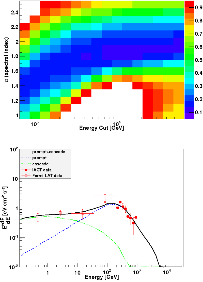
Figure 5.4 Source H 2356-309 analyzed under the assumption of H0 . (top) Confidence level, or the probability of exclusion of the gamma-ray source model (with fixed \alpha and \epsilon_c ), where the remaining three parameters of the model ( \gamma , \epsilon_B , and F_0 , see Eq. 3.9) are chosen so as to minimize \chi^2 . (bottom) Simulated dFED of the best fit model of \alpha = 1.8 , \epsilon_c = 4.22 TeV, showing both the prompt and secondary cascade contributions to the total dFED, along with the HE and VHE data.
