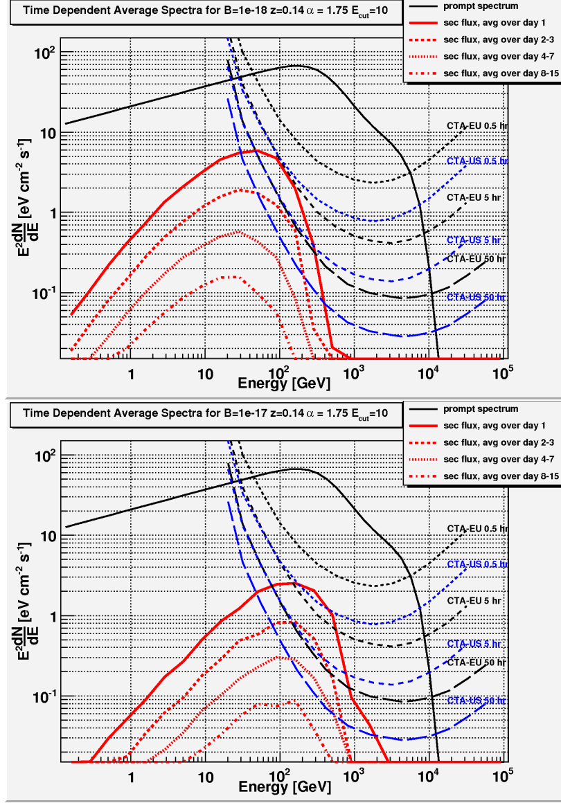
Figure 6.6 Simulated spectra for a source at z=0.14 , for a flare with spectral index = 1.75 , and cutoff energy 10 TeV, and (top) B_{\text{IGMF}} = 10^{-18} \text{ G} and (bottom) B_{\text{IGMF}} = 10^{-17} \text{ G} .
