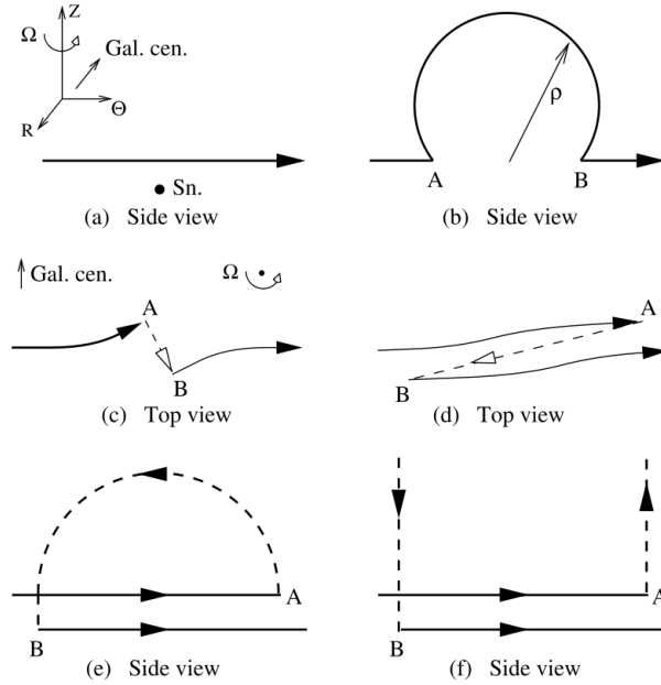
Figure 1.1 (Figure taken from [KZ08]). The operation of the \alpha - \Omega dynamo. In (a) and (b) a supernova (noted as Sn) blows the magnetic loop. It is twisted into the poloidal plane by Coriolis forces as is seen in the top view of (c). The dashed line represents the upper part of the loop. In (d) the lower part of the line is stretched by differential rotation. Then the upper part of the line is removed to infinity as in (e) and (f).
