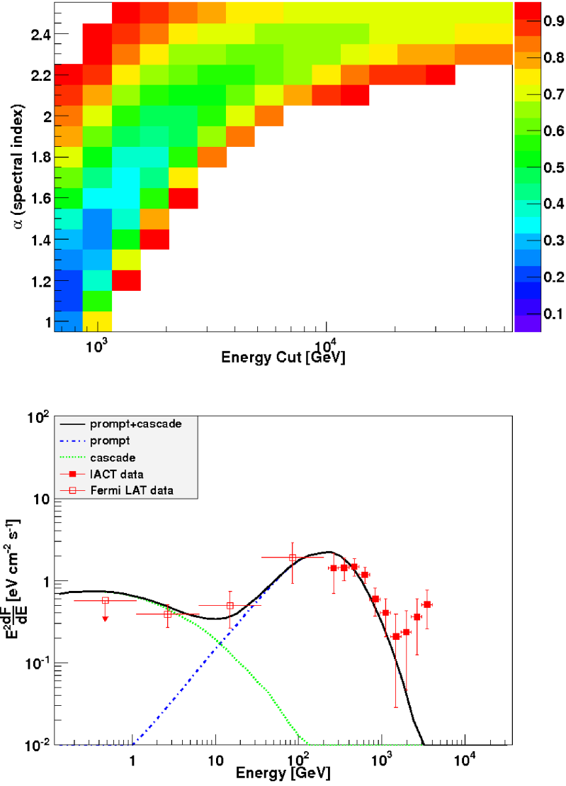
Figure 5.3 Source 1ES 1101-232 analyzed under the assumption of H0 . (top) Confidence level, or the probability of exclusion of the gamma-ray source model (with fixed \alpha and \epsilon_c ), where the remaining three parameters of the model ( \gamma , \epsilon_B , and F_0 , see Eq. 3.9) are chosen so as to minimize \chi^2 . (bottom) Simulated dFED of the best fit model of \alpha = 1.2 , \epsilon_c = 0.75 TeV, showing both the prompt and secondary cascade contributions to the total dFED, along with the HE and VHE data.
