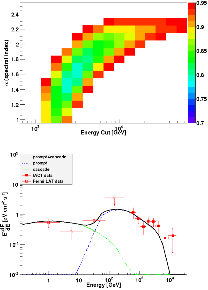
Figure 5.10 Source 1ES 0229+200 analyzed, assuming EBL Model 3 and H0 . (top) Confidence level, or the probability of exclusion of the gamma-ray source model (with fixed \alpha and \epsilon_c ), where the remaining three parameters of the model ( \gamma , \epsilon_B , and F_0 , see Eq. 3.9) are chosen so as to minimize \chi^2 . (bottom) Simulated dFED of the best fit model (C.L. = 0.78) of \alpha = 1.6 , \epsilon_c = 3.16 TeV, showing both the prompt and secondary cascade contributions to the total dFED, along with the HE and VHE data.
