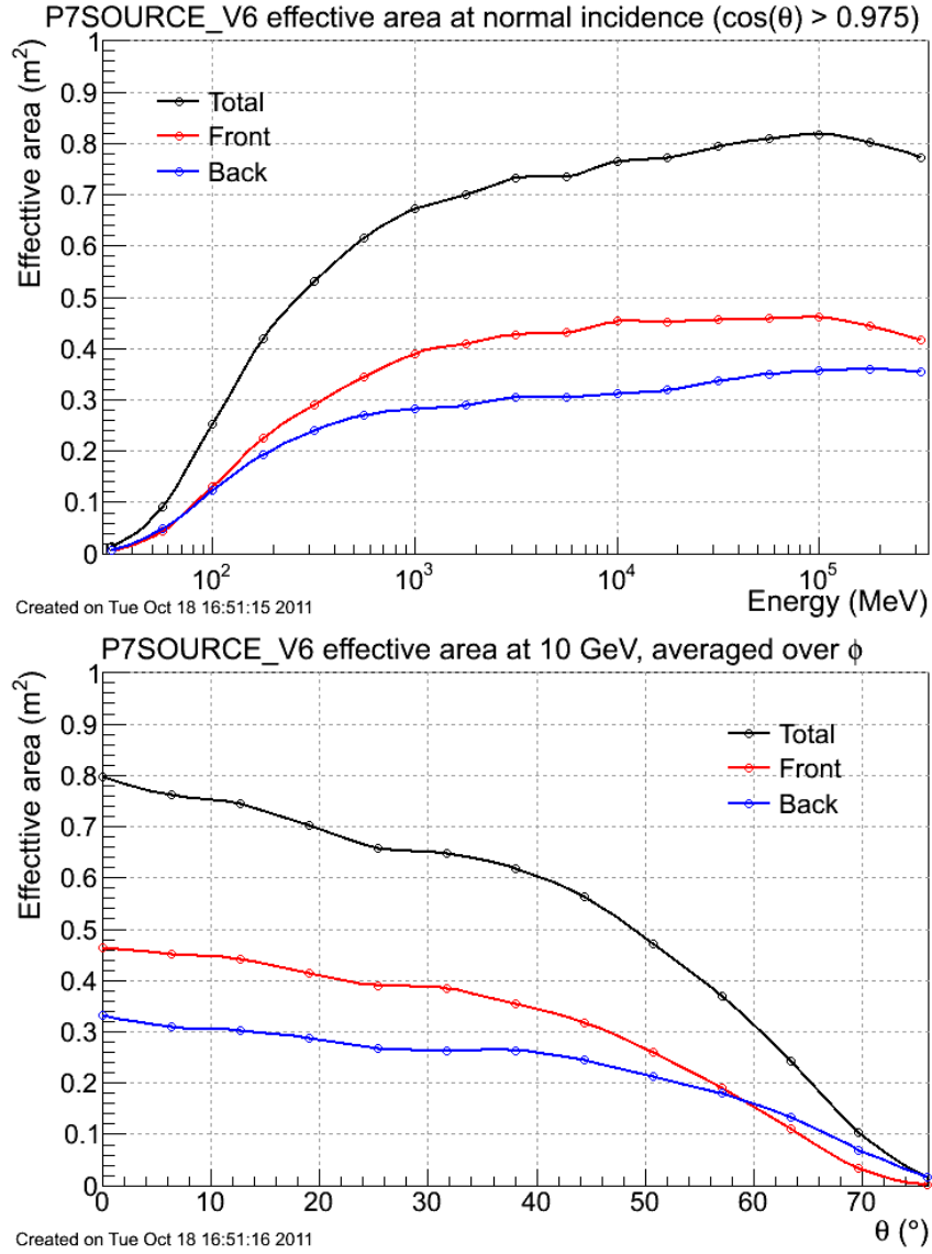
Figure 4.2 LAT Effective Area curves as a function of various parameters. (top) The Effective Area as a function of energy for photons impinging on the LAT at an angle defined by \cos \theta > 0.975 . (bottom) Effective Area as a function of polar incidence angle, for photons of energy 10 GeV.
