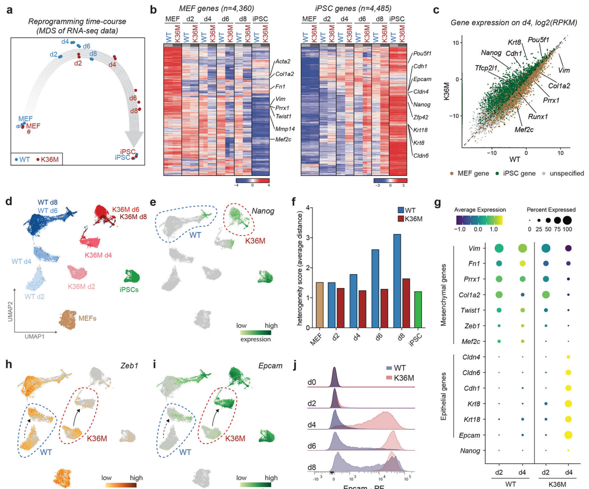
Fig. 2: K36M endows iPSC intermediates with transcriptional homogeneity and epithelial plasticity.
