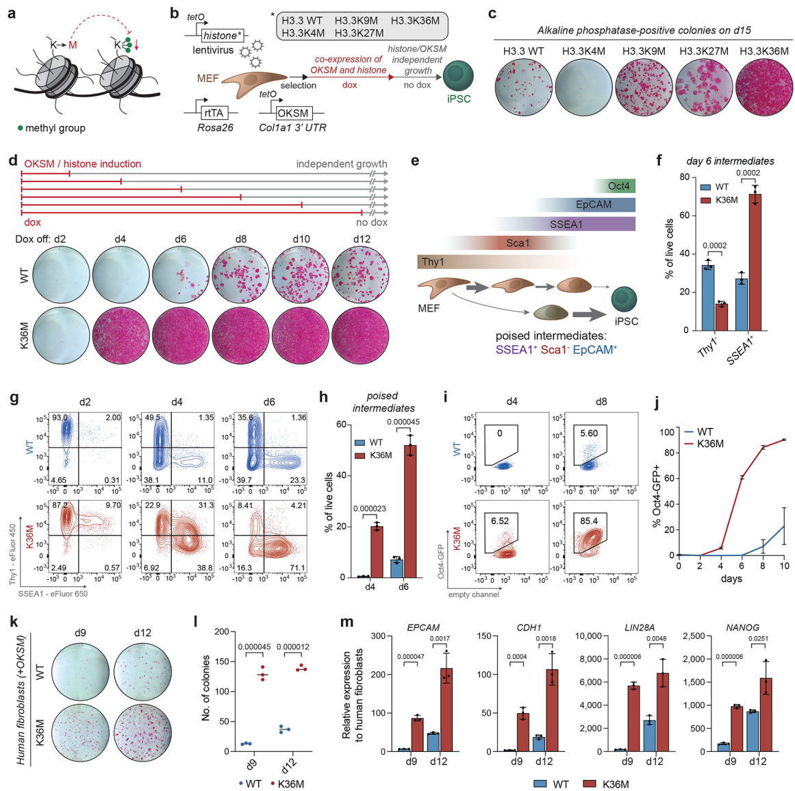
Fig. 1: Histone mutant analysis reveals crucial role of H3K36-methylation in cell identity maintenance.
