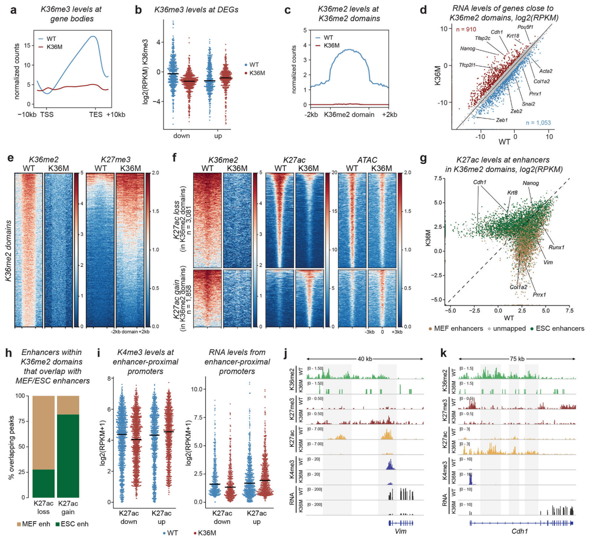
Fig. 4: K36M decommissions MEF enhancers and activates ESC enhancers.
