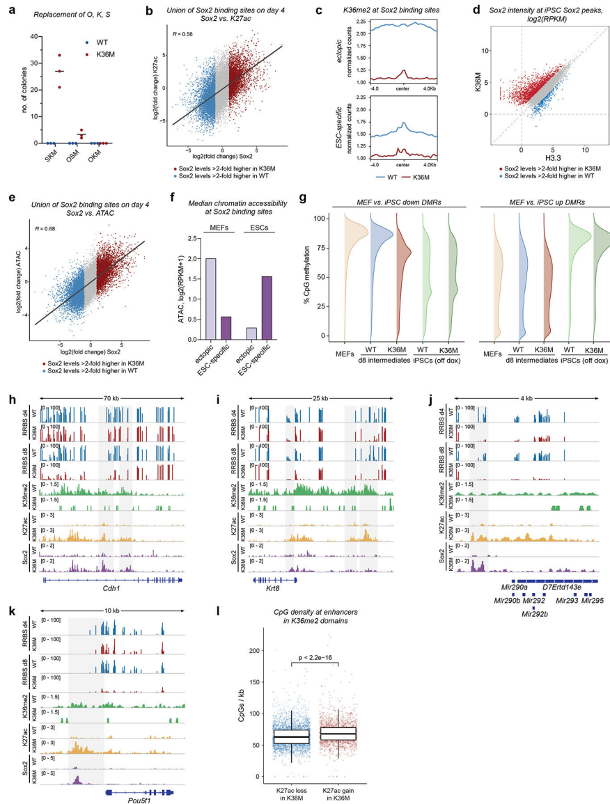
Extended Data Fig. 9: K36M rewires DNA methylation patterns.
