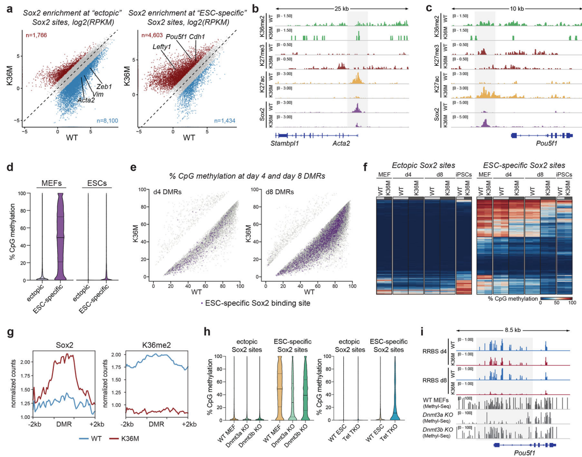
Fig. 5: K36M-dependent chromatin rewiring alters transcription factor binding preferences.
