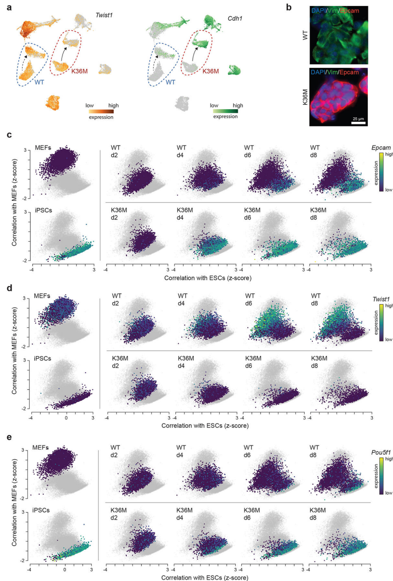
Extended Data Fig. 4: K36M confers epithelial plasticity on cells undergoing reprogramming. (a) Gene expression of Twist1 and Cdh1 on the same UMAP embedding as used in Fig. 2d. Dashed circles encompass day-2 and day-4 samples for WT (blue circle) and K36M (red
