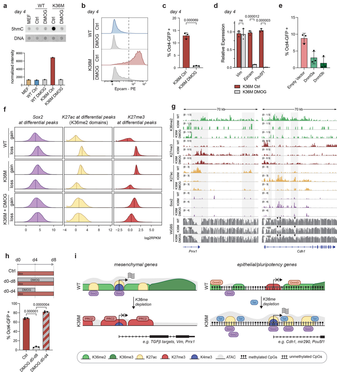
Fig. 6: DNA demethylation is limiting for K36M-dependent enhancer activation and reprogramming.
