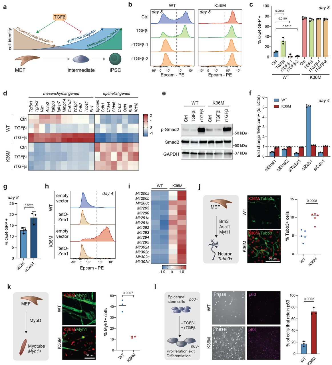
Fig. 3: K36M acts downstream of TGFβ and Smad2 but upstream of Zeb1.
