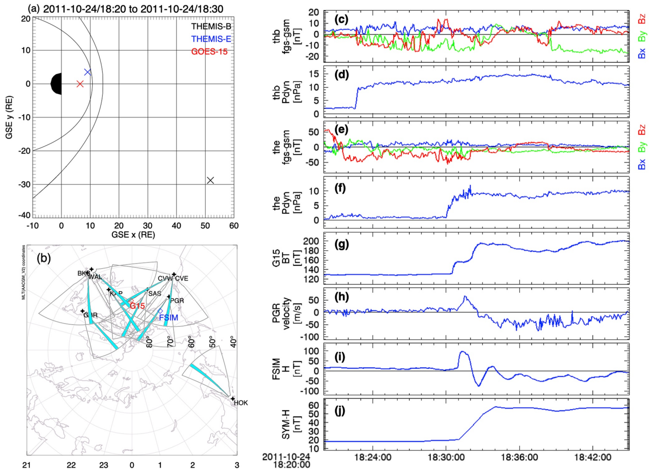
Figure 1. (Left) Locations of (a) Time History of Events and Macroscale Interactions during Substorms (THEMIS) B (black) and E (blue) spacecraft and Geostationary Operational Environment Satellite (GOES) 15 (red) satellite in the X–Y plane in Geocentric Solar Ecliptic (GSE) coordinates from 18:20 UT to 18:30 UT on 24 October 2011; (b) locations of the ionospheric footprint of GOES 15 (red), the Fort Simpson (FSIM) ground magnetometer (blue), and Super Dual Auroral Radar Network (SuperDARN) radar fields of view and THEMIS mode camping beams (cyan) in altitude-adjusted corrected geomagnetic coordinates at 18:32 UT. Right: space and ground observations from 18:20 UT to 18:45 UT of (c and d) interplanetary magnetic field components and solar wind dynamic pressure from THEMIS B spacecraft measurements; (e and f) magnetic field components and dynamic pressure from THEMIS E spacecraft measurements; (g) total magnetic field from the GOES 15 satellite; (h) Doppler velocity measurements from the SuperDARN Prince George radar (beam 12 and gate 11); (i) detrended horizontal magnetic field from the FSIM ground magnetometer; (j) SYM-H index.
