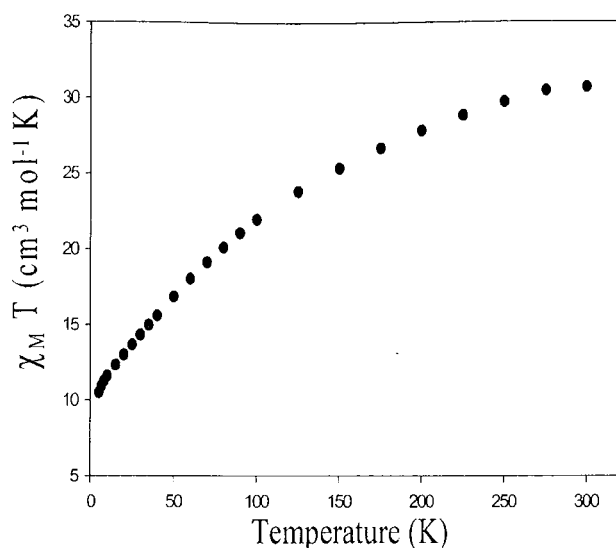
Figure 3. \chi_M T vs T plot for complex 1 .
