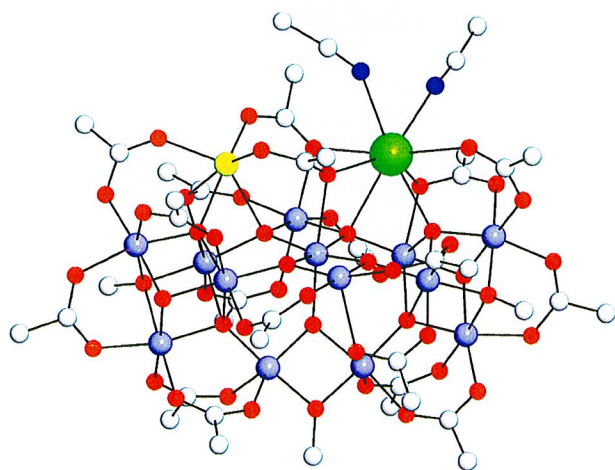
Figure 2. Labeled [\text{Mn}_{14}\text{SrO}_{13}(\text{OMe})_3]^{14+} core of complex 1 . Color scheme: Mn III , light blue; Mn II , yellow; Sr, green; O, red; C, grey. H atoms have been omitted for clarity.
