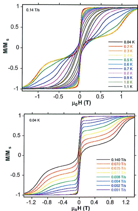
Figure 6. Magnetization ( M ) vs DC field ( H ) hysteresis loops for a single crystal of 1 in 12 MeCN: (top) at the indicated temperatures and a fixed field sweep rate of 0.14 T/s; and (bottom) at the indicated field sweep rates and a fixed temperature of 0.04 K. The magnetization is normalized to its saturation value, M_S .
