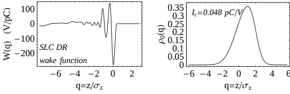
Figure 1: Wake function for the SLC Damping Ring and Haissinski distribution for I_c = 0.048 V/pC.
