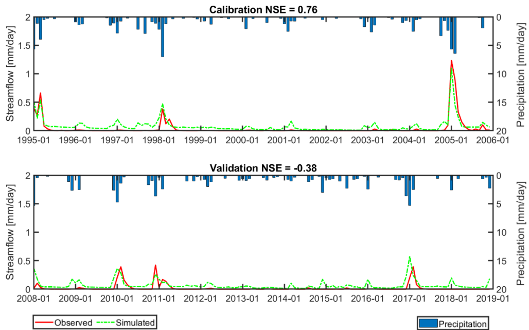
Figure 30. Subbasin 154 mean monthly streamflow (mm/day) – top: calibration (1995 - 2005) and bottom: validation (2008 - 2018).
