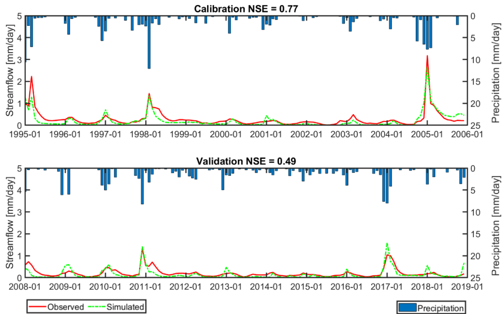
Figure 25. Subbasin 143 mean monthly streamflow (mm/day) – top: calibration (1995 - 2005) and bottom: validation (2008 - 2018).
