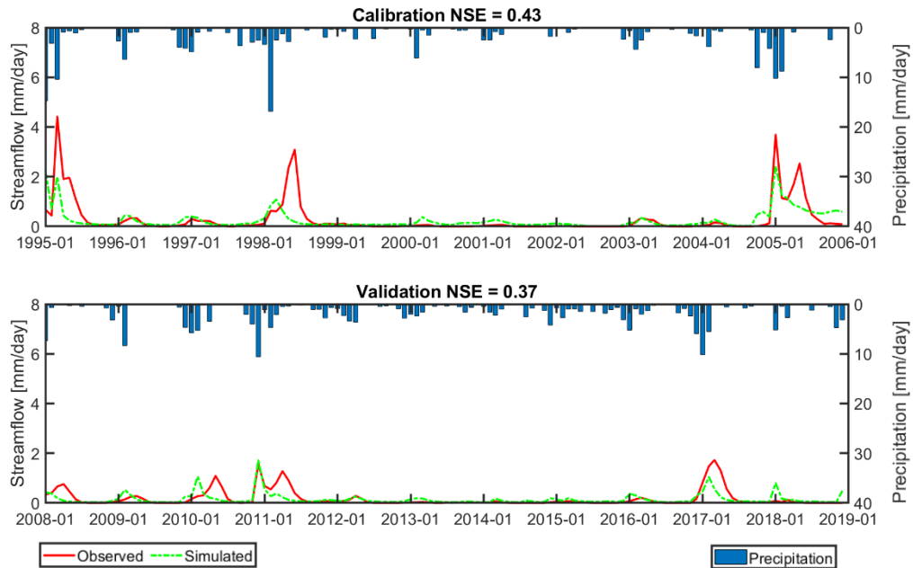
Figure 26. Subbasin 145 mean monthly streamflow (mm/day) – top: calibration (1995 - 2005) and bottom: validation (2008 - 2018).
