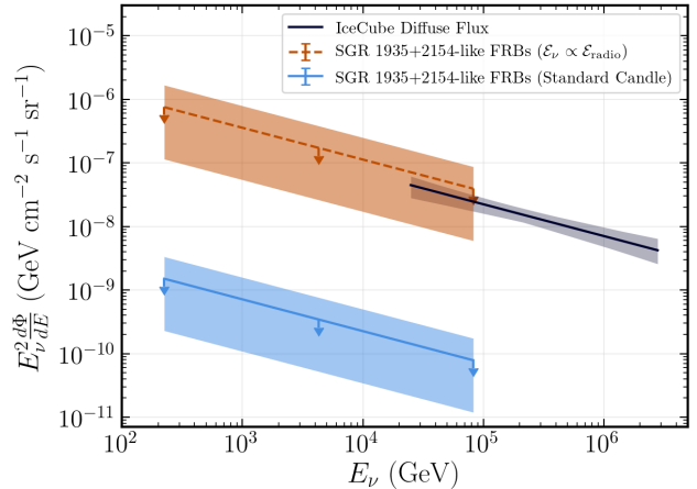
Figure 8. Upper limits on the contribution to the diffuse neutrino flux from a population of FRBs similar to SGR 1935+2154, for a variety of luminosity functions. The rate of such a population is taken from Bochenek et al. (2020), and the limit on the neutrino luminosity is derived from our analysis of FRB 200428. For a naive standard candle assumption (light blue), the strict upper limit from the Galactic burst limits the contribution of FRBs to be less than 1% of the diffuse astrophysical neutrino flux. However, if the emitted energy in neutrinos were to scale linearly with the energy emitted at radio wavelengths (dashed orange), as described in the text, then FRBs are not ruled out as contributing significantly to the diffuse neutrino flux. The band on each of these limits represents the uncertainty on the reported volumetric rate of these transients.
