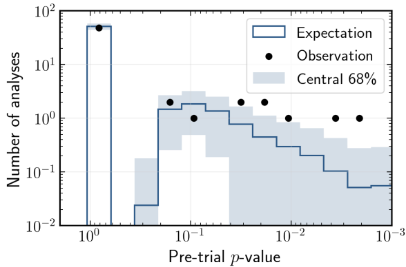
Figure 5. Distribution of p -values from all analyses. The p -values represent the outcome of each individual analysis, and do not include a trials correction for the ensemble of all analyses performed. As many of these analyses are looking for coincidences over short time windows, a large fraction of analyses have zero coincident events, yielding \mathcal{T} = 0 , and a p -value of exactly 1.0. We compare our distribution of p -values to those expected from many sets of ensembles of pseudo-experiments from scrambled background data for each of the 58 analyses performed.
