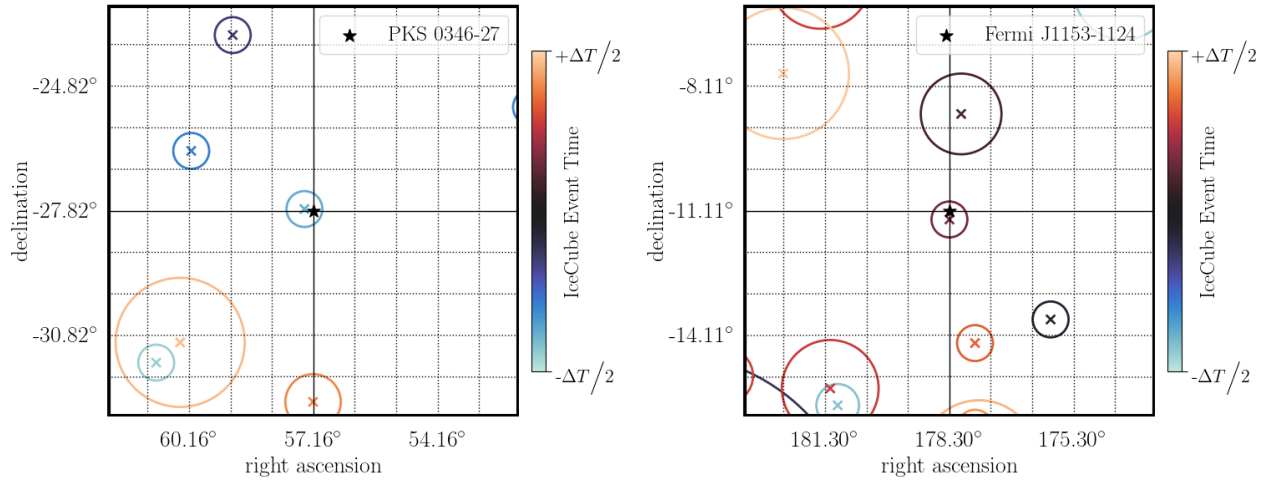
Figure 9. Skymaps for the two analyses which resulted in a p -value less than 0.01, pre-trials. Maps are centered on the location of the source being investigated. Each colored \times represents a neutrino candidate event in the GFU sample, the color represents the arrival time of the event, and the size of the circle is each event’s angular uncertainty (90% containment). The analysis for PKS 0346-27 (left) lasted four days containing a period of increased gamma-ray emission detected by Fermi -LAT and the analysis of a newly detected gamma-ray source Fermi J1153-1124 (right) was 2 days in duration.
