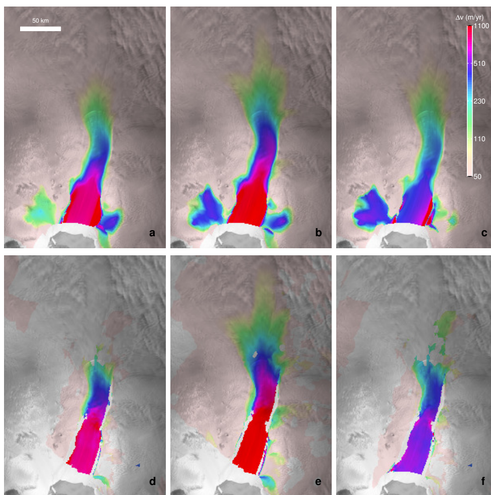
Figure 7. Changes in observed and modeled velocities in \text{m yr}^{-1} on a logarithmic scale. (a) Modeled year 11–year 1, (b) modeled year 15–year 1, (c) modeled year 15–year 11, (d) , observed 2006–1996, (e) observed 2010–1996, (f) observed 2011–2006. Modeled velocities are from the increased basal melting experiment (melting multiplied by 1.5).
