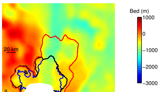
Figure 10. Grounding line position at the beginning of the experiments (blue line), and at the end of the melting experiments in the case of \beta = 1 (black line) and for a basal melting rate parameterization based on the ice shelf base elevation similar to Favier et al. (2014) (red line), overlain on the bedrock elevation.
