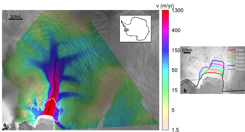
Figure 1. (a) Initial modeled 2008 velocity of Pine Island Glacier, overlain on a MODIS Mosaic of Antarctica with initial grounding line position (white) and glacier centerline (black). (b) Ice front positions used in the sensitivity study.
