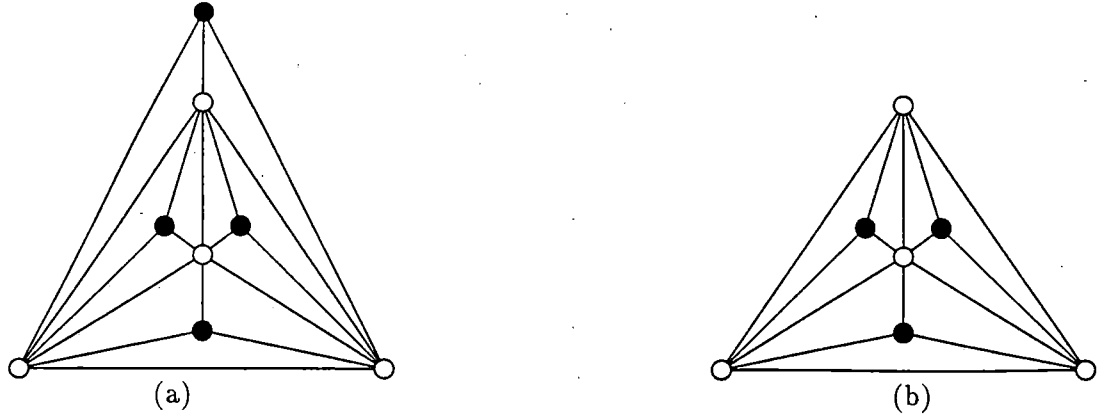
Figure 1: (a) The stellated tetrahedron is Hamiltonian, but noninscribable. (b) This graph is 1-Hamiltonian and has a Hamiltonian cycle passing through every edge, but it is not Delaunay realizable.
