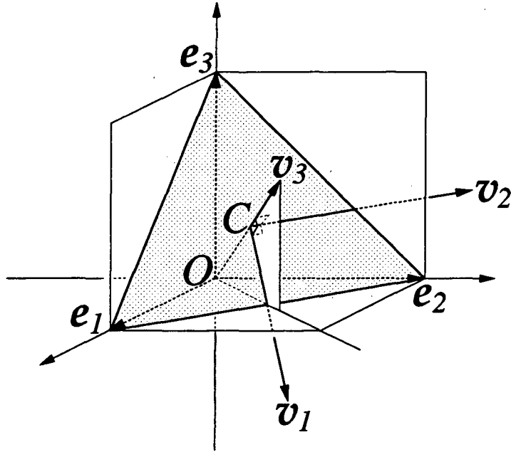
Figure 1: S_3 acts as a rotation of the triangle spanned by three orthonormal vectors e_{1,2,3} . The vector v_3 corresponds to the 1_A representation, and two vectors v_{1,2} , in the plane of the triangle, to the 2 representation.
