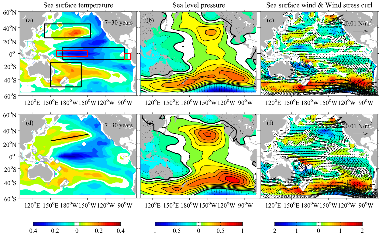
FIG. 6. The (a),(d) SST ( ^{\circ}\text{C} ), (b),(e) SLP (hPa), and (c),(f) sea surface wind stress ( \text{N m}^{-2} ; vectors) and wind stress curl ( 10^{-8} \text{ N m}^{-3} ; color shading) patterns corresponding to the Pacific QD sea level mode as shown in Figs. 5a–c, derived from the SVD1 of 7–30-yr bandpass-filtered sea level and each of the other variables based on (top) OFES and NCEP–NCAR data and (bottom) steric sea level and JRA-55 data. The three regions used to define the IPO index (Henley et al. 2015) are shown with black boxes in (a). The red boxes in (a) indicate the Niño-4 and Niño-1+2 regions. The black line in (d) marks the orientation of SST anomalies in the central–western North Pacific.
