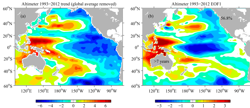
FIG. 1. (a) Altimeter-observed sea level linear trend ( \text{mm yr}^{-1} ) during 1993–2012 in the Pacific with the global mean ( \sim 3.2 \text{ mm yr}^{-1} ) removed; (b) the EOF1 pattern of low-frequency ( >7 \text{ yr} ) sea level variations (cm) in the Pacific for the altimeter data. The percentages in (b) represent the percent of variance explained by EOF1.
