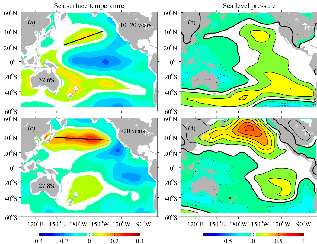
FIG. 10. The ENSO-like QD variability patterns, derived as the SVD1 patterns of 10–20-yr bandpass-filtered (a) SST ( ^{\circ}\text{C} ) and (b) SLP (hPa) in the Pacific over 1860–2012. (c),(d) As in (a),(b), but for the ENSO-like MD variability patterns, derived as the SVD1 patterns of 20-yr low-pass-filtered SST and SLP in the Pacific over 1910–2012. The data are from the ERSST and the NOAA CIRES 20CR. In (a),(c), the black lines mark the orientation of SST anomalies in the central–western North Pacific. The percentages in (a),(c) represent the percent of variance explained by the SVD1.
