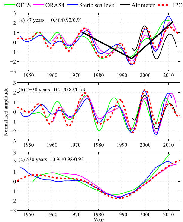
FIG. 3. The EOF1 time series of sea level variations in the Pacific on time scales (a) >7 , (b) between 7 and 30, and (c) >30 yr from the altimeter (black), OFES (green), ORAS4 (magenta), and steric sea level (blue). The reversed IPO index time series on corresponding time scales are also shown (red dashed lines). The numbers at the top left in each panel indicate the correlations between the reversed IPO index and the EOF1 time series on corresponding time scales for OFES, ORAS4, and steric sea level. The thick black lines in (a) roughly mark the trend reversal before and after the early 1990s.
