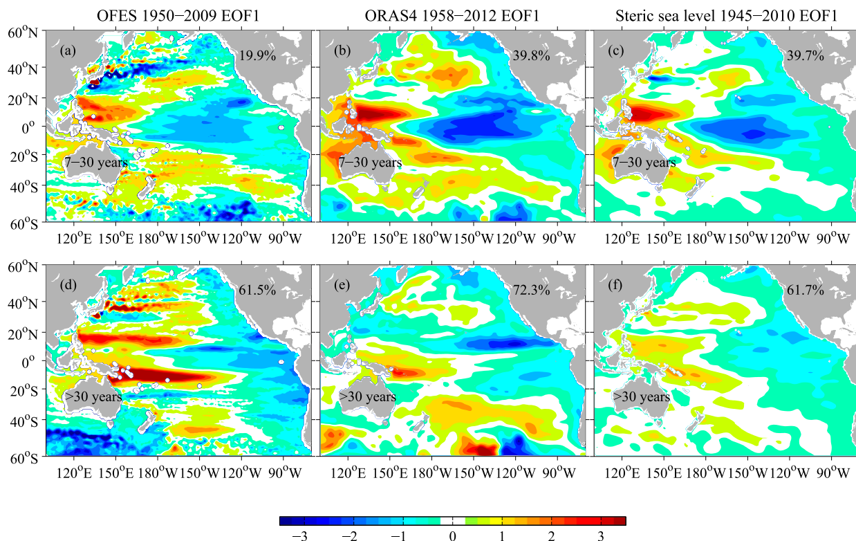
FIG. 5. The EOF1 patterns of sea level variations (cm) in the Pacific on time scales (a)–(c) between 7 and 30 yr, and (d)–(f) >30 yr from the (left) OFES, (center) ORAS4, and (right) steric sea level. The percentage in each panel represents the percent of variance explained by the EOF1.
