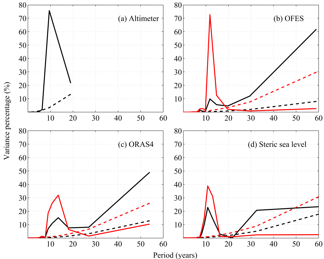
FIG. 4. Power spectra of the EOF1 time series of sea level variations in the Pacific on time scales >7 yr (black) and between 7 and 30 yr (red) for the (a) altimeter, (b) OFES, (c) ORAS4, and (d) steric sea level. The y axis is plotted as the percent of variance explained by the signal at a particular period. Dashed lines represent the 95% significance level.
