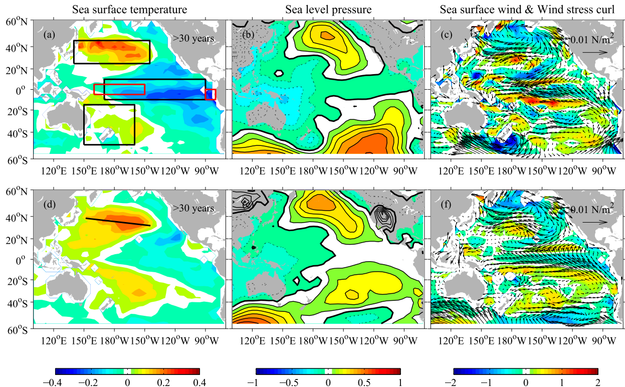
FIG. 8. As in Fig. 6, but for patterns corresponding to the Pacific MD sea level mode as shown in Figs. 5d–f, derived from the SVD1 of 30-yr low-pass-filtered sea level and each of the other variables.
