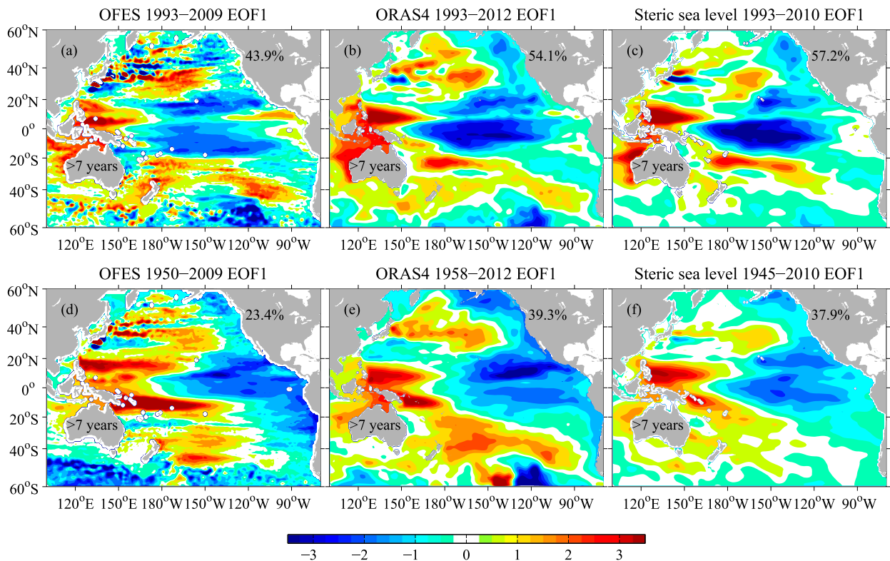
FIG. 2. The EOF1 patterns of low-frequency (>7 yr) sea level variations (cm) in the Pacific from the (a),(d) OFES, (b),(e) ORAS4, and (c),(f) steric sea level based on (top) data after 1993 and (bottom) data over the full available period. The percentages in each panel represent the percent of variance explained by EOF1.
