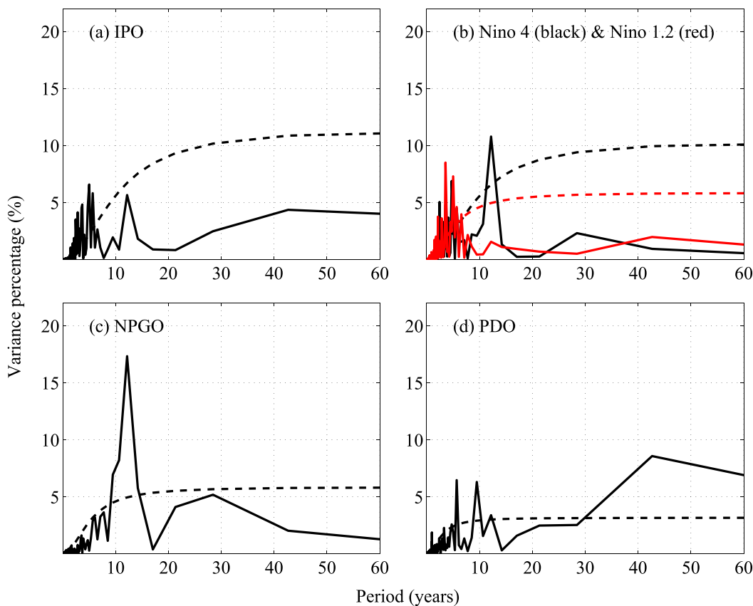
FIG. 7. Power spectra of the (a) IPO, (b) Niño-4 and Niño-1+2 SST, (c) NPGO, and (d) PDO indices since 1950. The y axis is plotted as the percent of variance explained by the signal at a particular period. Dashed lines represent the 95% significance level.
