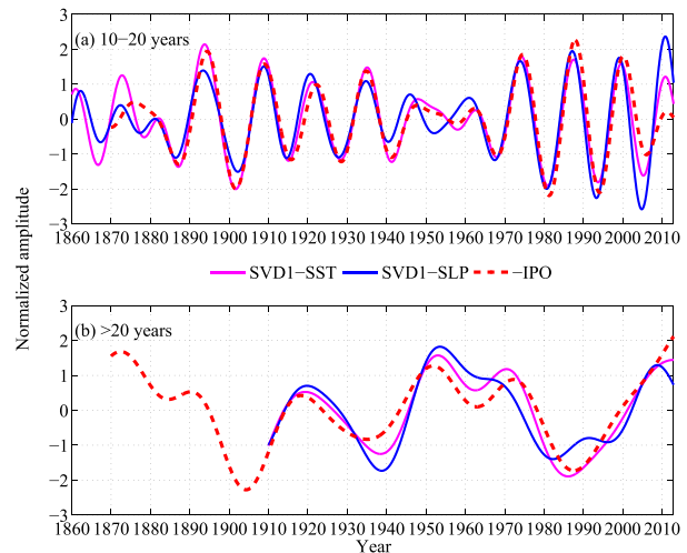
FIG. 9. The SVD1 time series of SST and SLP in the Pacific on time scales (a) between 10 and 20 yr and (b) >20 yr. The reversed IPO index time series on corresponding time scales are also shown (red dashed lines).
