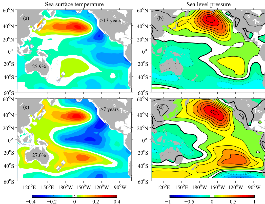
FIG. 11. As in Fig. 10, but over 1910–2012 on time scales (a),(b) >13 and (c),(d) >7 yr.
