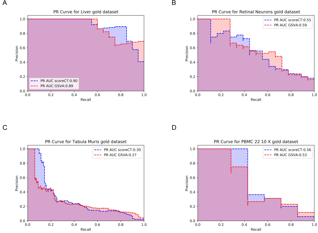
Figure 2.4: scoreCT comparison with GSVA on selected scRNA-seq datasets. We compared scoreCT predictions to GSVA , a top performing method evaluated in [Diaz-Mejia et al., 2019] and show precision-recall curves for the (A) liver dataset from [MacParland et al., 2018], (B) retinal neurons dataset from [Shekhar et al., 2016] (C) Tabula Muris atlas [Schaum et al., 2018] and (D) PBMC dataset from [Zheng et al., 2017] .
