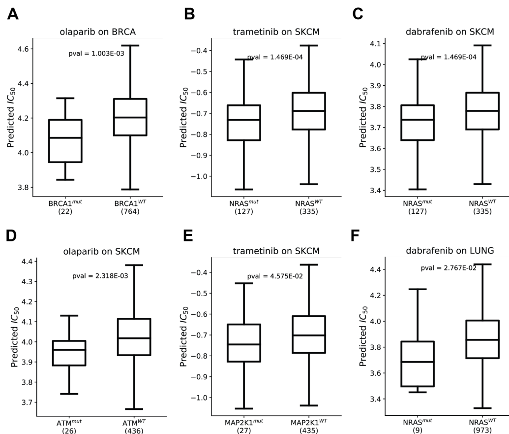
Figure 4. Functional Analysis. (A) Predicted log( IC_{50} ) for BRCA1 mutant and wild-type (WT) breast cancer (BRCA) samples in-silico treated with olaparib. P-value corresponds to the one-sided Mann Whitney U test discriminating between mutant and WT predicted log( IC_{50} ). (B) Predicted log( IC_{50} ) for NRAS mutant and wild-type (WT) melanoma (SKCM) samples in-silico treated with trametinib. (C) Predicted log( IC_{50} ) for NRAS mutant and wild-type (WT) melanoma (SKCM) samples in-silico treated with dabrafenib. (D) Predicted log( IC_{50} ) for ATM mutant and wild-type (WT) melanoma (SKCM) samples in-silico treated with olaparib. (E) Predicted log( IC_{50} ) for MAP2K1 mutant and wild-type (WT) melanoma (SKCM) samples in-silico treated with trametinib. (F) Predicted log( IC_{50} ) for NRAS mutant and wild-type (WT) LUSC/LUAD (LUNG) samples in-silico treated with dabrafenib.
