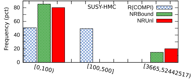
Figure 2.10: Constraint set size distribution for SUSY-HMC.
