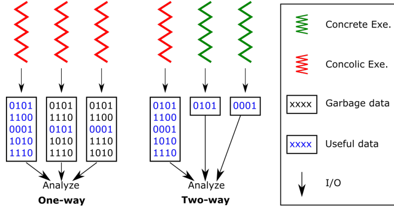
Figure 2.7: Instrumentation comparison: one-way v.s. two-way.
