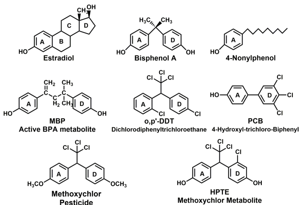
Figure 4. Synthetic chemicals that act as endocrine disruptors. Many synthetic chemicals used in plastics and other industrial products contain a phenolic group that mimic the A ring of estradiol or two phenolic groups that mimic the A and D rings of estradiol [40, 77]. For example, bisphenol A, which is used in plastics and is widespread in the environment, is a xeno-estrogen [40, 41, 114]. BPA can be metabolized to 4-methyl-2,4-bis(4-hydroxyphenyl)pent-1-ene (MBP), which has transcriptional activity at nM concentrations [115, 116]. Metabolism of the pesticide methoxychlor [1,1,1-trichloro-2,2-bis(4-methoxyphenyl)ethane] to HPTE (2,2-bis( p -hydroxyphenyl)-1,1,1-trichloroethane) also yields an active xeno-estrogen that is approximately 100-fold more active than methoxychlor [75]. Interestingly, despite the absence of a phenolic group, o,p' -DDT (2,2-bis( o,p -dichlorophenyl)-1,1,1-trichloroethane) is a pesticide with estrogenic activity [76, 77].
