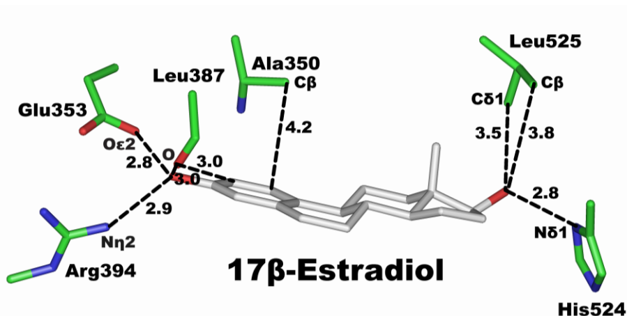
Figure 7. Structure of ER \alpha with 17 \beta -estradiol [34, 117].
