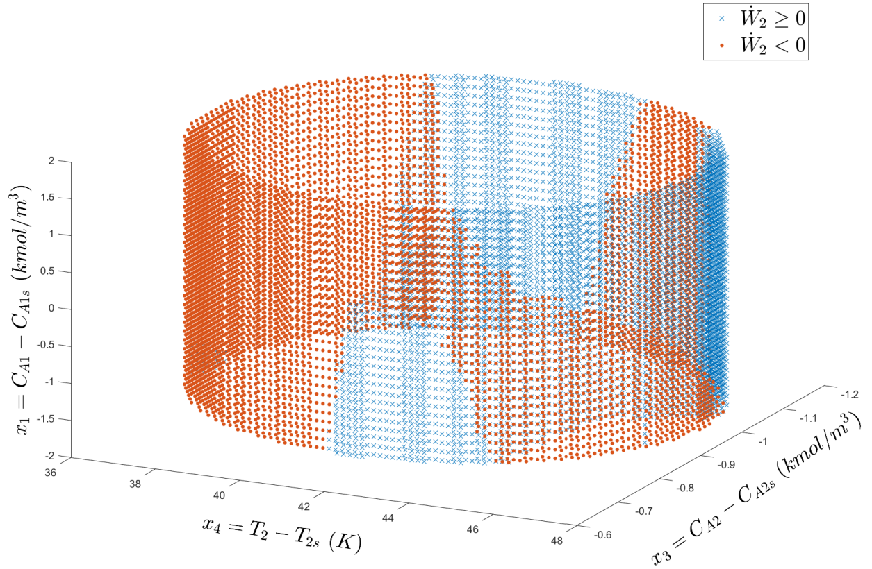
Figure 7.3: Discretized points (x_3, x_4) near CSTR-2's unsafe region \mathcal{D}_2 in state-space showing the negativity and non-negativity of \dot{W}_2 under the CLBF-based Sontag control law with respect to different values of x_1 discretized from CSTR-1's safe operating region \mathcal{U}_{\rho_1} .
