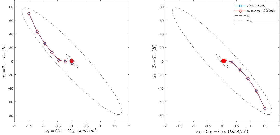
Figure 4.8: Closed-loop trajectories of true states the two-CSTR process operated under the decentralized LMPC system when geometric attacks are added on the temperature sensor T_1 of the first CSTR at t = 0.30 hr and detected by the 2-class FNN detector at t = 0.35 hr, after which all sensors are switched to their secure back-up sensors and the true process states are maintained within the ultimate bounded region \Omega_{\rho_s} around the operating steady-state.
