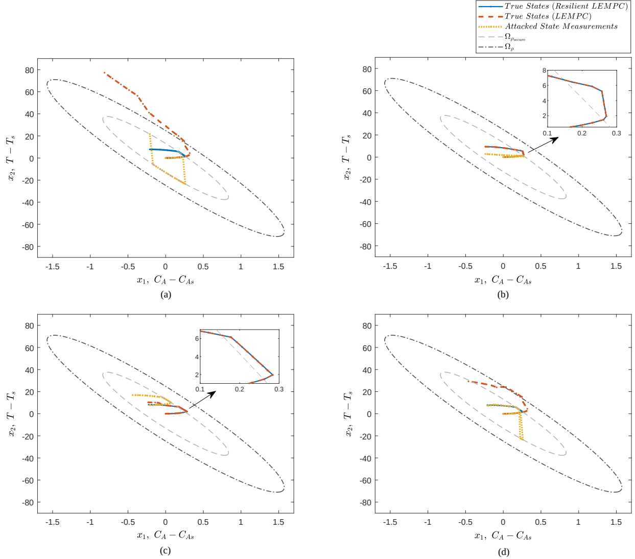
Figure 3.5: State-space plot showing the evolution of true process states and attacked state measurements (yellow trajectories) over one material constraint period under LEMPC (red trajectories) and under resilient LEMPC (blue trajectories) when (a) min-max, (b) geometric, (c) replay, and (d) surge attacks, are targeting the temperature sensor, where the dash-dotted ellipse is the stability region \Omega_\rho and the dashed ellipse is \Omega_{\rho_{secure}} .
