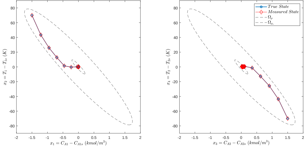
Figure 4.6: Closed-loop trajectories of true states the two-CSTR process operated under the decentralized LMPC system when min-max attacks are added on the temperature sensor T_2 of the second CSTR at t = 0.30 hr , and detected by the 2-class FNN detector at t = 0.30 hr .
