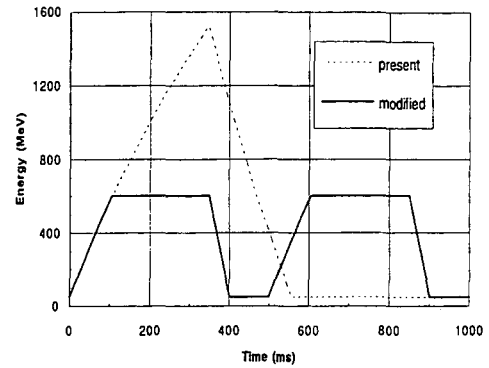
Figure 3. Ramping schedule for the ALS booster. The dotted line is the booster schedule for normal operation.
