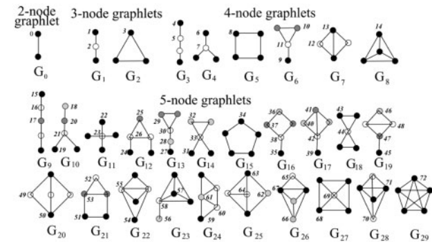
Fig. 1. Graphlets with 2–5 nodes, G_0, G_1, \dots, G_{29} . The automorphism orbits are numbered from 0 to 72, and the nodes belonging to the same orbit are of the same shade within a graphlet (Pržulj, 2007)
