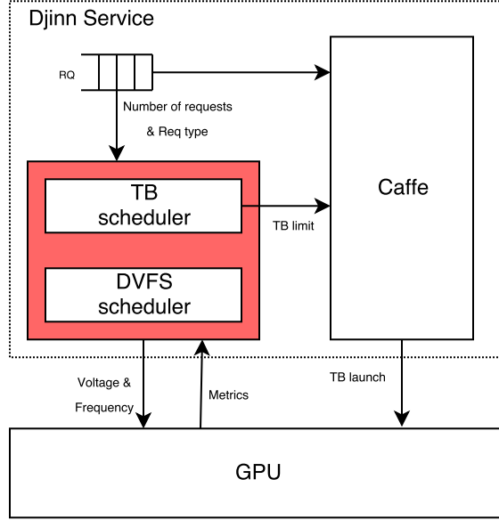
Figure 4.1: Runtime Framework in Djinn
