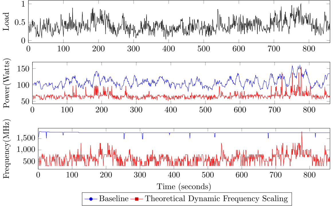
Figure 4.2: Power and Frequency Results of Titan X while running a Google data center utilization trace. Baseline (Blue) shows the behavior of existing power management in modern GPUs. The red line shows the potential for power savings by latency-aware dynamic frequency scaling.
