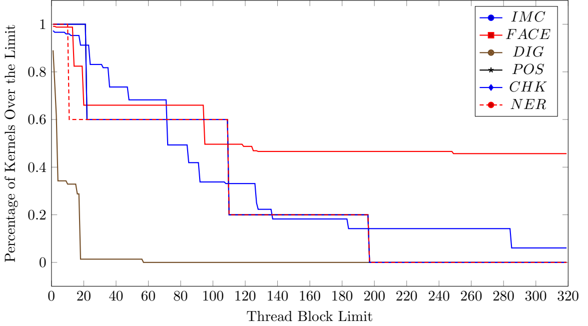
Figure 3.5: Percentage of Kernels that are greater than the limit. This chart shows that a large percentage of kernels do not utilize all GPU resources
