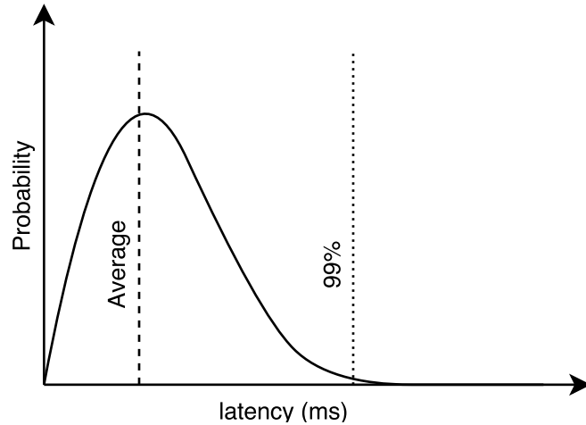
Figure 2.4: Example of Latency Distribution in Data Centers. Guaranteed latency is under the 99 percentile, but average latency is much lower than the tail. This gives some slack to slow down requests and save energy.
