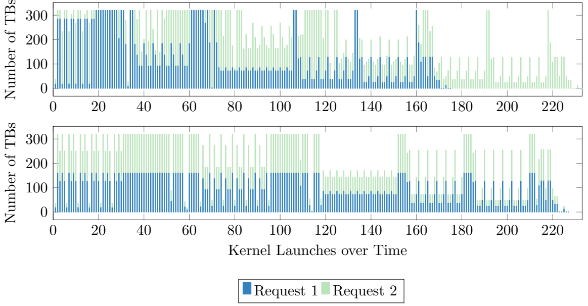
Figure 3.3: Simple example of the effect of thread block scaling with two concurrent requests of IMC workload. The top figure shows how request 1 consumes most of the resources, delaying request 2. The bottom figure shows how limiting the number of thread blocks by half can reduce the overall time of finishing both requests.
