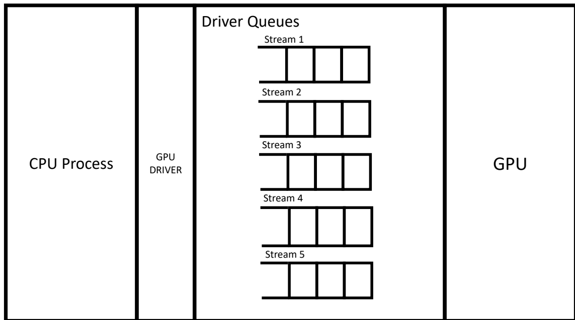
Figure 2.2: How the driver handles kernel calls from a CPU Process. Kernels from different streams are able to execute concurrently, however kernels from the same stream are pushed into Driver Queues and executed sequentially
