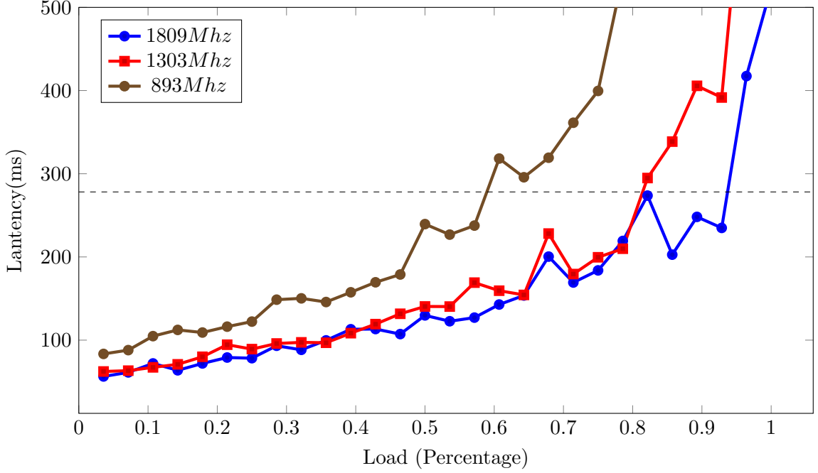
Figure 3.1: Impact of frequency and server load on tail latency. At light loads, lower frequencies are able to maintain QoS.
