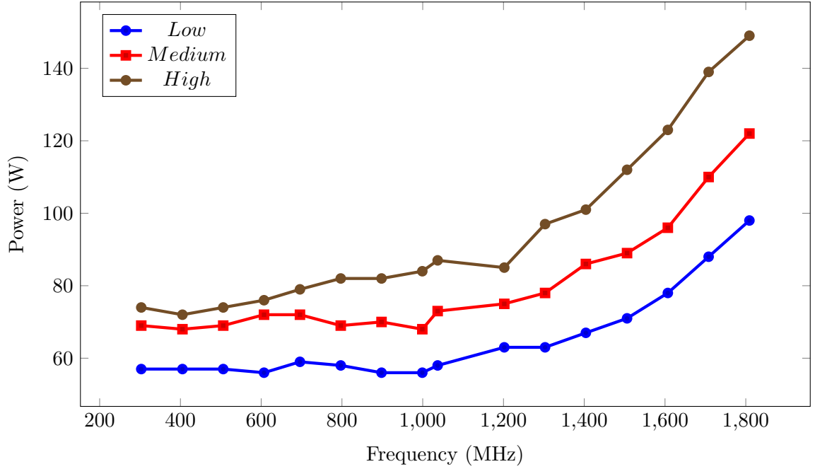
Figure 3.2: Power Usage of Low, Medium, High loads at varying frequencies. Power savings is limited at lower frequencies.
