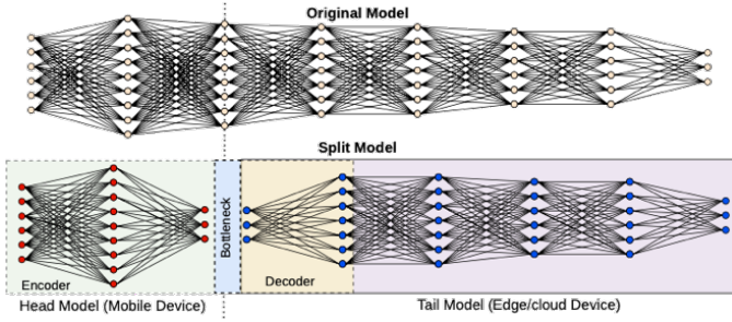
Fig. 1: Supervised Compression for Split Computing [1].
