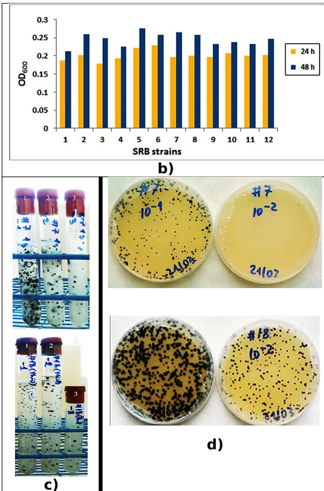
Fig.1. Identification of SRB in the environmental samples collected in Georgia a) Cultivation in liquid medium (vials with diluted samples: #6; #7; #16; #12); b) Optical density ( OD_{600} ) of bacterial cultures cultivated in liquid medium-87: 1. D. vulgaris Hildenborough, 2. D. africanus PCS, 3. DvRCH1/GE6, 4. D/PA35E4/GE7, 5. DvH/GE7/1, 6. DvH/GE15, 7. D/LZK1/GE16, 8. DvH/GE16/1, 9. D/JG1/GE18, 10. D/GE19, 11. D/LZK1/GE20, 12. D/LZK1/GE20/1; c) Bacterial colonies in soft agar medium (samples: #7 and #18); d) Bacterial colonies on solid medium (samples: #7 and #18).
