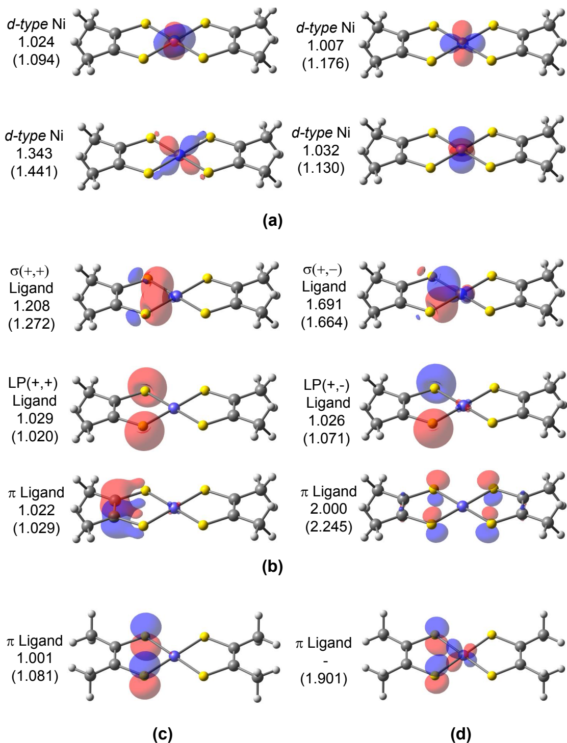
Figure 4: Valence LOs of the [\text{Ni}(\text{S}_2\text{C}_2\text{Me}_2)_2]^0 system with IAO-AutoSAD and TFVC (in parenthesis) FOLI values. d -type orbitals on Ni (a), ligand's \sigma , lone pair (LP) and \pi orbitals (b). Last localized ligand \pi orbital for [\text{Ni}(\text{S}_2\text{C}_2\text{Me}_2)_2]^{2-} (c). Last localized ligand \pi orbital from the beta density of [\text{Ni}(\text{S}_2\text{C}_2\text{Me}_2)_2]^- using TFVC (d). The isosurface value is 0.075 a.u.
