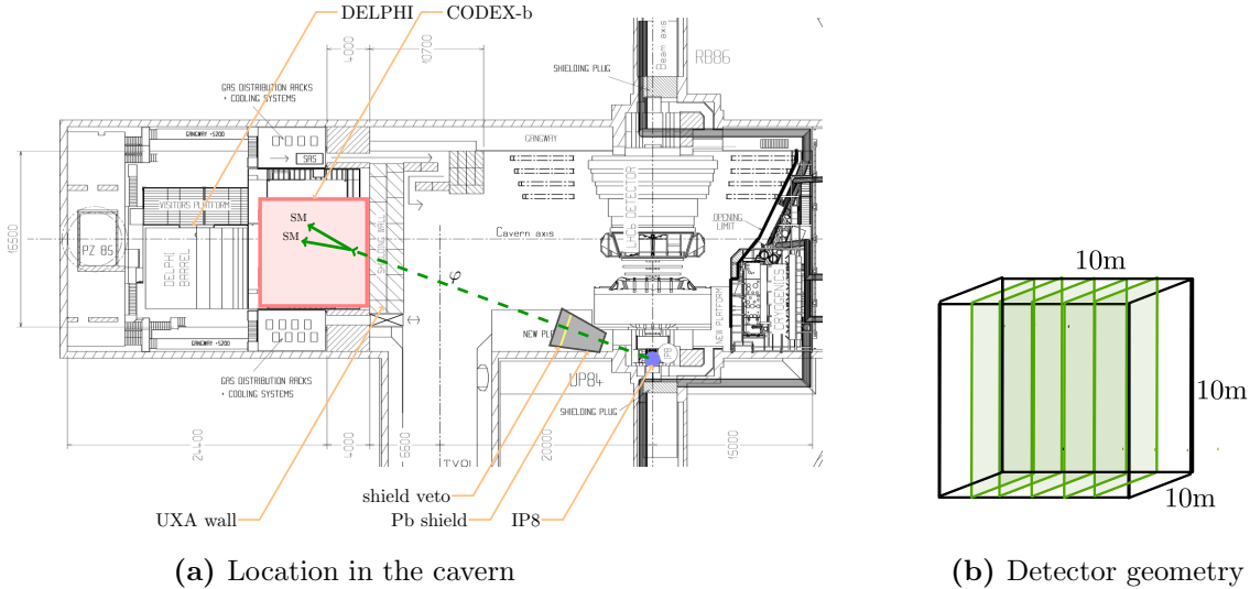
FIG. 3: Left: Layout of the LHCb experimental cavern UX85 at point 8 of the LHC [9], overlaid with the CODEX-b volume, as reproduced from Ref. [8]. Right: Schematic representation of the proposed detector geometry.
