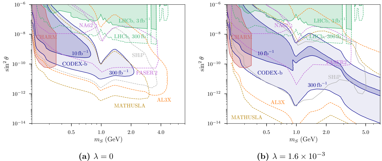
FIG. 9: Reach of CODEX-b as a function of \sin^2 \theta , for two representative values of \lambda . The MATHUSLA reach is shown for its 200m \times 200m configuration for 3 ab ^{-1} ; for AL3X 100 fb ^{-1} of integrated luminosity was assumed.
