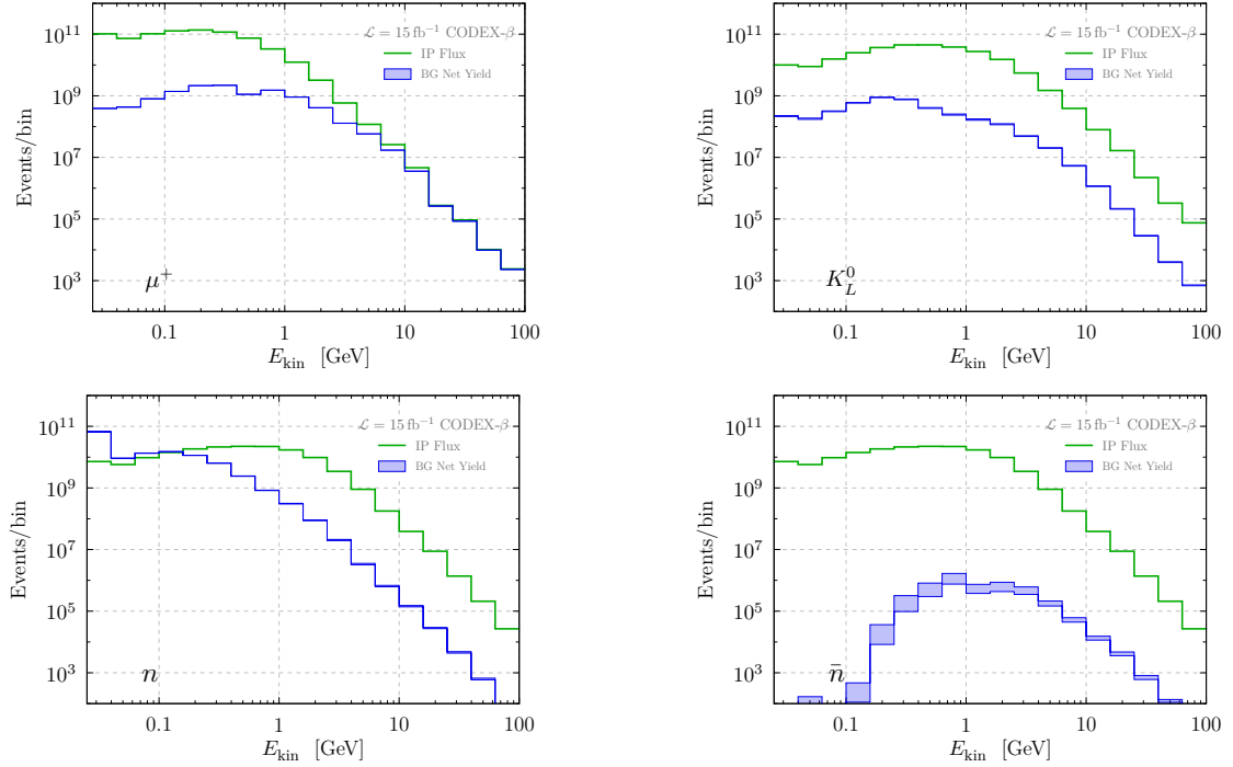
FIG. 28: Background fluxes per kinetic energy bin, comparing primary IP fluxes (green) with the background flux (blue) in the CODEX- \beta acceptance after passage through the 3 m UXA concrete wall.
