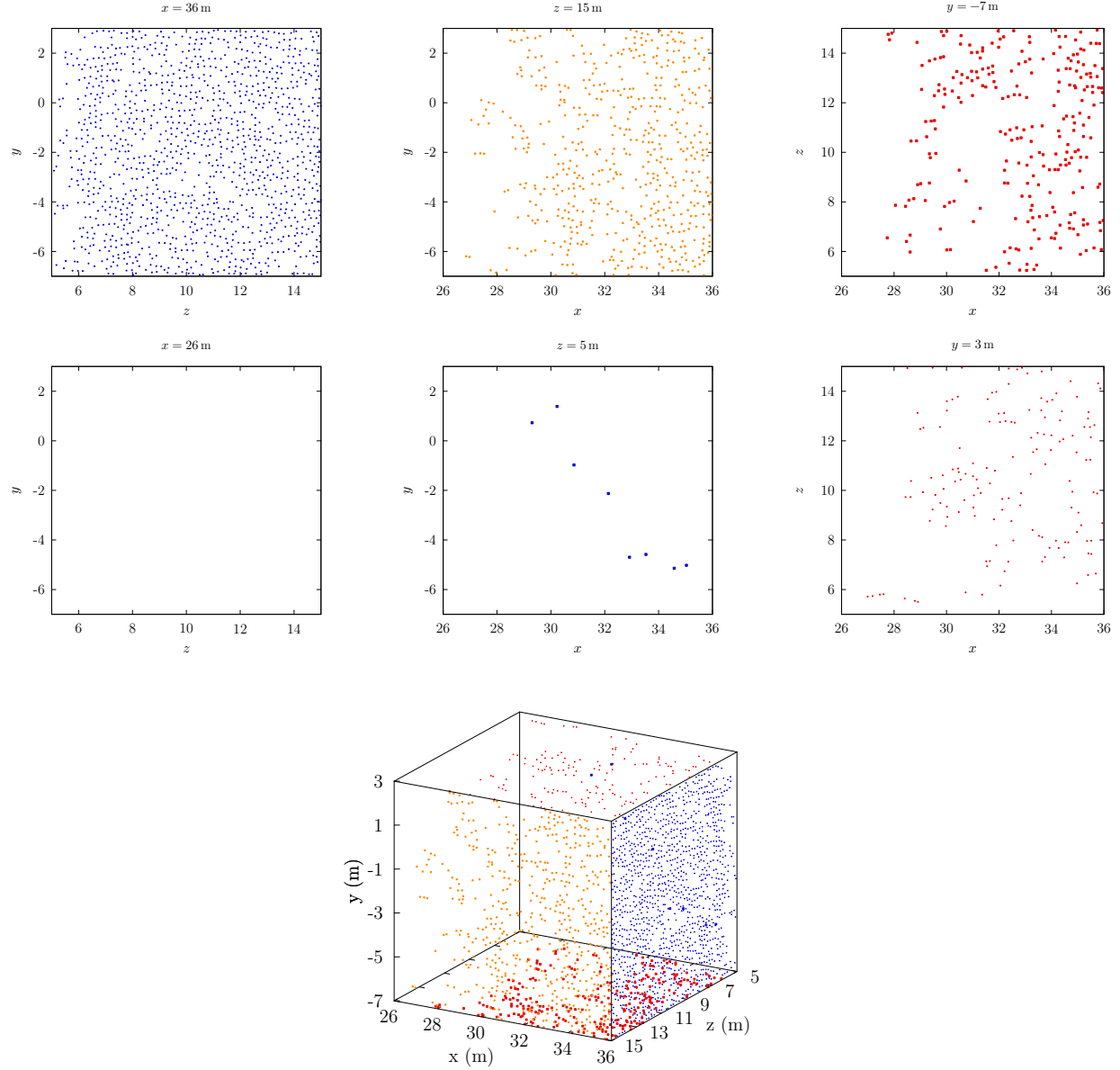
FIG. 30: Above: Scatter plot of hits on the faces of the box for 496 decays inside the box, from a h \rightarrow A'A' \rightarrow 4\tau benchmark. (From left to right) Top row: x = 36 m, z = 15 m, y = -7 m. Bottom row: x = 26 m, z = 5 m, y = 3 m. Below: The corresponding scatter plots shown in projection on the surfaces of the detector, with the same color scheme.
