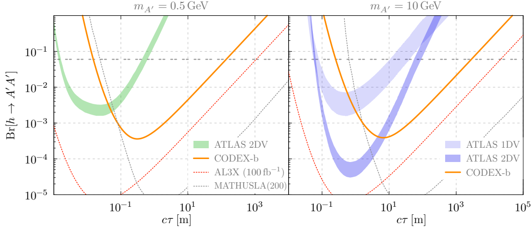
FIG. 7: Reach for h \rightarrow A'A' , as computed in Ref. [8]. Shaded bands refer to the optimistic and conservative estimates of the ATLAS sensitivity [46, 47] for 3 \text{ ab}^{-1} , as explained in the text. The horizontal dashed line represents the estimated HL-LHC limit on the invisible branching fraction of the Higgs [48]. The MATHUSLA reach is shown for its 200\text{m} \times 200\text{m} configuration with 3 \text{ ab}^{-1} ; for AL3X 100 \text{ fb}^{-1} of integrated luminosity was assumed.
