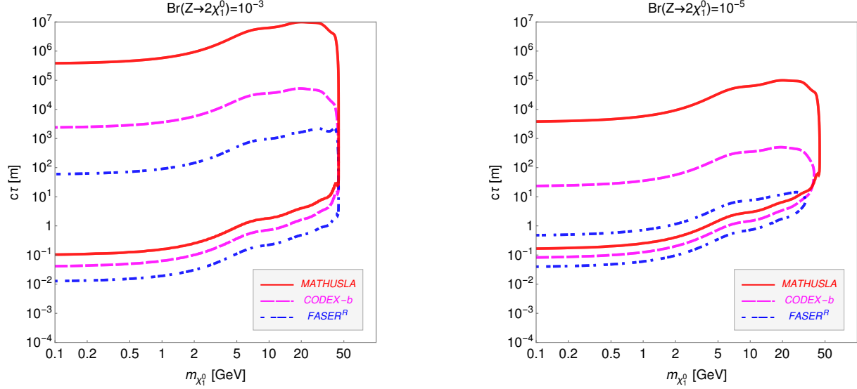
FIG. 16: Projected sensitivity of CODEX-b for light neutralinos with R-parity violating coupling, as produced in Z decays, reproduced from Ref. [83] with permission of the authors. Also shown are projections for the 200m×200m MATHUSLA configuration and FASER R , the 1m radius configuration (referred to as FASER2 elsewhere in this document).
