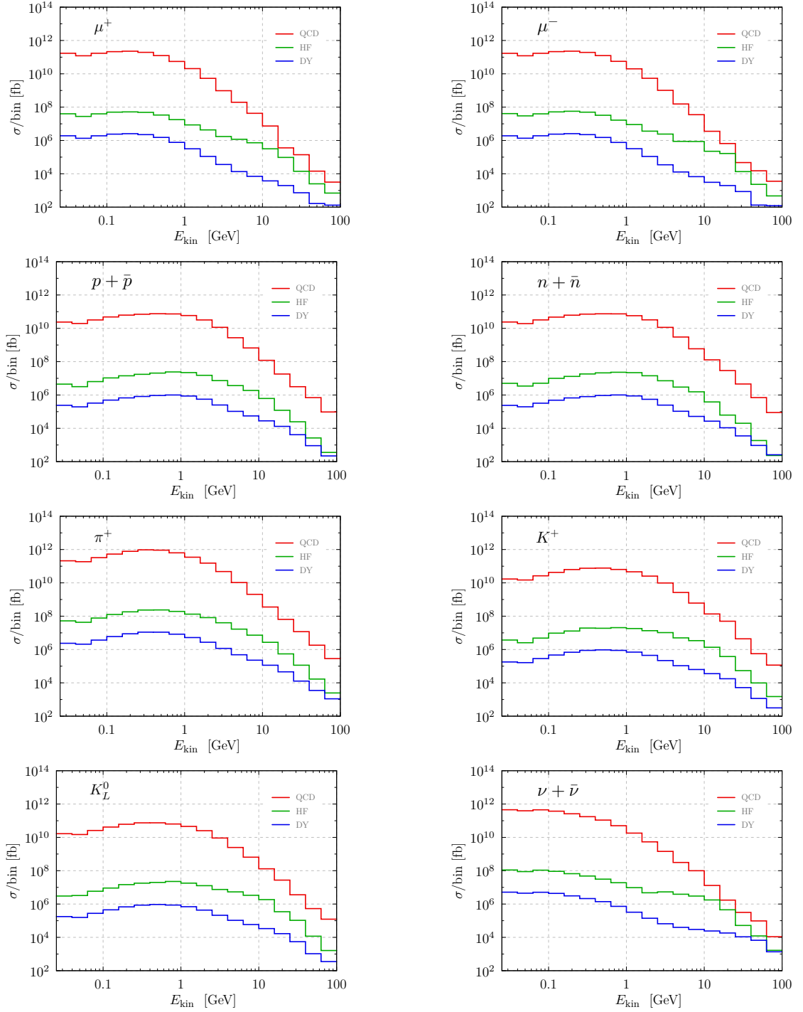
FIG. 22: IP production cross-section per kinetic energy bin, for minimum bias (QCD), Heavy Flavor (HF), and Drell-Yan (DY) production channels.
