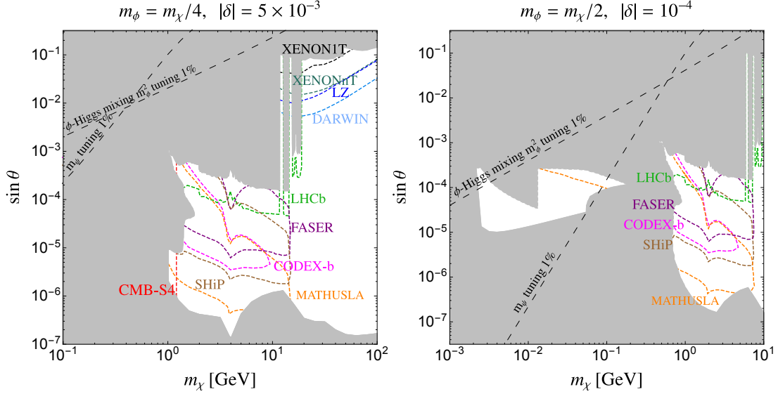
FIG. 20: Projected sensitivity to the coannihilation dark matter benchmark, reproduced from Ref. [133] with permission of the authors. The projections are effectively the same as those in Fig. 9a. In every point of the plot, \Delta is fixed to reproduce the observed relic density. Left: The remaining parameters are set as y = e^{i\pi/4} , m_\phi = m_\chi/4 and \delta = 5 \times 10^{-3} e^{i\pi/4} , with \delta \equiv \delta m/m_\chi . Right: The remaining parameters are set instead as y = e^{i\pi/4} , m_\phi = m_\chi/2 and \delta = 10^{-4} e^{i\pi/4} . MATHUSLA sensitivity is shown for the 200m \times 200m configuration, while FASER sensitivity is shown for the 1m radius configuration, now referred to as FASER2.
