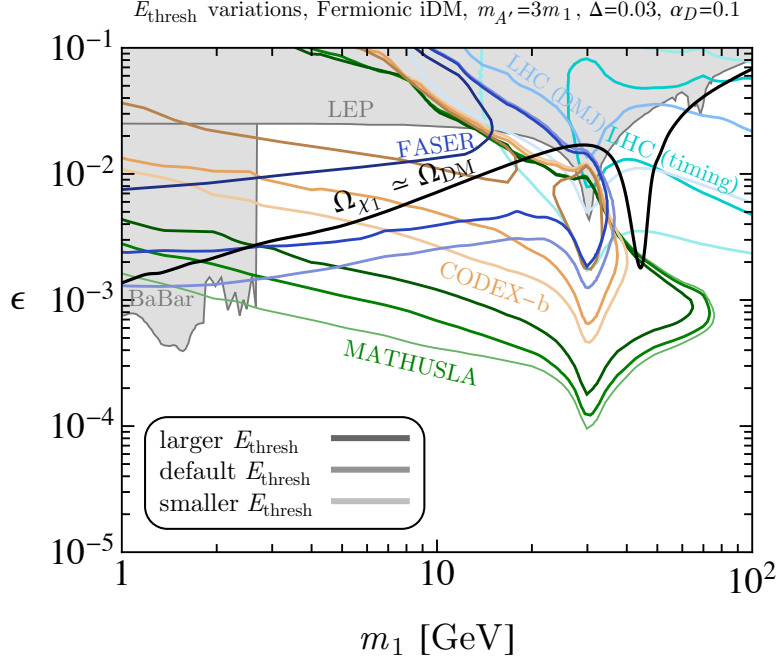
FIG. 18: Sensitivity estimates for the inelastic dark matter benchmark, reproduced from Ref. [128] with permission of the authors. The black line indicates the line on which the correct dark matter relic density is predicted by the model. Darker/lighter shades correspond to larger/smaller minimum energy thresholds for the decay products of \chi_2 , with CODEX-b shown in orange shades. For CODEX-b and MATHUSLA (200m×200m), the minimum energy is taken to be 1200, 600, or 300 MeV per track. For FASER2 (1m radius), the total visible energy deposition is taken to be greater than 200, 100, or 50 GeV. For a displaced muon-jet search at ATLAS/CMS and a timing analysis at CMS with a conventional monojet trigger, the minimum required transverse lepton momentum is 10, 5, or 2.5 GeV and 6, 3, or 1.5 GeV, respectively.
