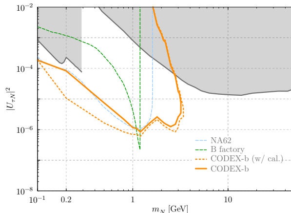
FIG. 35: Projected sensitivity of CODEX-b to Dirac heavy neutral leptons for U_{\tau N} \gg U_{eN}, U_{\mu N} for a tracking detector only (solid) compared to an optimistic case (dashed) with a calorimeter capable of reconstructing the N \rightarrow \nu \pi^0 final state, assuming the background differential flux of single \pi^0 's is negligible or reducible.
