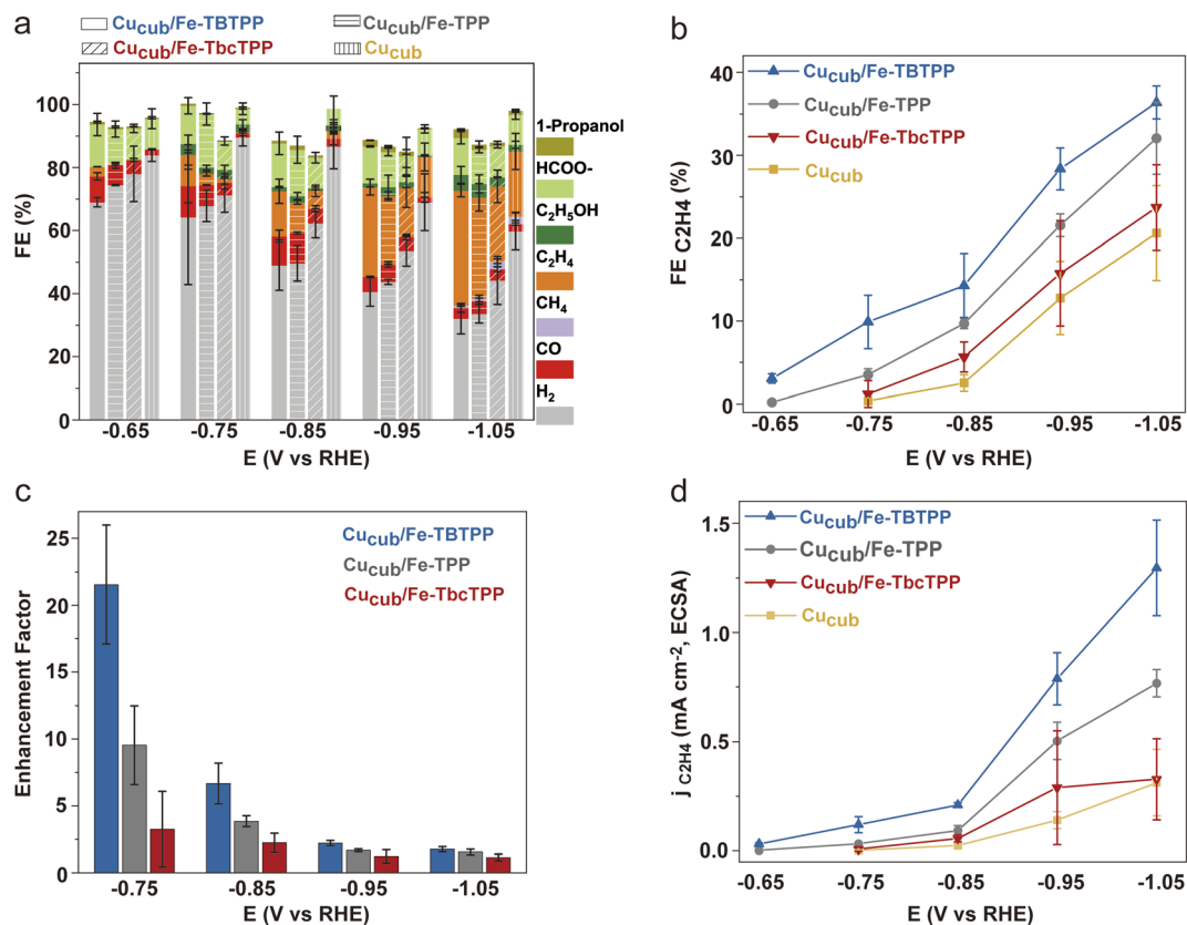
Fig. 4 (a) Total FEs and (b) FE_{C_2H_4} for Cu_{cub}/Fe-TBTTP , Cu_{cub}/Fe-TPP , Cu_{cub}/Fe-TbcTPP and Cu_{cub} as a function of potential; (c) C_2H_4 product enhancement factor of the Cu_{cub}/Fe-Por compared to the pristine Cu_{cub} (enhancement factor = (FE_{C_2H_4} \text{ of } Cu_{cub}/Fe-Por)/(FE_{C_2H_4} \text{ of } Cu_{cub}) as a function of potential; (d) j_{C_2H_4}/ECSA for Cu_{cub}/Fe-TBTTP , Cu_{cub}/Fe-TPP , Cu_{cub}/Fe-TbcTPP and Cu_{cub} as a function of potential. The electrodes for these experiments were prepared by loading 3.12 \times 10^2 \text{ nmol cm}^{-2} of Cu_{cub} and 8 \text{ nmol cm}^{-2} of the Fe-Por onto glassy carbon electrodes. The reported values are an average of three independent experiments with error bars indicating the standard deviations.
