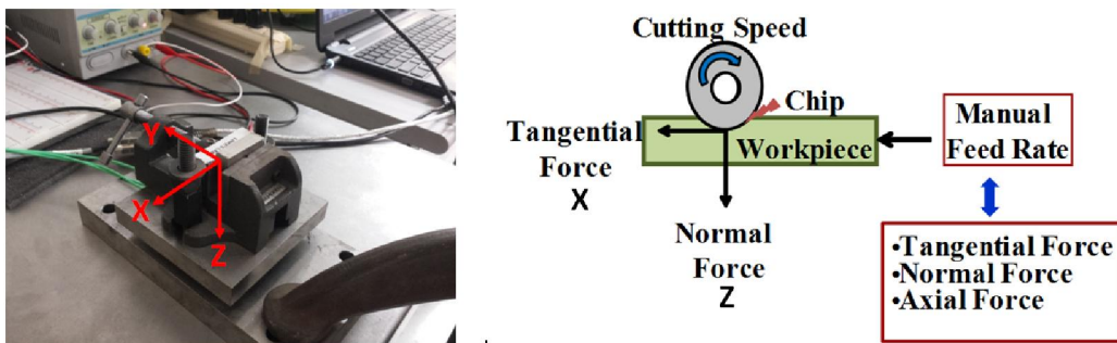
Figure 2: An image of a grinding sample (left) and a figure showing the force data collection module (right). Forces in three directions were measured, tangential (x-axis), normal (z-axis) and axial (y-axis).
