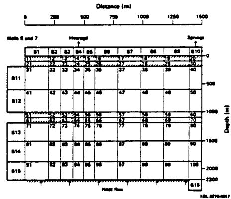
Figure 3: Simplified reservoir model and mesh used in the study of the natural state.
