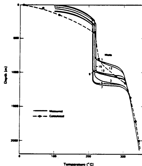
Figure 8: Comparison between observed and calculated temperature profiles in the old wellfield.
