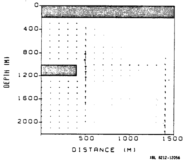
Figure 10: Steady-state flow field in the natural state (best case).
