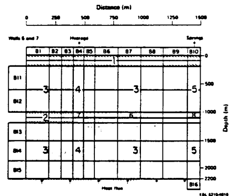
Figure 4: Different reservoir zones used in the best model.
