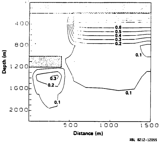
Figure 9: Steady-state vapor saturations in the natural state.
