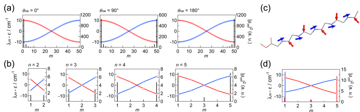
Figure 8. Excitonic properties calculated for the fully extended structure with (\phi, \psi) = (\pm 180^\circ, \pm 180^\circ) .
