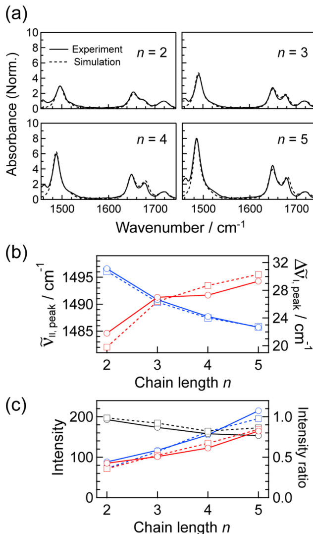
Figure 2. (a) Measured FT IR spectra (solid) of the Ac-(Deg) n -OtBu ( n = 2–5) peptides in CDCl 3 . Each spectrum was normalized by the peak absorbance of the ester C=O band at ~1718 cm -1 after subtracting the solvent background spectrum. Simulated linear IR spectra (dashed) are superimposed on the measured spectra after following the same normalization procedure. (b) Frequency separation between the two amide-I bands ( \Delta \tilde{\nu}_{I, \text{peak}} , red) and the peak frequency of the amide-II band ( \tilde{\nu}_{II, \text{peak}} , blue) in the measured (circles) and simulated (squares) linear spectra. (c) Integrated area intensity of the amide-I (red) and II (blue) bands, and their ratio I_I/I_{II} (black) in the measured (circles) and simulated (squares) linear spectra. The solid and dashed lines through the markers in the panels (b) and (c) are guides for eyes.
