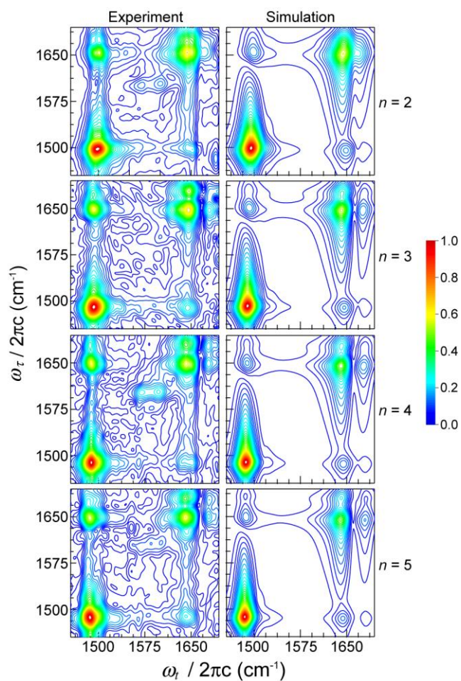
Figure 6. Measured (left column) and simulated (right column) absolute magnitude 2D IR amide-I/II spectra of Ac-(Deg) n -OtBu ( n = 2-5 ) in CDCl 3 with the NR pulse sequence and \langle Y, Y, Z, Z \rangle polarization configuration. See the captions of Figure 5 for other details.
