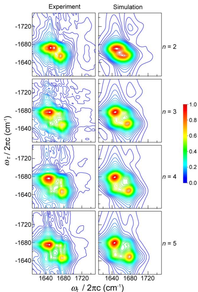
Figure 3. Measured (left column) and simulated (right column) absolute magnitude 2D IR amide-I spectra of Ac-(Deg) n -OrBu ( n = 2\text{--}5 ) in CDCl 3 with the R pulse sequence and \langle \pi/4, -\pi/4, Y, Z \rangle polarization configuration. Each spectrum is normalized by the maximum amplitude, and plotted with 40 equally-spaced contour lines from 0 to 1.
