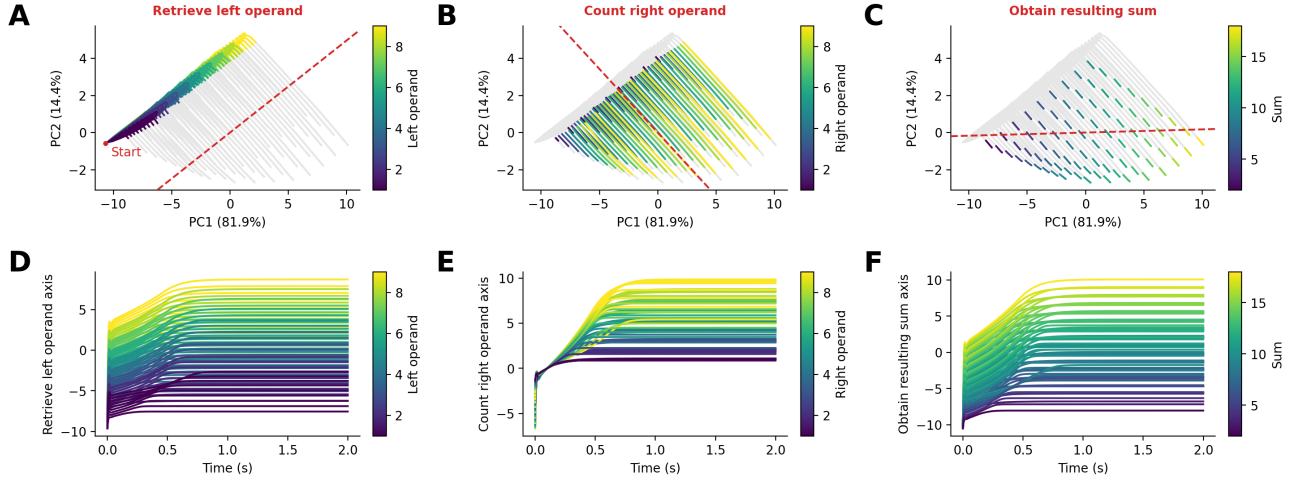
Figure 2: RNNs implement counting as a sequential drift along two number-line representations. A-C. Principal component (PC) analysis of population neural activity across all single-digit additions, projected onto the first two PCs (which together explain 96.3% of variance). Trajectories are colored by left operand (A), right operand (B), and resulting sum (C), highlighting three successive phases of computation: rapid retrieval of the left operand within the first 100 ms (A), slow iterative counting of the right operand until the working-memory output stabilizes (B), and settling onto a two-dimensional manifold encoding the final sum (C). D-F. Projections of the same trajectories onto the decoded linear subspaces (red axes in A-C) that best decode the left operand (D), right operand (E, after subtracting for each trial the PC values at 100 ms to remove the left-operand offset), and resulting sum (F). Subspace projections correlate with the left operand early in the trial (D, before 100 ms), and with the right operand and resulting sum after counting is complete (E-F, once the output has stabilized), confirming that the two principal components reflect distinct computational roles during initialization and counting.
