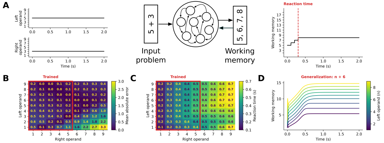
Figure 1: RNNs generalize a counting strategy to solve addition. A. Task and RNN model schematic. Operands are provided as constant inputs throughout the trial (left). They are processed by an RNN with feedback (middle), producing a scalar readout that implements counting (right). Reaction time is defined as the first time when working memory stays within 0.5 of its final value for the remainder of the trial. B-C. Model's mean absolute error (B) and reaction time (C) when tested on all single-digit additions with left and right operand between 1 and 9. D. Example working-memory trajectories for n + 6 additions with n between 1 and 9, all unseen during training. Each trajectory shows a smooth, continuous progression from the starting value n toward the sum n + 6 , followed by stabilization at the correct answer, demonstrating that the learned drift dynamics extend to longer counts without discrete jumps.
