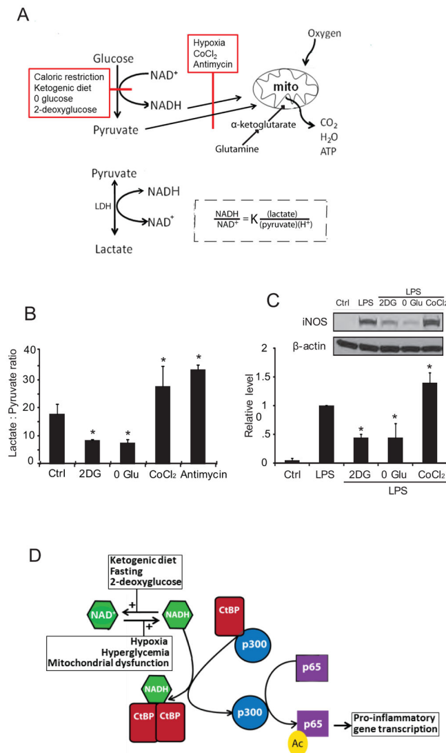
Figure 5. NADH and CtBP mediate coupling between glucose metabolism and gene transcription (A) Factors that slow glucose flux through glycolysis, such as reduced glucose availability or glycolytic inhibitors, reduce NADH levels and thereby reduce NADH:NAD + ratio, whereas factors that slow oxidative metabolism, such as hypoxia and mitochondrial inhibitors, have the opposite effect. Lactate dehydrogenase (LDH) maintains the lactate:pyruvate ratio in equilibrium with the cytosolic NADH:NAD + ratio. In the experiments shown, glutamine provided α-ketoglutarate to fuel mitochondrial ATP production in the absence of glycolysis. (B) The lactate:pyruvate ratio provides an index of the cytosolic NADH:NAD + ratio in cells treated with glycolytic inhibition (2DG, 1 mM 2-deoxyglucose; 0 Glu, glucose-free medium) or mitochondrial inhibitors (CoCl 2 , 200 μM cobalt chloride; antimycin, 1 μM antimycin A). n = 4; *p < 0.05 v. control. (C) LPS-induced iNOS expression was suppressed in RAW267.4 cells treated with 1 mM 2DG or glucose-free medium, and was increased in cells treated with the CoCl 2 . n = 4; * p < 0.05 v. control. Error bars show s.e.m. (D) CtBP normally binds and inhibits p300 acetylase. NADH promotes CtBP dimerization and resultant release of p300 from CtBP. Unbound p300 acetylates the p65 subunit of NF-κB to
