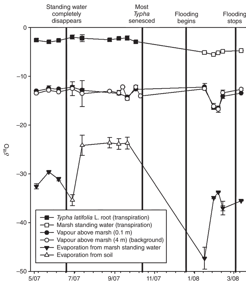
Figure 6. The isotopic composition of endmembers used for distinguishing between evaporation ( E ) and transpiration ( T ) in canopy vapour (collected at 0.1 m height above marsh water/soil surface). The endmembers were background vapour collected 4 m above the marsh water/soil surface, E from standing water and soil, and T (assumed to be similar to Typha latifolia L. root water in 2007, and marsh standing water in 2008).
