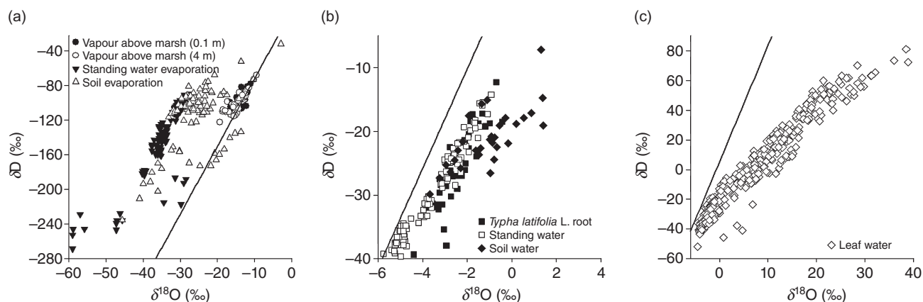
Figure 2. The \delta^{18}\text{O} – \delta\text{D} relationships of (a) within-canopy vapour collected 0.1 above marsh standing water and above-canopy vapor collected 4 m above marsh standing water and modelled evaporation ( E ) from marsh standing water and soil water (b) Typha latifolia L. root water and marsh standing water (c) leaf waters. In all plots, the solid line indicates the California meteoric water line as determined by Kendall & Coplen (2001). Note that figure axes vary in scale.
