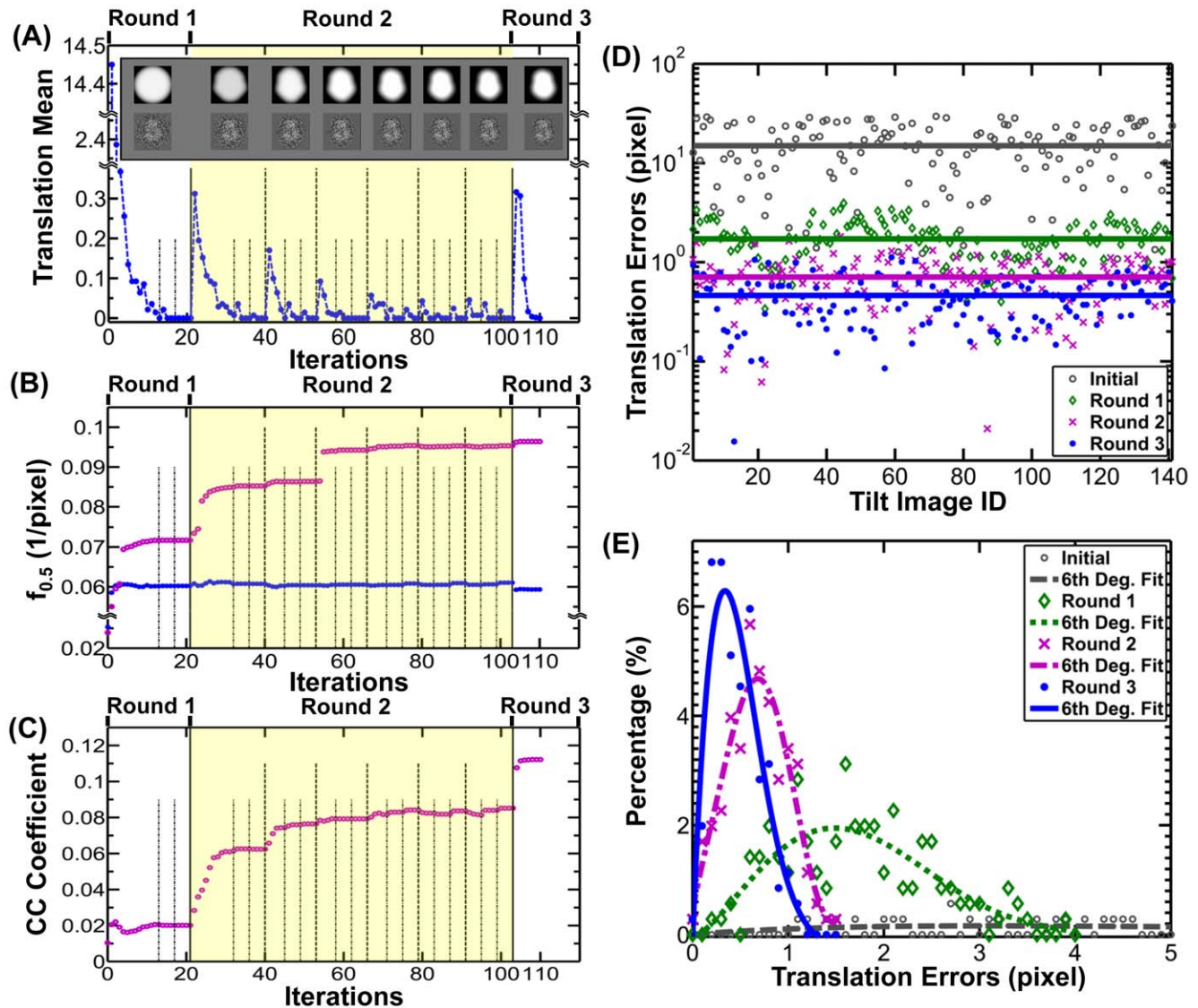
Figure 3. Monitoring the convergence of the iterations. Four parameters were used to monitor the progress of the iterations, translation mean, f_{0.5} values, cross-correlation coefficients (CC C), and translation errors. (A) The translation mean was the sum of the translation distances of all the images divided by the total number of images. The result showed that the translation means approached zero gradually. During the iteration, various sizes and shapes of masks were used and displayed. (B) Two types of f_{0.5} values were used to monitor the progress. One type (blue points), called intra- f_{0.5} , was calculated based on the iterated tilt images during the iteration and used to monitor the progress of the iterations. The result showed the intra- f_{0.5} values quickly improved in the first several iterations, but had no significant improvement afterward. Another type (purple circles) was a conventional f_{0.5} value that was calculated based on the iterated 3D reconstruction and the object. The result showed that the f_{0.5} values gradually improved through the iterations. (C) The CC C between each iteration 3D reconstruction and the object was computed, which also showed that the quality of reconstructions was gradually improved. (D) The distribution of the translation errors and (E) the histogram of the translation errors were used to analyze the translation parameters determined in each round. In the simulated raw images, the translation errors were evenly distributed with a mean of 14.96 pixels (gray line). After the first round, the translation errors were quickly reduced to a mean of 1.72 pixels with a peak population at 1.48 pixels (blue line). After the second round, the errors continued to be reduced to a mean of 0.71 pixels with a peak at 0.68 pixels (purple line). The errors were further minimized to a mean of 0.46 pixels with a peak at 0.34 pixels after the third round (blue line). doi:10.1371/journal.pone.0030249.g003
