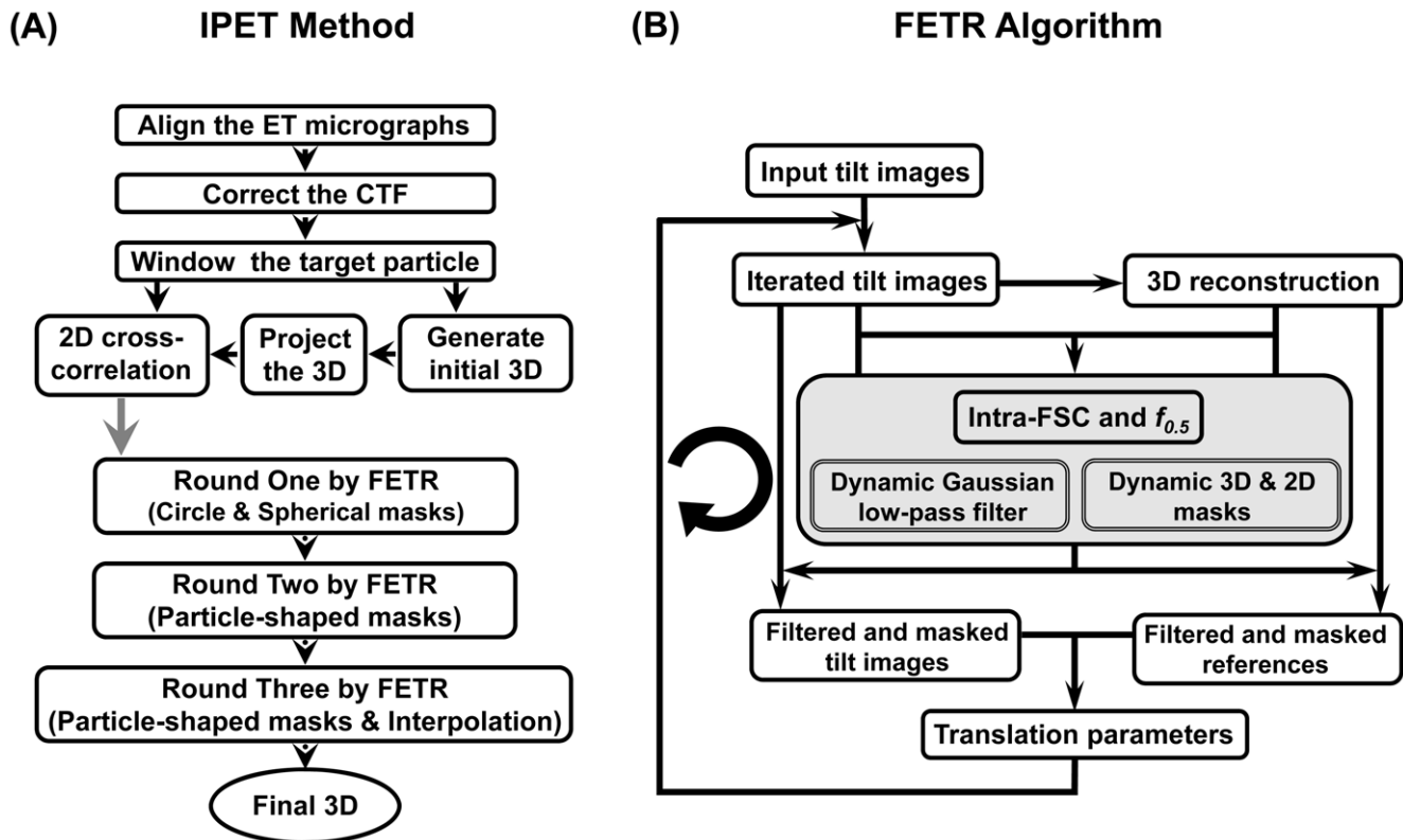
Figure 2. Flow diagram of individual-particle electron tomography (IPET) method and focused electron tomography reconstruction (FETR) algorithm. (A) The IPET method contains two phases: the electron tomography (ET) data collection with image preprocessing, and a focused electron tomography reconstruction (FETR) algorithm. In the first phase, the single-instance of particle was imaged by ET. The contrast transfer function (CTF) of the whole-micrograph-size tilt images was determined, and then corrected after tilt images were aligned. The small images containing only a targeted particle were selected and windowed from each of tilt whole-micrograph, and then directly back-projected into 3D as the initial/starting model for refinement. The 3D reconstruction refinement procedure contains three rounds of refinement loops in the FETR algorithm. Each round was essentially the same, except different masks were applied. In the first round, a series of automatically generated circular Gaussian-edge masks was used; in the second round, the automatically generated particle-shaped masks were used and while, in the third round, the last mask in second round was used with association of an additional interpolation method during determining the translation parameters. (B) Each round of refinement loops contains the same iteration algorithm, FETR. 3D reconstruction from the previous iteration (or initial model for the first iteration) was projected, and the projections were used as references for the next iteration. Before translational parameter searching, a dynamic Gaussian low-pass filter and automatically generated mask were applied to both the references and tilt images. doi:10.1371/journal.pone.0030249.g002
