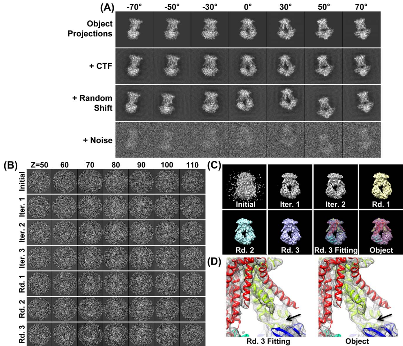
Figure 1. Simulating cryoET images and 3D reconstruction by IPET/FETR. (A) An object, a 3D density map of a single-instance protein (molybdate, portion of PDB entry 2ONK) was projected into a total of 141 tilt series of 2D images by following the simulated cryoET tilt-angles (containing both tilt-axis and tilt-angle errors in a range of \pm 0.5^{\circ} ), in which seven projections were presented (first row); to simulate contrast transfer function (CTF), CTF at a defocus of 1.5 \mu\text{m} was applied to each image and then deconvoluted (second row); to simulate the translation errors, each image was randomly shifted with a maximal radius range of 30 pixels (third row); to simulate the noise, Gaussian noise (SNR = 0.2) was added to each image (last row). These images were used as the cryoET “raw” images for 3D reconstruction. (B) By FETR, the reference-free initial model was generated by directly back-projecting the “raw” images according to the measuring tilt-angles (containing immeasurable tilt-errors). The convergence of 3D reconstruction was approached by iterations through three major rounds. Selected ET slices of the 3D reconstruction of initial model, iteration one to three, round one to three, were displayed. (C) The isosurfaces of the corresponding 3D reconstructions were also displayed after they were low-pass filtered to 8 \text{\AA} . The initial model displayed as a globular noisy blob, while the quality of reconstructions had been greatly improved after the 1–2 iterations. The reconstructions of each round contained many structural details, such as the \alpha -helices. Docking the crystal structure into the isosurface from the final reconstruction displayed a near perfect match and no distinguishing differences from the object. (D) Zoom-in views of docked final reconstruction and object displayed slight difference as indicated by the arrows. doi:10.1371/journal.pone.0030249.g001
