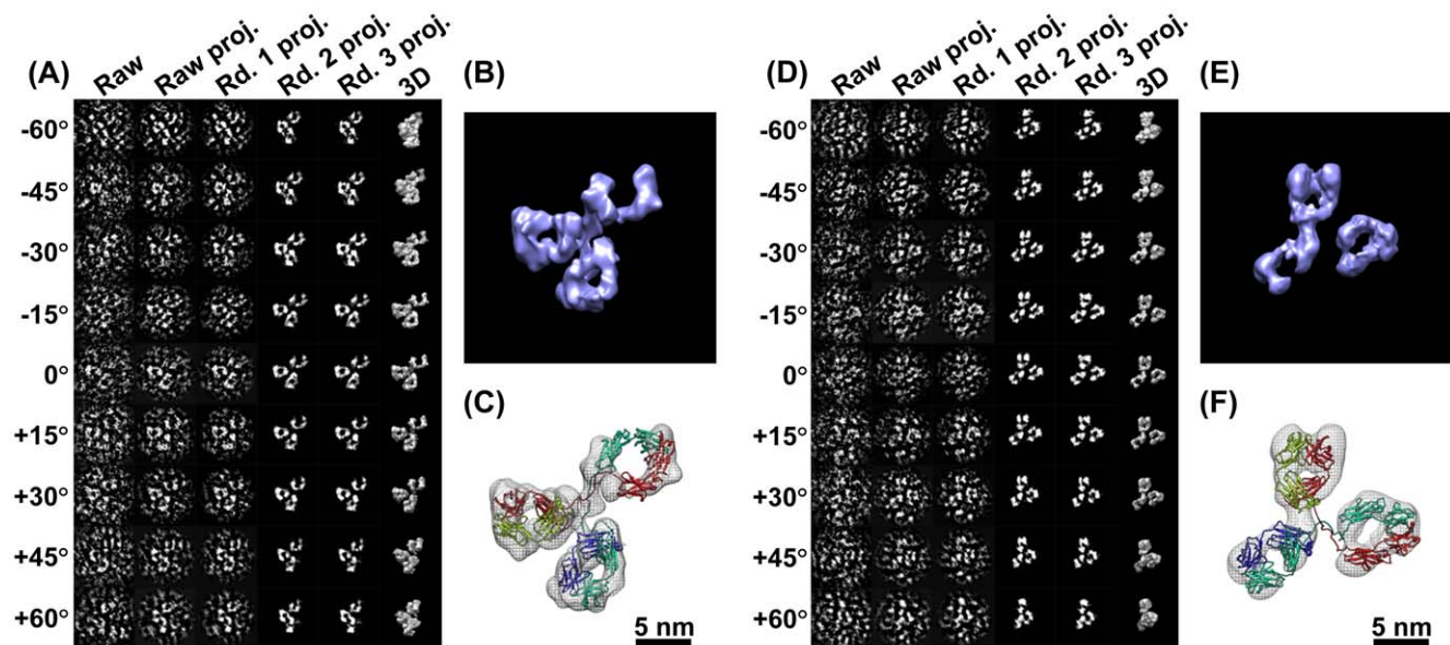
Figure 4. 3D reconstructions with negative staining of an IgG antibody by IPET. (A) A single-instance of an IgG antibody was imaged by negative staining (NS) ET. Nine tilted views of the same single IgG particle were selected from 81 tilt micrographs that were CTF corrected by TOMOCTF, and then displayed in leftmost column. By FETR algorithm, the 3D reconstruction was iterated and converged. The corresponding tilting projections of the 3D reconstruction from major iterations were displayed beside the raw images in six columns. (B) The final 3D reconstruction of a targeted individual antibody particle was displayed in a contour level that contained a volume corresponding to 160 kDa. The reconstruction displayed three ring-shaped domains that corresponding to three domain of IgG antibody. (C) Docking the crystal structure (PDB entry 1IGT) of each domain of the IgG antibody into each ring-shaped density of IgG showed a good fit. The docking was performed by a rigid-body docking option in Chimera program [79]. The loops between the domains were simply connected by Chimera. (D) Another example of the IPET method in a 3D reconstruction of another single-instance of a targeted individual IgG antibody particle. The NS-ET images of the raw images and projections of the related reconstruction were also displayed. (E) The 3D reconstruction of this antibody particle displayed a similar structural feature to the first one, such as the three domains. (F) Docking the IgG antibody crystal structure into the density map showed a good fit as well. doi:10.1371/journal.pone.0030249.g004
