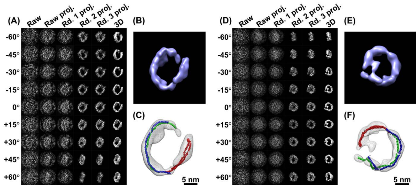
Figure 5. 3D reconstructions of a cryoET 17 nm nascent HDL particle by IPET. (A) An individual targeted nascent HDL particle embedded in vitreous ice was imaged by the cryoET technique. The tilt images of a targeted particle were windowed from the tilt series of cryoET micrographs after the CTF was corrected by TOMOCTF. Nine represented tilted views of a targeted 17 nm HDL particle were shown in leftmost column. These selected tilt images were from 81 tilt micrographs that were taken at the specified tilt angles. The other six columns in each grid showed the results of progressive refinement from certain iterations. (B) Reconstructed to 3D density map. The high-density portion corresponding to proteins, apolipoprotein A-I (apoA-I), was formed in a ring shape. (C) By docking the double-helices into the ring-shaped density, the size suggests three apoA-I molecules exist in a 17 nm HDL particle. (D) Another targeted 17 nm HDL particle was imaged and reconstructed for 3D density map. (E–F) The 3D reconstruction showed the similar structural feature to the first HDL particle, suggesting our cryoET reconstructions are consistent as reported by cryoEM observation [51].
