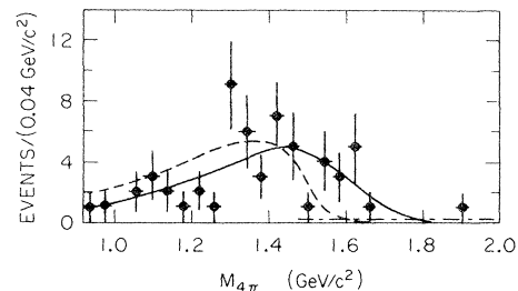
FIG. 2. 3\pi^\pm\pi^0 invariant-mass distribution for the selected decays. The curves are drawn for m_{\nu_\tau} = 0 (solid) and 250 MeV/ c^2 (dashed) and with the assumption that the four-pion state is dominated by a \rho' resonance of mass 1570 MeV/ c^2 and width 510 MeV/ c^2 . The dash-dotted line represents the hadronic background.
