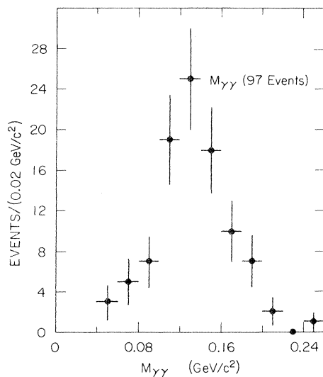
FIG. 1. \gamma\text{-}\gamma invariant-mass distribution for the 3\pi^\pm\pi^0 candidates before requiring that the confidence level for a fit to the \pi^0 hypothesis be greater than 10%.
