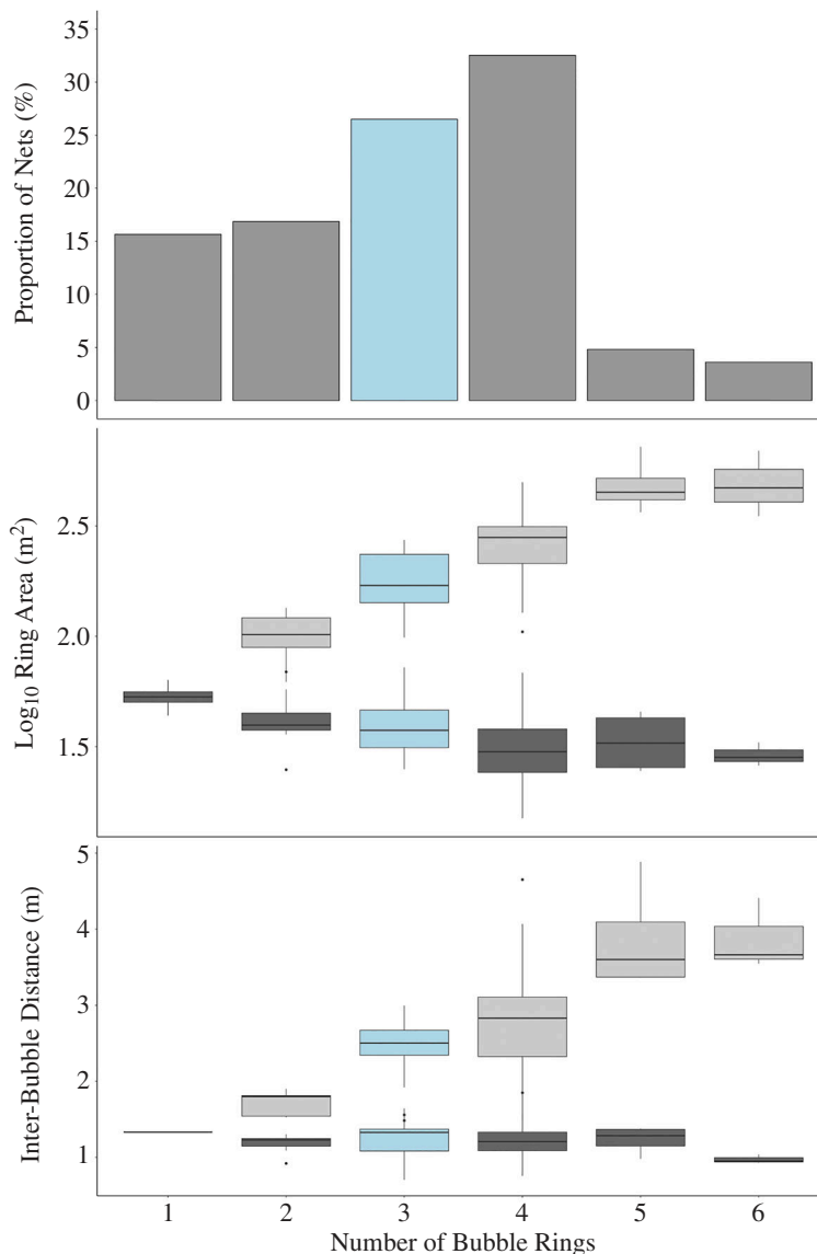
Figure 3. UAS-derived net measures relative to the number of rings in bubble-nets. Median ring count for all nets (3) highlighted in blue. (a) Proportion of nets by ring number, (b) \log_{10} area ( \text{m}^2 ) of outer (light grey) and innermost (dark grey) rings. (c) Horizontal distance (metres) between neighbouring bubbles (mesh size) in the outer (light grey) and innermost (dark grey) rings.
