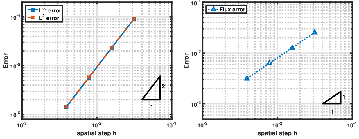
Figure 2.2: Error plot with respect to the mesh size h using Algorithm 1 on a uniform square mesh with \theta = 1 . Left : \|\mathbf{m}^h - \mathbf{m}\|_{L^\infty} and \|\mathbf{m}^h - \mathbf{m}\|_{L^2} , Right : \|\mathbf{p}^h - \mathbf{p}\|_{\mathcal{F}} .
