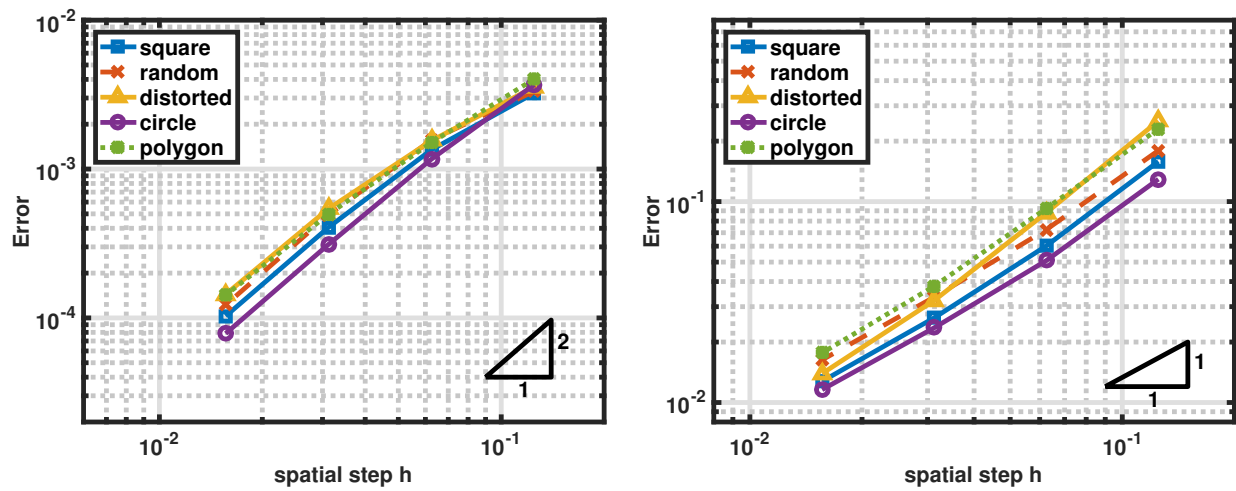
Figure 2.8: Error plot with respect to the mesh size h using Algorithm 1 and \theta = 1 with Dirichlet boundary conditions. Left : \|\mathbf{m}^h - \mathbf{m}\|_Q , Right : \|\mathbf{p}^h - \mathbf{p}\|_{\mathcal{F}} .
