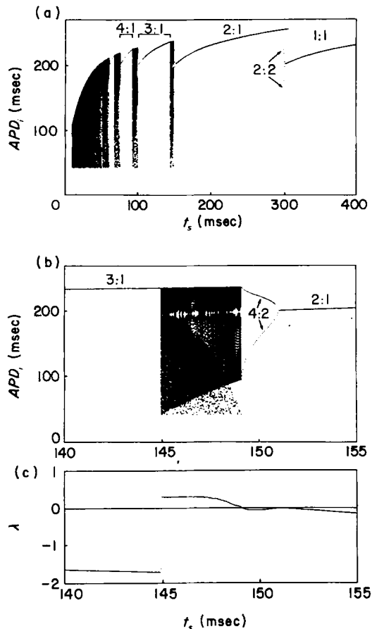
FIG. 5. (a), Bifurcation diagram ( APD_1 vs. t_s ) for t_s = 10 –400 msec. At each t_s , eqn (6) was iterated 20 000 times and the first 19 800 iterates discarded to suppress transients due to initial conditions. Increment in t_s was 1 msec. To demonstrate bistability, two initial conditions were used at each t_s ( APD_1 = 240 and 270 msec). (b), Expanded view of bifurcation diagram of (a) in range t_s = 140 –155 msec. The period-doubling of the period-1 orbit on the n = 2 branch (corresponding to the 2:1 rhythm of Fig. 1(c)) to a period-2 orbit [corresponding to the 4:2 rhythm of Fig. 1(d)] is clearly shown, as is the transition from the 4:2 rhythm to aperiodic dynamics [Figs 1(e) and 4(e)]. Increment in t_s was 0.05 msec. (c), Liapunov number ( \lambda ) calculated over the same range of t_s as displayed in (b). \lambda was calculated from eqn (7) with N = 20\,500 . The first 500 iterates were discarded to minimize the contribution to \lambda of chaotic transients seen close to the 3:1 boundary (Grebogi et al. , 1984). Computations shown in Figs 4 and 5 were carried out on an HP1000 minicomputer in double precision (approximately 15 significant decimal digits).
