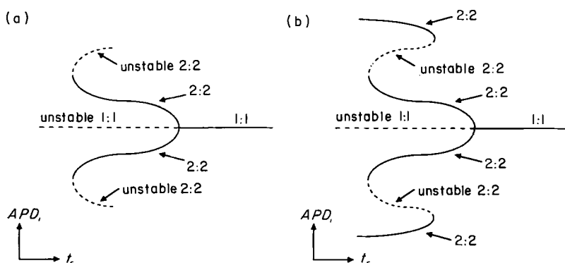
FIG. 8. Schematic bifurcation diagrams. (a), Bifurcation diagram illustrating how period-2 orbit of Fig. 4(c) (corresponding to a 2:2 rhythm) is destroyed. (b), Alternative bifurcation diagram showing how it is possible to obtain coexistence of two stable period-2 orbits (corresponding to two different 2:2 rhythms). Solid lines indicate stable orbits, dashed lines unstable orbits. Saddle-node bifurcations occur at turning points in (a) and (b). See text for further description.
