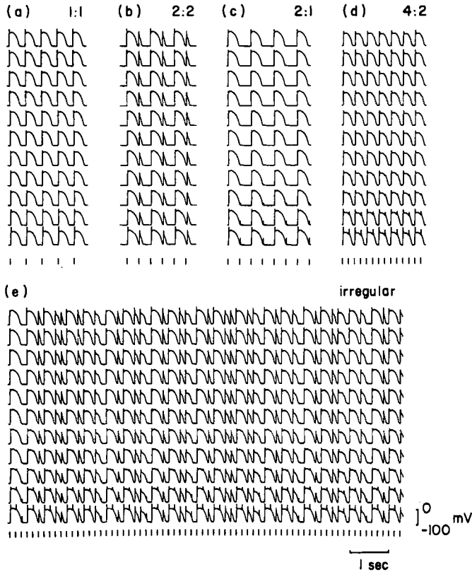
FIG. 1. Response of one-dimensional cable to periodic stimulation. (a), 1:1 rhythm, t_s = 400 msec, (b), 2:2 rhythm, t_s = 301 msec, (c), 2:1 rhythm, t_s = 290 msec, (d), 4:2 rhythm, t_s = 151 msec, (e), irregular rhythm, t_s = 143 msec. In (b), the APD in the segment 90 alternates between 62 and 249 msec, and the conduction velocity in the middle of the strand between 62 and 67 cm sec -1 . (a)–(e), Bottom to top: stimulus pulses and transmembrane potential ( V ) vs. time ( t ) in segments 1, 10, 20, ..., 90, 100 of strand. Voltage traces are displaced vertically with an offset of 125 mV. Traces in (a)–(d) taken from near end of a 10-sec simulation run, at which point the transient due to initial conditions has largely damped out. Note the small-amplitude voltage responses in (c)–(e) that decrement in amplitude with distance down the strand. Calibration bar in (e) also refers to (a)–(d).
