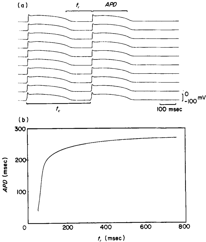
FIG. 3. (a), Response of one-dimensional cable to premature stimulation. The first action potential shown is the last one of the basic drive train. The second action potential is produced by injecting a premature stimulus into segment 1 of the strand at t_c = 400 msec. The coupling interval ( t_c ) is defined as the time from the onset of the last stimulus pulse of the basic drive train to the onset of the premature stimulus. The action potential duration ( APD ) is defined as the time from -60 mV on the upstroke to -60 mV on the repolarizing limb of the prematurely elicited action potential in segment 90 of the cable. The recovery time ( t_r ) is defined as the time from -60 mV on the repolarizing limb of the last action potential of the basic train in segment 90 to -60 mV on the upstroke of the prematurely elicited action potential. Bottom to top: segments 1, 10, 20, . . . , 80, 90. (b), Action potential duration restitution curve. APD is plotted as a function of t_r for t_c changing in steps of 1 msec in the range 292 \text{ msec} < t_c < 367 \text{ msec} , 2 msec steps for 367 \text{ msec} < t_c < 545 \text{ msec} , and 10 msec steps for 545 \text{ msec} < t_c < 1005 \text{ msec} .
