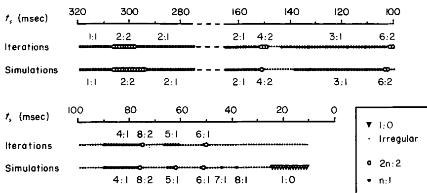
FIG. 6. Comparison between results of cable simulations and map iterations. Since 10 sec of activity in the cable was simulated, the number of iterations carried out at a given t_s was the smallest integer just larger than 10000/Nt_s , where N is the average ratio of conducted beats to stimuli in a given simulation run. For t_s < 38 msec, N = 8 . APD_i = 240 msec, which is close to the APD of the first action potential in the simulations. t_s changed in 1 msec steps. ( \nabla ), 1:0; ( \circ ), irregular; ( \bullet ), 2n:2; ( \bullet ), n:1.
