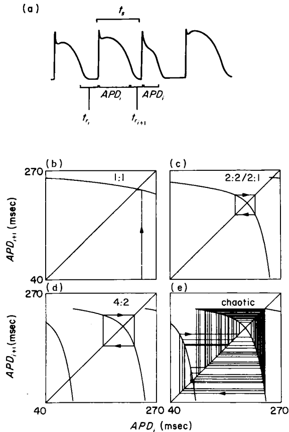
FIG. 4. (a) Schematic diagram used in deriving eqn (5), as described in text. Panels (b)–(e) show plots of the map of eqn (6) at four different values of t_s . Iterations are also shown, starting from an initial condition of APD_i = 240 msec, which is close to the APD of the first action potential in the simulations of Fig. 1. The arrows give the direction of iteration. Transients are suppressed in (c)–(e). (b), t_s = 400 msec. Iterates asymptotically converge to the stable period-1 orbit, corresponding to a 1:1 rhythm. (c), t_s = 301 msec. Iterates converge to the stable period-2 orbit shown, corresponding to a 2:2 rhythm. For some initial conditions, iterates converge to the stable period-1 orbit on the right-hand branch of the map [ n=2 in eqn (6)], corresponding to a 2:1 rhythm. Bistability is thus present (see text). (d), t_s = 150 msec. A third branch has now appeared on the map corresponding to n=3 in eqn (6). The period-1 orbit on the right-hand branch ( n=2 ) in (c) above has period-doubled, leading to a period-2 orbit on the middle branch here, corresponding to 4:2 rhythm. (e), t_s = 146 msec. Aperiodic orbit, visiting the leftmost ( n=1 ) and middle ( n=2 ) branches of the map. The rightmost ( n=3 ) branch has not yet intersected the line of identity APD_{i+1} = APD_i .
