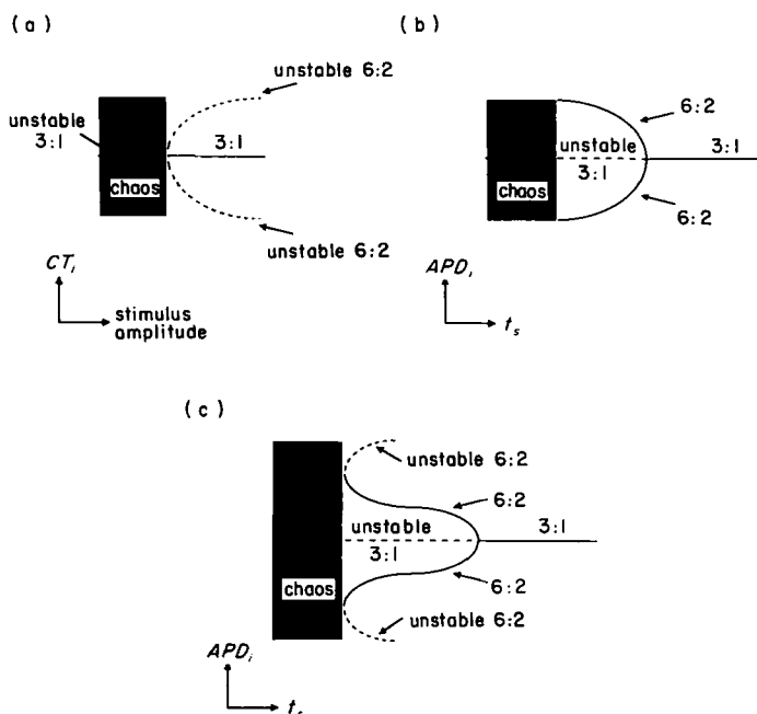
FIG. 9. Schematic bifurcation diagrams. (a), Bifurcation diagram illustrating type III intermittency of Matsumoto et al. (1987b) in squid giant axon. CT_i is the conduction time of the i th action potential to propagate down the axon. (b), Bifurcation diagram illustrating transition from 3:1 rhythm to chaos in Figs 5(a) and (6), Bifurcation diagram obtained from that in (b) by modifying APD restitution curve. Solid lines indicate stable orbits, dashed lines unstable orbits. Saddle-node bifurcation occurs at turning point in (c). See text for further description.
