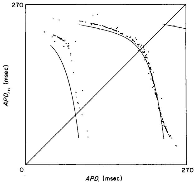
FIG. 7. The return map. Symbols give return map ( APD_{i+1} vs. APD_i ) obtained from numerical simulation of the cable equation at t_s = 143 msec [see Fig. 1(e)] for 60 sec. Superimposed is the three-branched map [see Fig. 4(e)], eqn (6), derived from the response to premature stimulation, at the same t_s .
