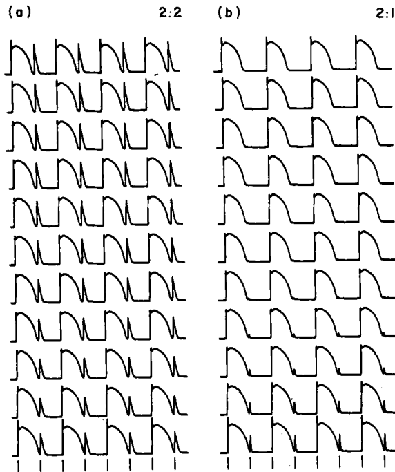
FIG. 2. Bistability in the response of the cable to periodic stimulation. t_s = 295 msec. (a), 2:2 rhythm, obtained starting numerical integration from standard initial conditions (given in Methods). (b), 2:1 rhythm, obtained starting numerical integration from asymptotic rest initial conditions. Traces taken from near end of a 10-sec simulation run in order to allow transients to dissipate. APD of first action potential at start of simulation run from which (b) is taken was 22 msec greater than in (a). APD in segment 90 in the steady-state: 250 and 43 msec (a), 254 msec (b).
