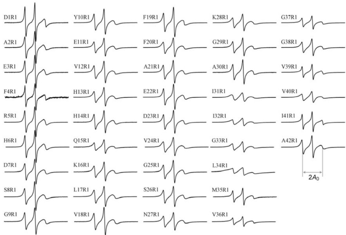
Figure 2. EPR spectra of spin-labeled A \beta 42 globulomers.
