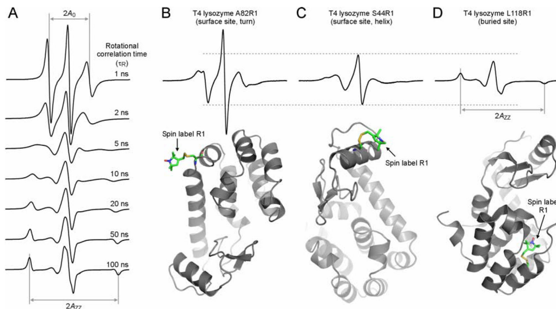
Figure 1. Effect of spin label mobility and labeling location on EPR spectral lineshape.
